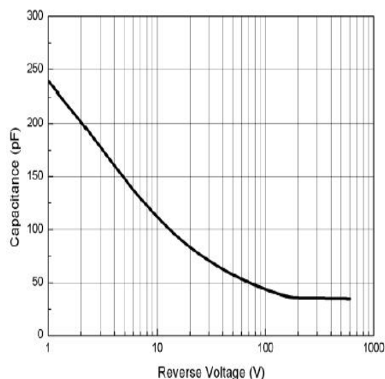
Fig.4-Typical Junction Capacitance
