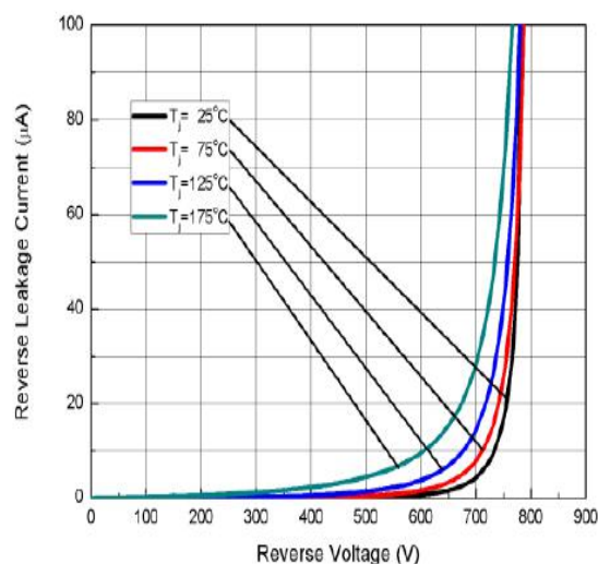
Fig.2-Typical Reverse Characteristics
