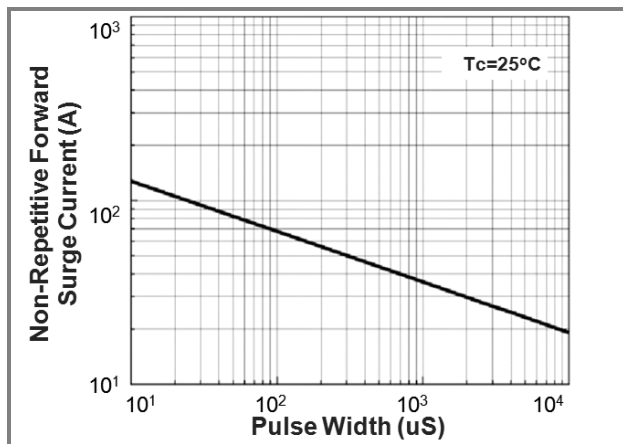
Fig.4 Non-Repetitive Peak Forward Surge Current (Pulse Mode)
