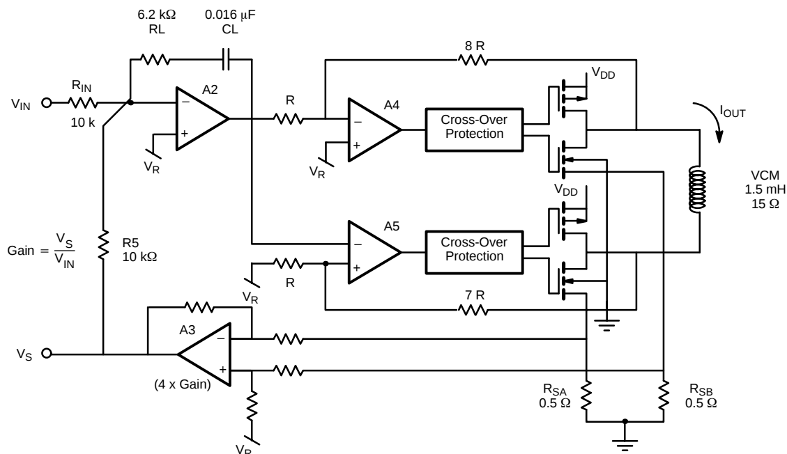
FIGURE 3. Transconductance Amplifier
