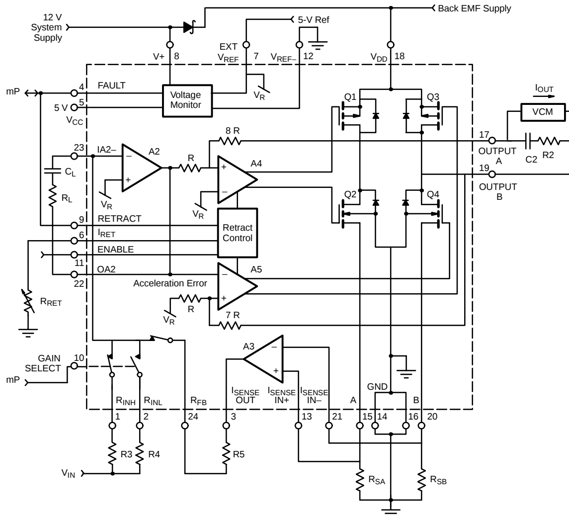
FIGURE 1. Si9961 Typical Application
