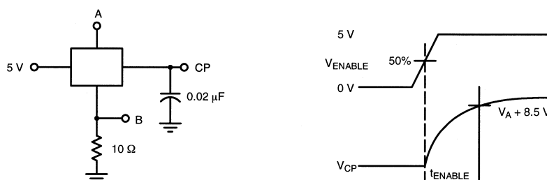
FIGURE 2. Test Circuit 2
