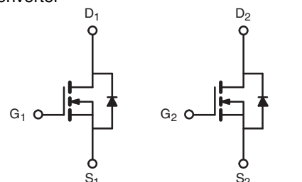
N-Channel MOSFET
