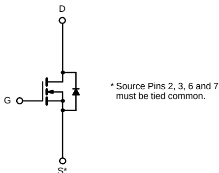
N-Channel MOSFET
