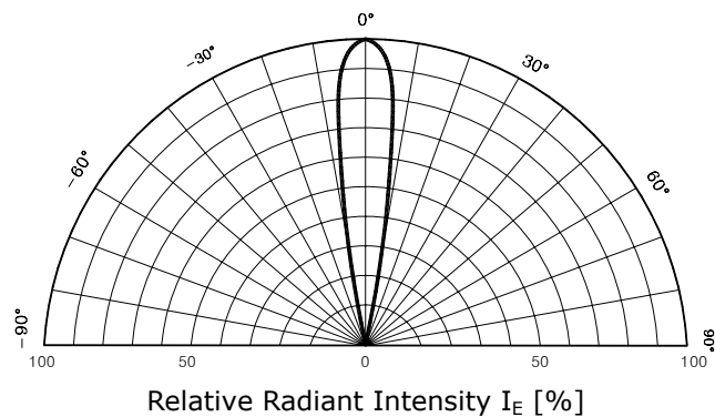
Fig. 5 Radiation Diagram
