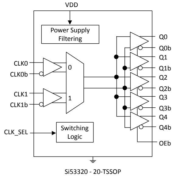
Figure 4.1. Si533320 Block Diagram
