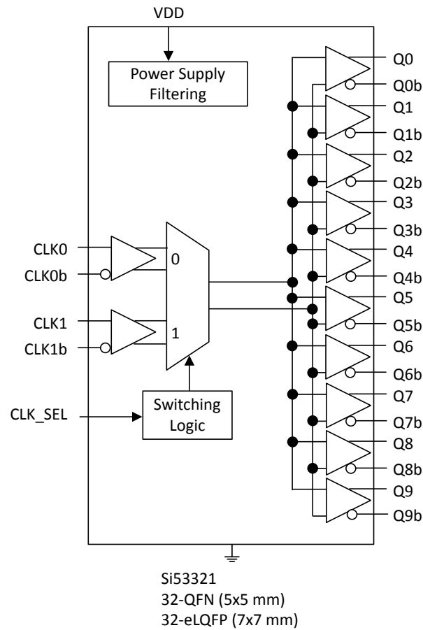
Figure 4.2. Si533321 Block Diagram
