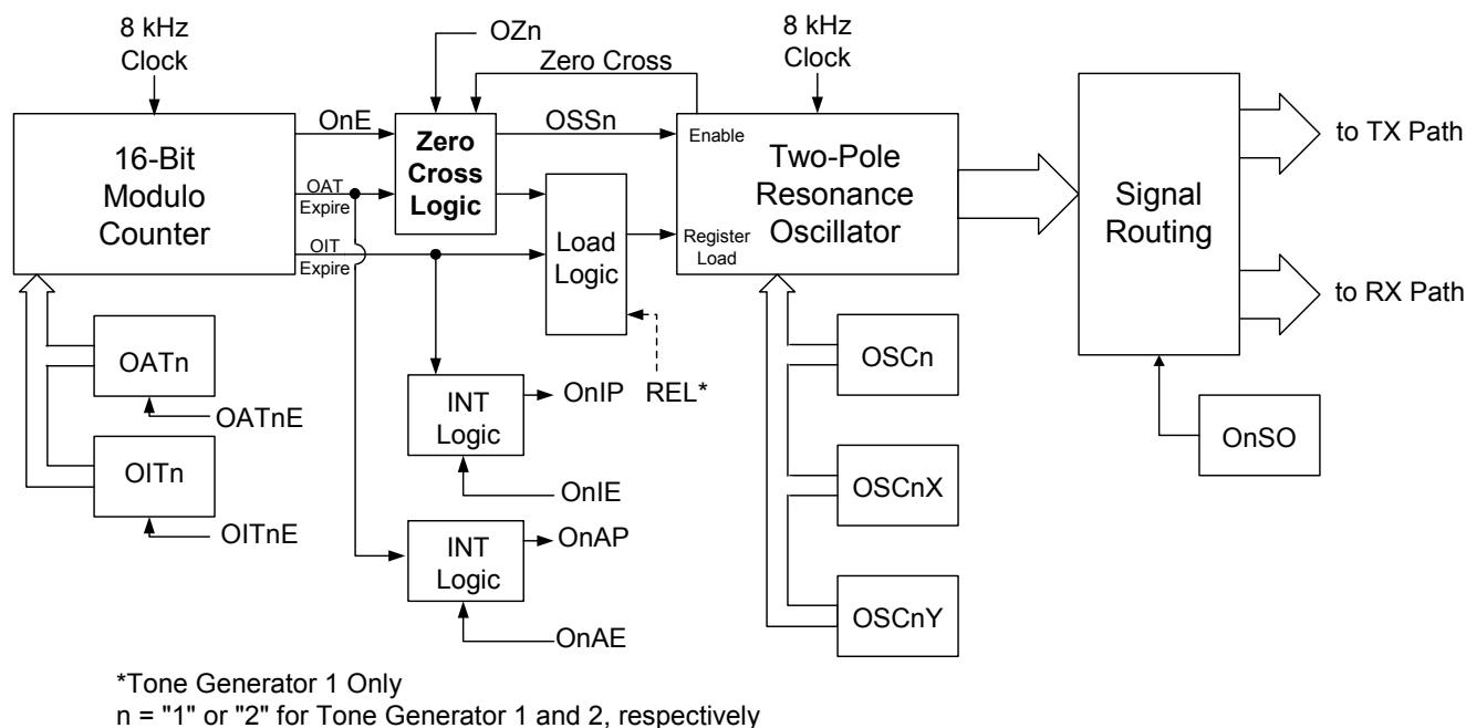
Figure 11. Simplified Tone Generator Diagram
