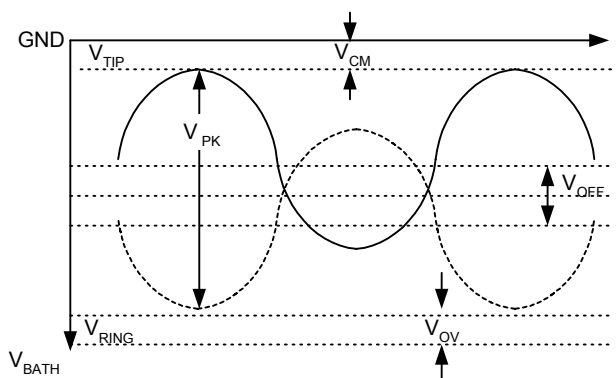
Figure 23. Balanced Ringing
