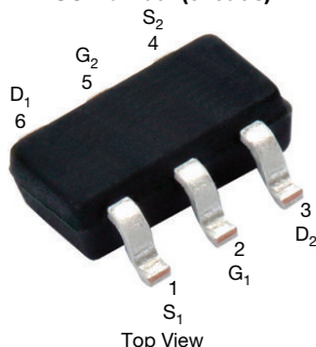
SOT-363 SC-70 Dual (6 leads)
