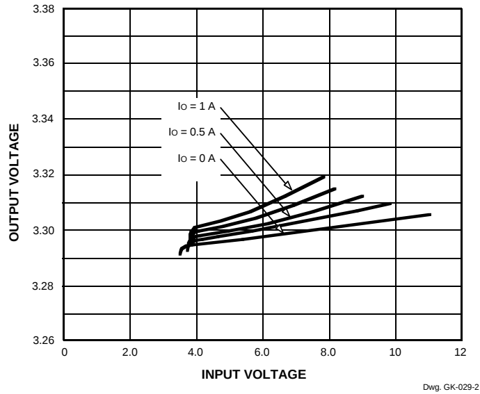
Line regulation
