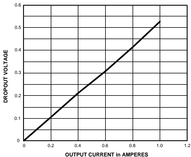
Dropout voltage
