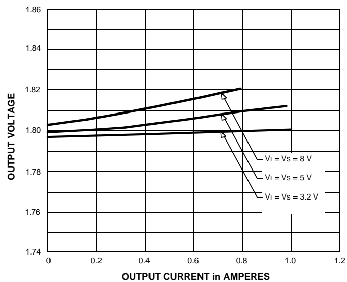
Load regulation
