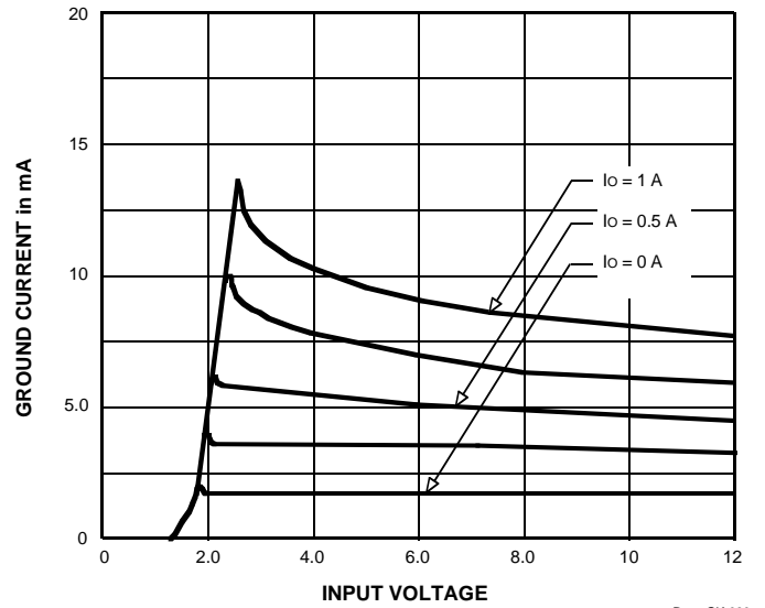
GND current
