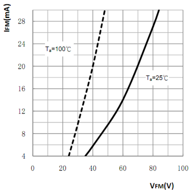
Forward Characteristics
