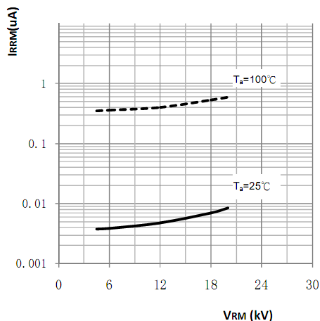
Reverse Characteristics
