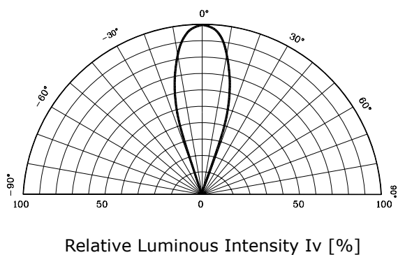
Fig. 5-1 Radiation Diagram(X)
