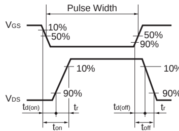
Fig.18 Switching Waveforms
