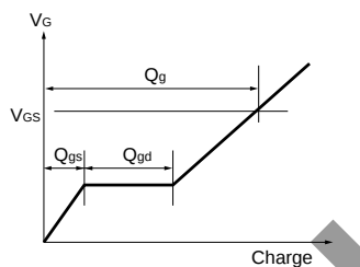
Fig.2-2 Gate Charge Waveform
