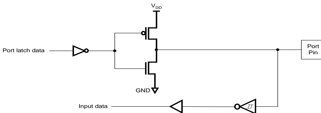
Push-Pull Mode
