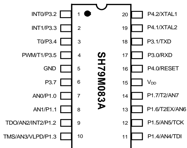
Pin Configuration Diagram
