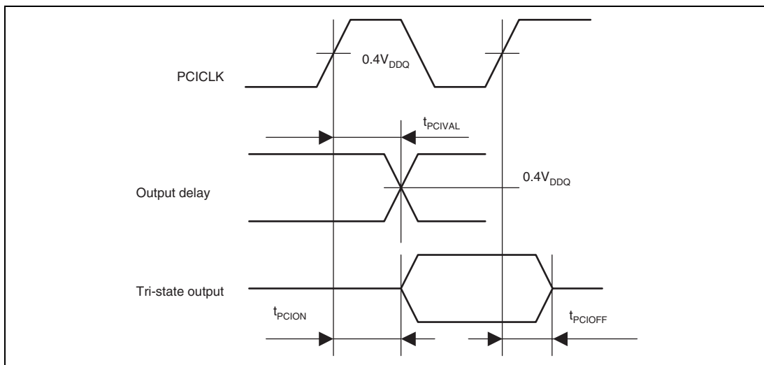
Figure 32.38 PCI Output Signal Timing
