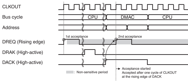
Figure 14.15 Example 3 of DREQ Input Detection in Cycle Steal Mode Edge Detection (Word Transfer in 8-Bit Bus Width, Longword Transfer in 8/16-Bit Bus Width, or 16/32-Byte Transfer in 8/16/32/64-Bit Bus Width: DACK of DMA1 Transfer Is Connected)
