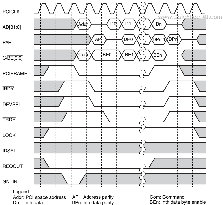
Figure 13.22 Master Read Cycle in Normal Mode (Burst)
