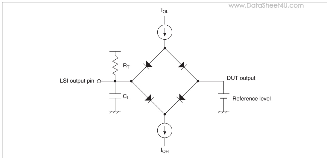
Figure 32.76 Output Load Circuit
