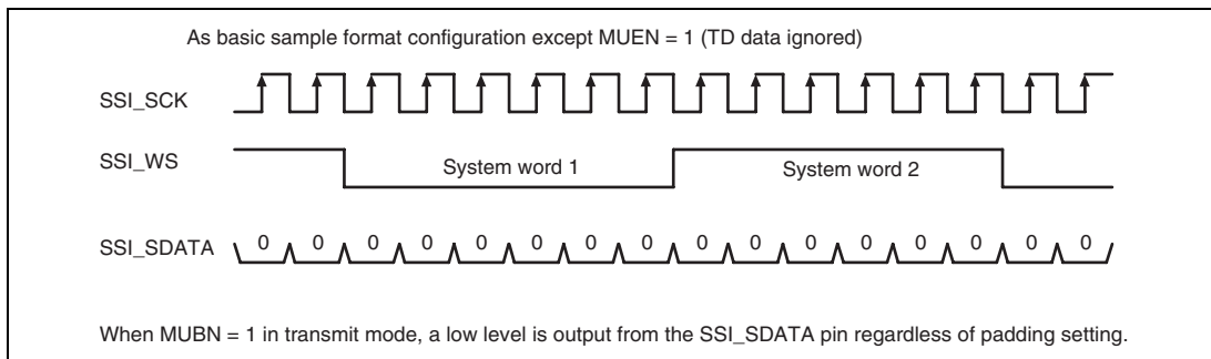
Figure 26.17 Mute Enabled
