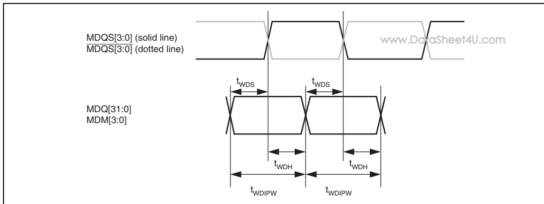
Figure 32.32 MDQS and MDQ/MDM Output Waveform (Write)
