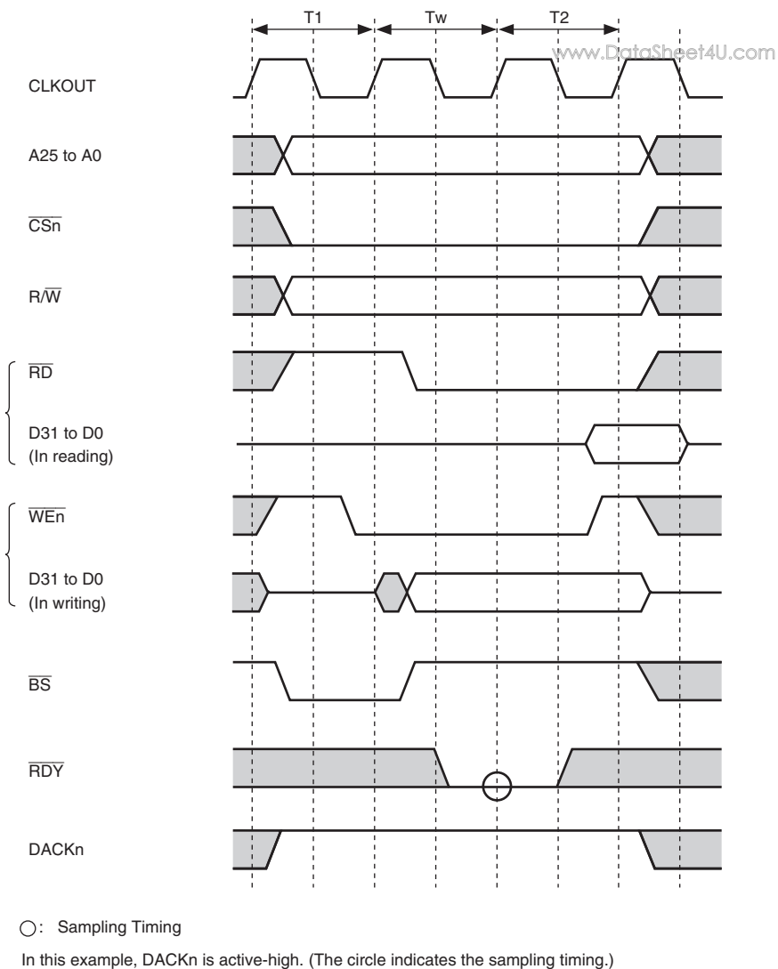
Figure 11.9 SRAM Interface Wait Timing (Software Wait Only)
