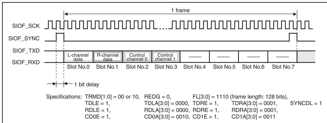
Figure 22.18 Transmit and Receive Timing (16-Bit Stereo Data (3))
