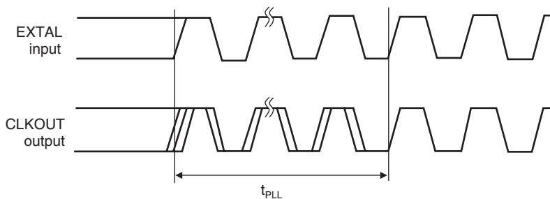
Figure 32.5 PLL Synchronization Settling Time
