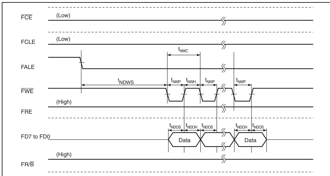
Figure 32.70 Data Write Timing of NAND-Type Flash Memory
