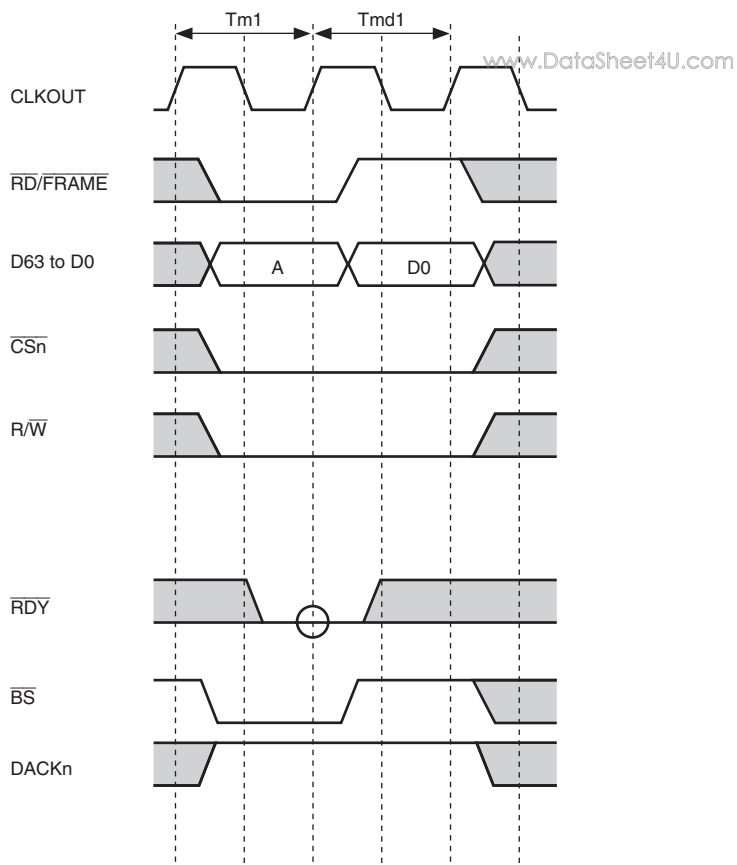
Figure 11.26 MPX Interface Timing 3 (Single Write Cycle, IW = 0000, No External Wait, 64-Bit Bus Width)
