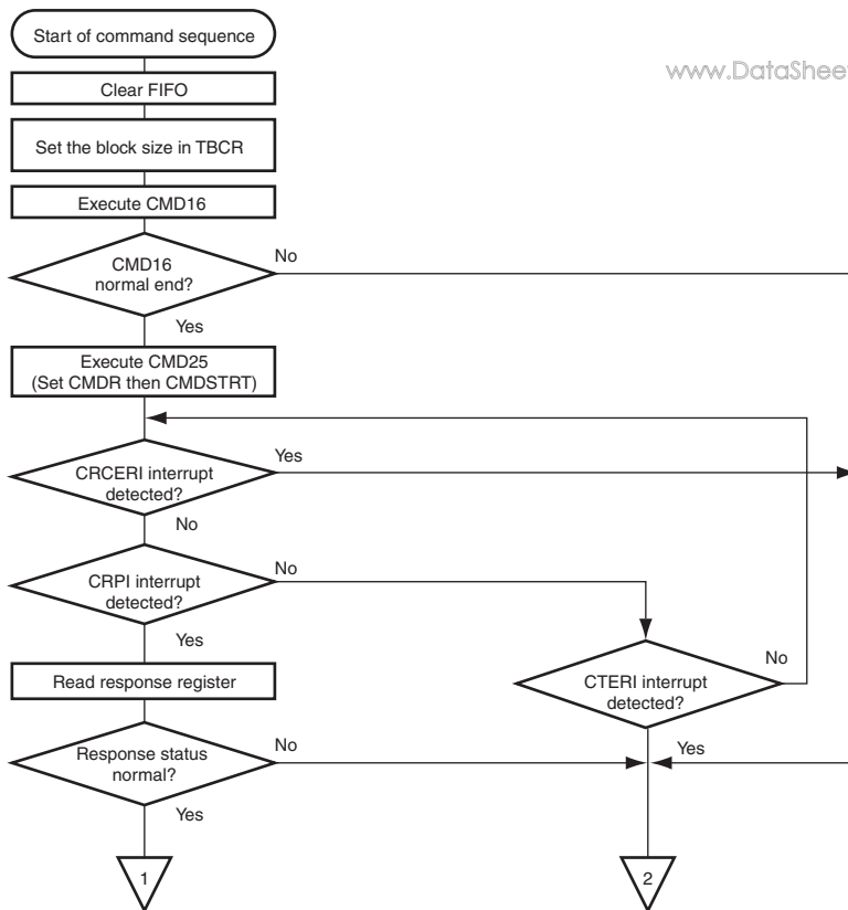
Figure 24.20 (1) Example of Operational Flow for Commands with Write Data (Open-ended Multiple Block Transfer)
