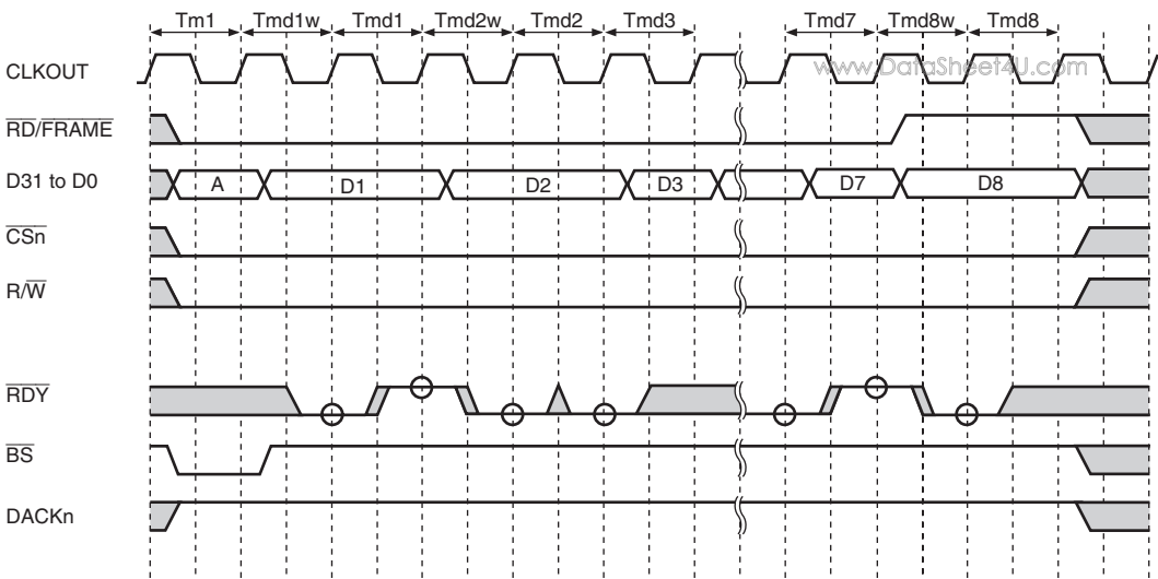
Figure 11.35 MPX Interface Timing 12 (Burst Write Cycle, IW = 0001, External Wait Control, 32-Bit Bus Width, 32-Byte Data Transfer)
