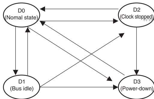
Figure 13.18 Power Down State Transitions on PCI Bus
