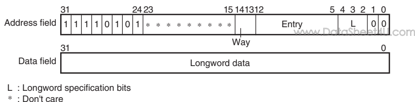
Figure 8.8 Memory-Mapped OC Data Array (Cache size = 32 Kbytes)
