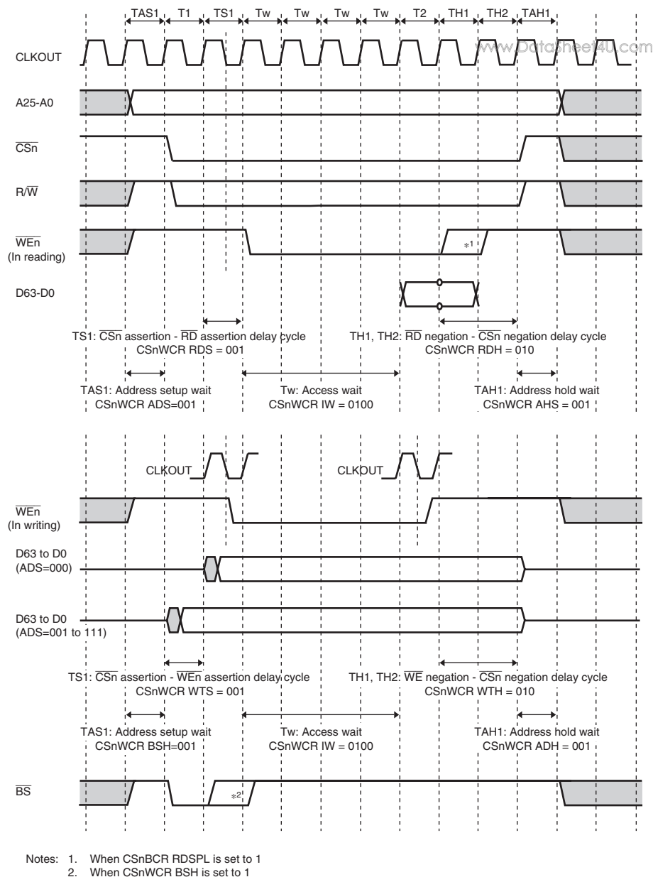
Figure 11.39 Wait State Timing of Byte Control SRAM
