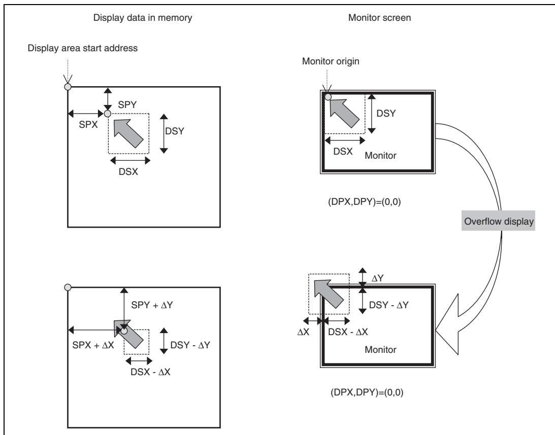
Figure 19.11 Schematic Diagram of Upper-Left Overflow Display
