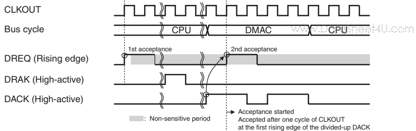
Figure 14.14 Example 2 of DREQ Input Detection in Cycle Steal Mode Edge Detection (Word Transfer in 8-Bit Bus Width, Longword Transfer in 8/16-Bit Bus Width, 16/32-Byte Transfer in 8/16/32/64-Bit Bus Width: DACK of DMA1 Transfer Divided)
