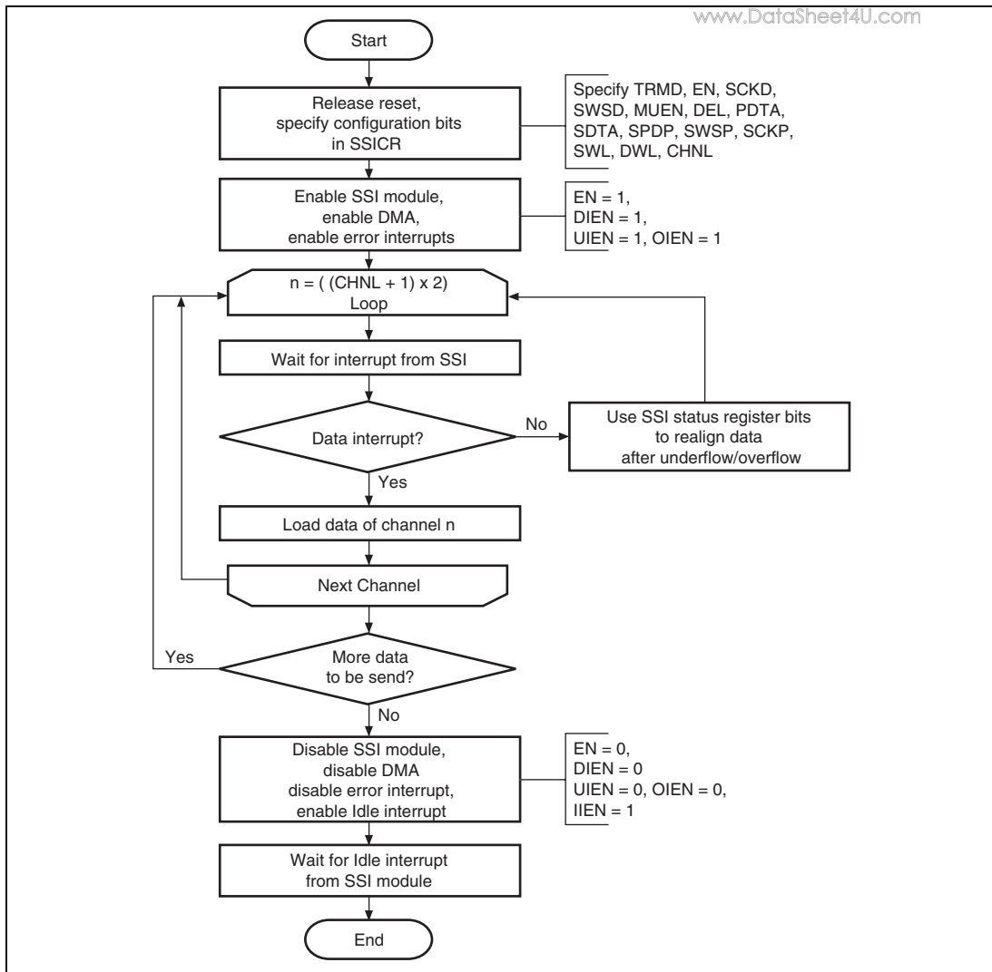
Figure 26.22 Transmission Using Interrupt Data Flow Control
