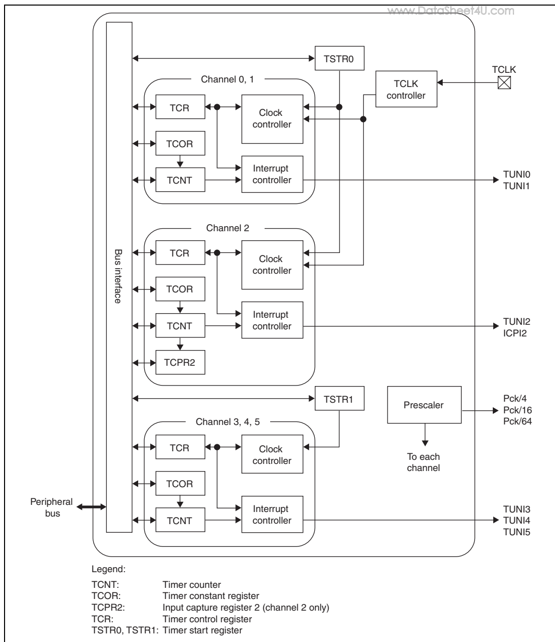
Figure 18.1 Block Diagram of TMU
