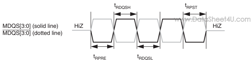
Figure 32.29 Restriction of MDQS Input Waveform (Read)
