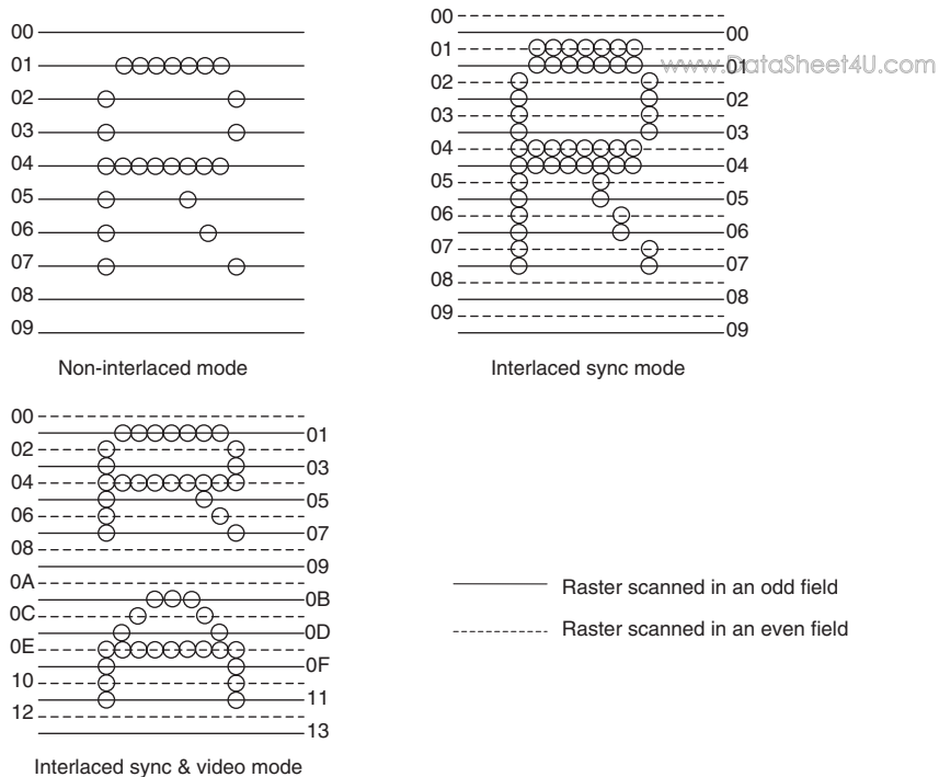
Figure 19.16 Example of Display in Each Scan Mode
