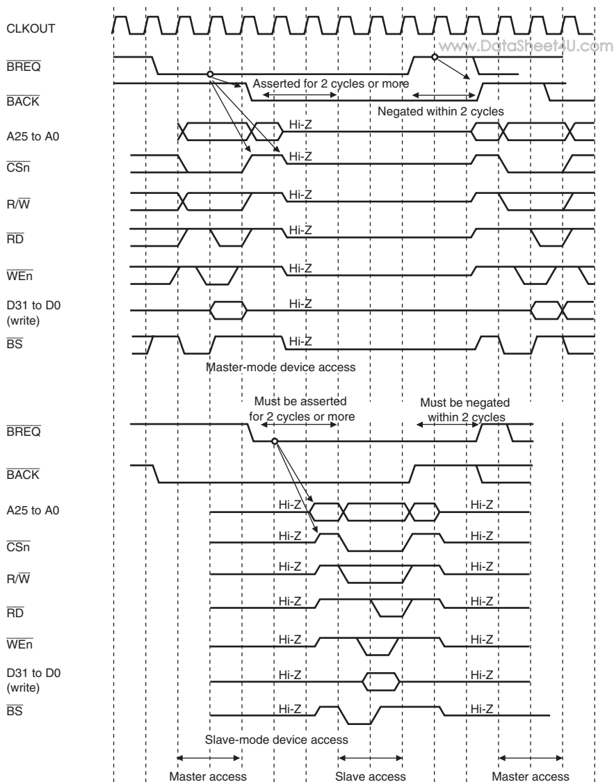
Figure 11.42 Arbitration Sequence
