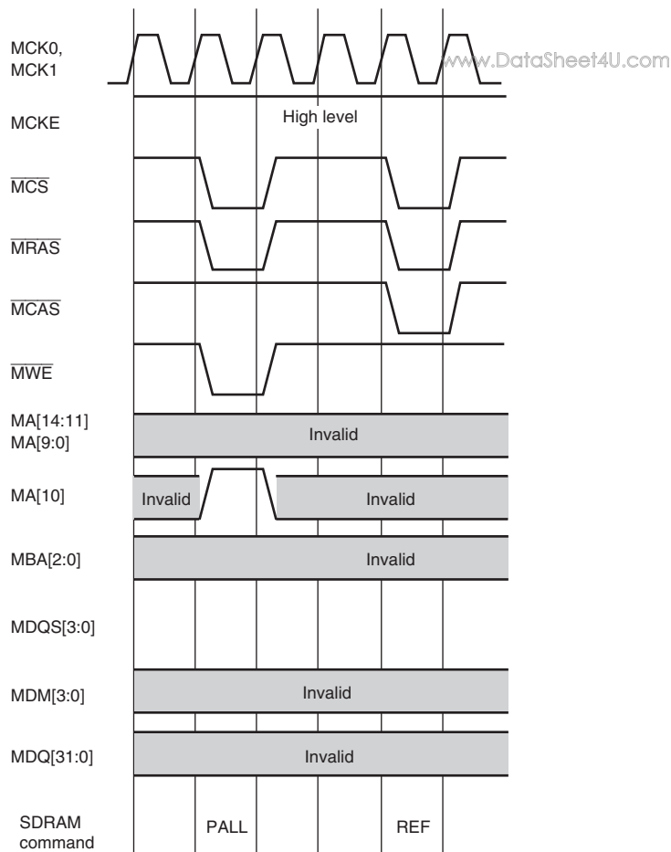
Figure 12.12 Auto-Refresh Operation
