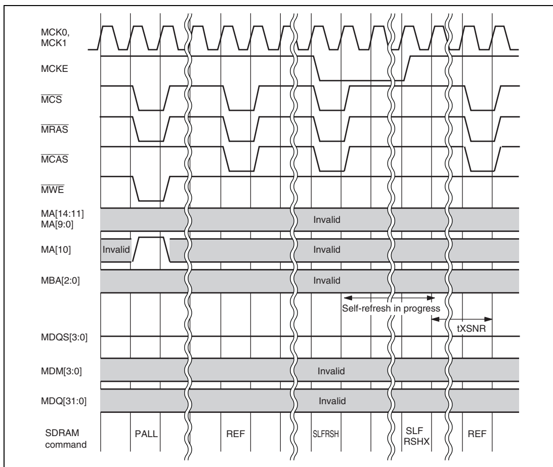
Figure 12.13 Self-Refresh Operation
