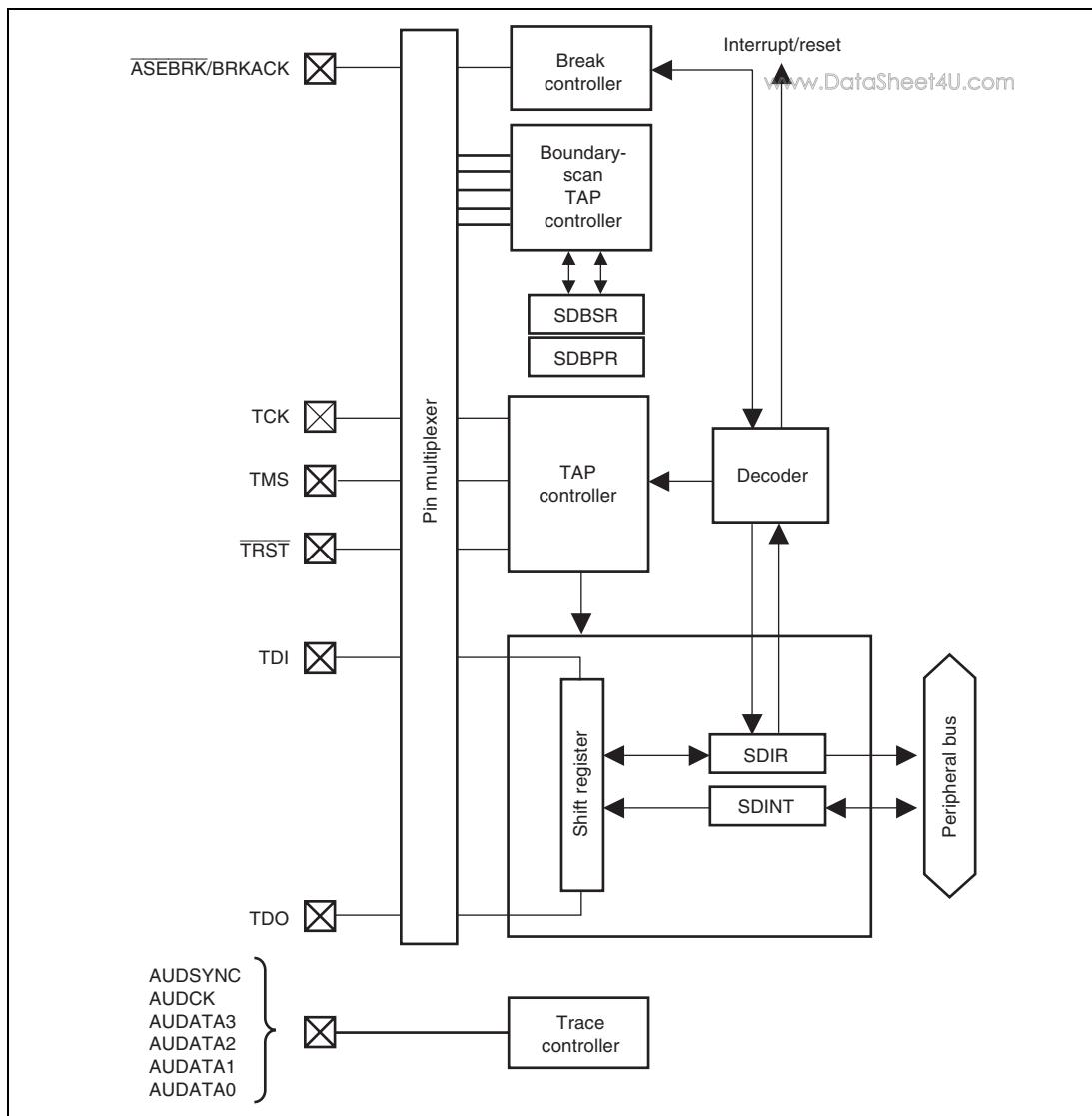
Figure 30.1 Block Diagram of H-UDI
