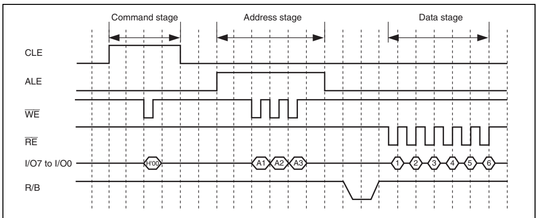
Figure 27.2 Reading Operation Timing for NAND-Type Flash Memory
