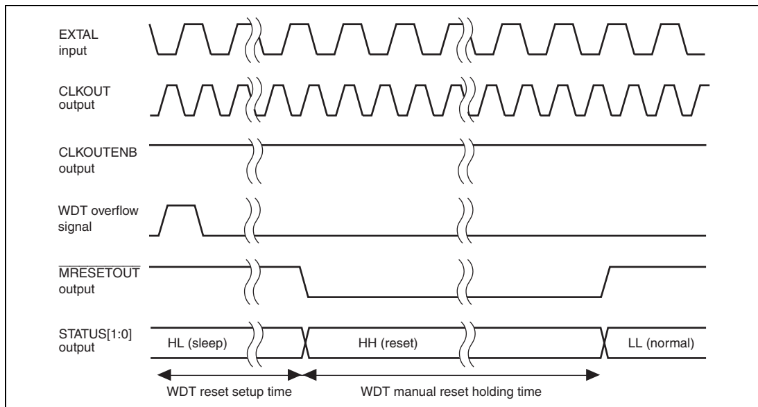
Figure 16.9 STATUS Output by Manual Reset Caused by WDT Overflow in Sleep Mode
