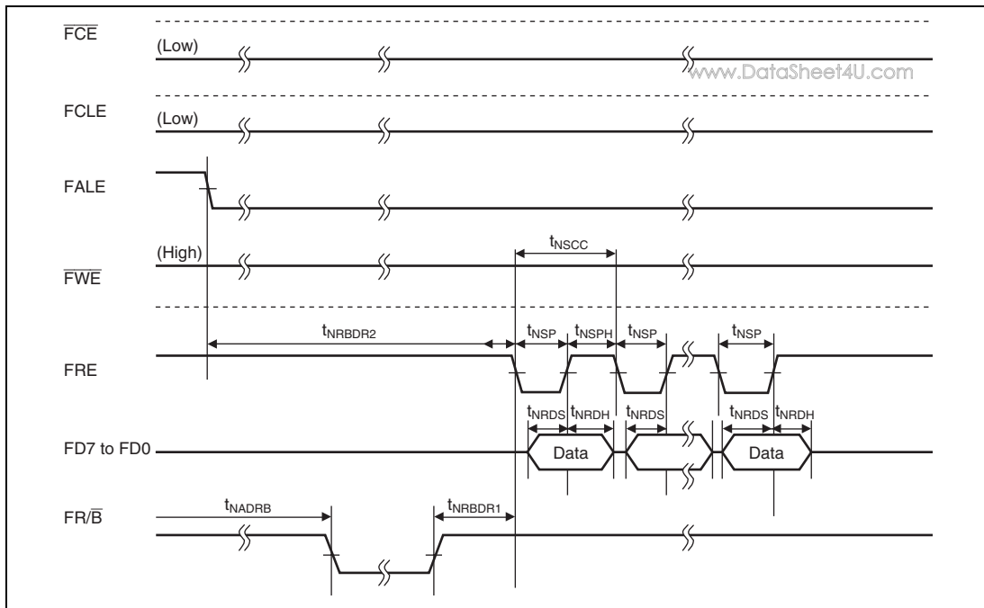
Figure 32.69 Data Read Timing of NAND-Type Flash Memory
