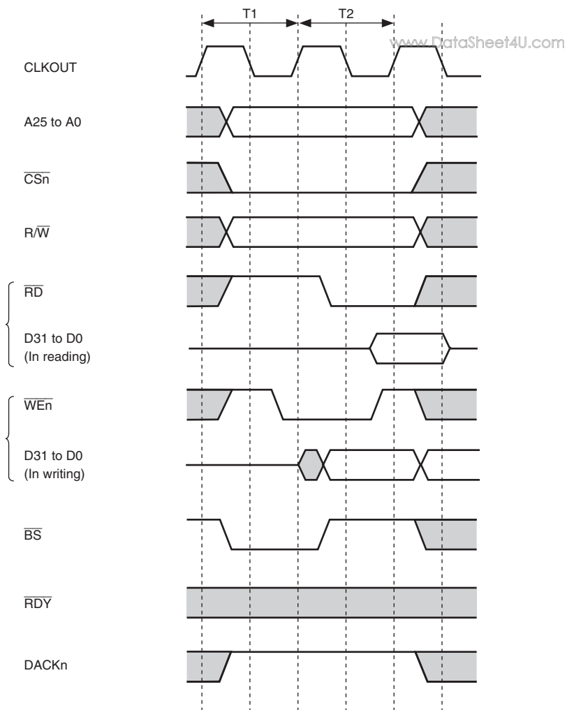
Figure 11.5 Basic Timing of SRAM Interface
