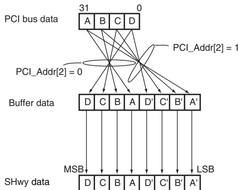
Figure 13.14 Endian Conversion from PCI Bus to SuperHyway Bus (Byte Swapping: TBS = 1)
