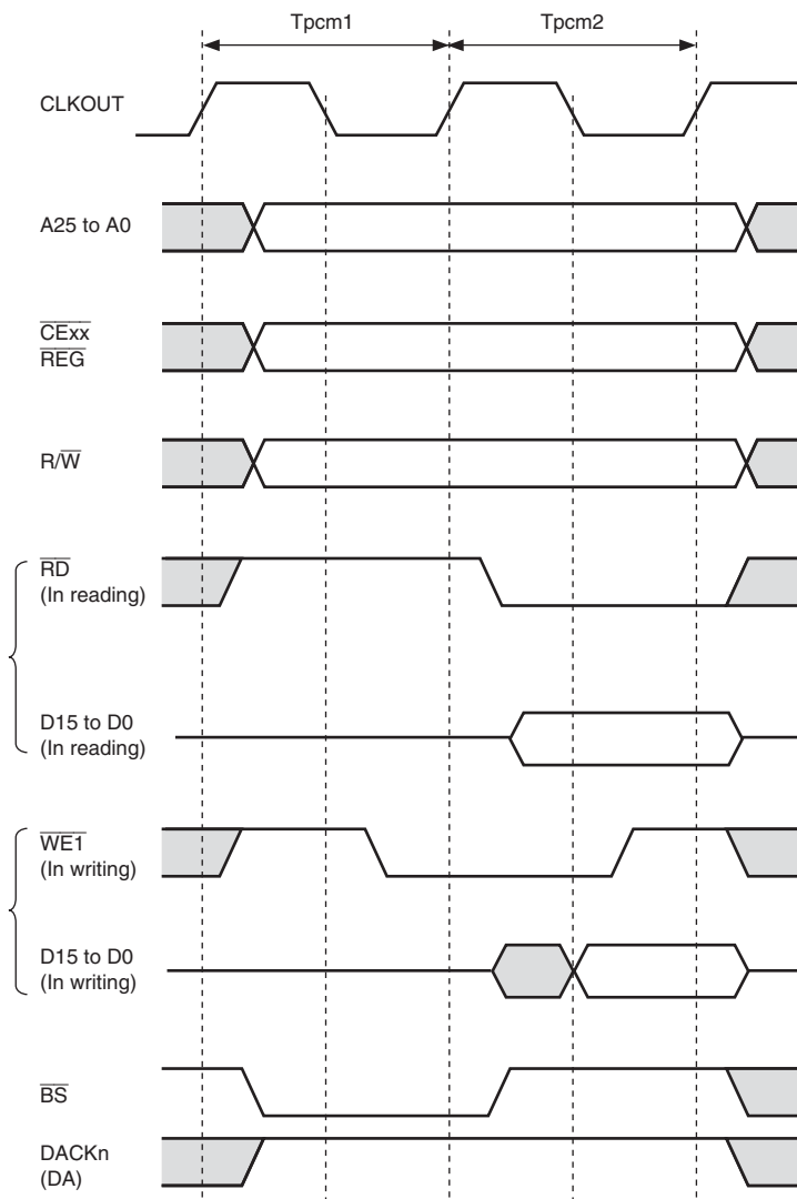
Figure 11.17 Basic Timing for PCMCIA Memory Card Interface
