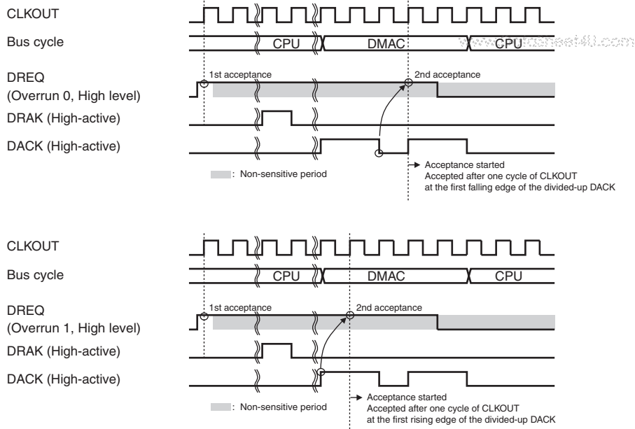
Figure 14.17 Example 2 of DREQ Input Detection in Cycle Steal Mode Level Detection (Word Transfer in 8-Bit Bus Width, Longword Transfer in 8/16-Bit Bus Width, 16/32-Byte Transfer in 8/16/32/64-Bit Bus Width: DACK of DMA1 Transfer Divided)
