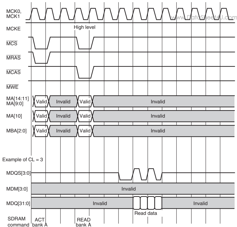
Figure 12.8 Waveforms for 1/2/4/8/16-Byte Reading (When the Bus Width Is Set to 32 Bits)
