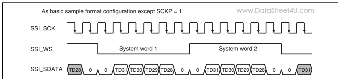
Figure 26.10 Inverted Clock
