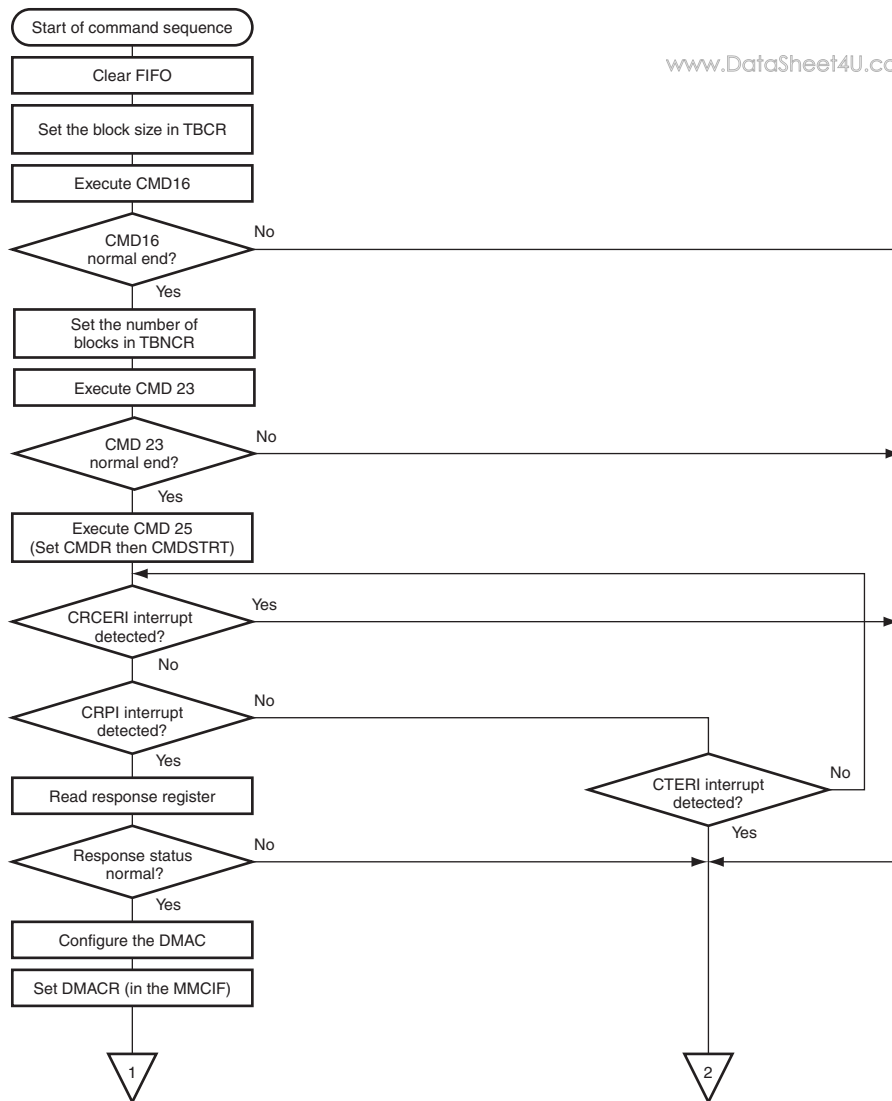
Figure 24.27 (3) Example of Write Sequence Flow (Pre-defined Multiple Block Transfer)
