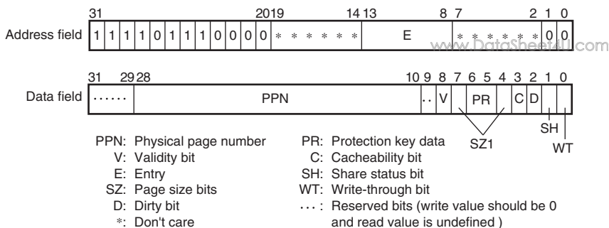
Figure 7.23 Memory-Mapped UTLB Data Array (TLB Compatible Mode)
