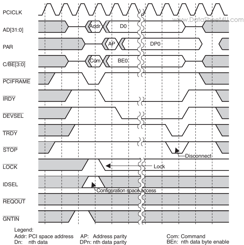
Figure 13.24 Target Write Cycle in Normal Mode (Single)
