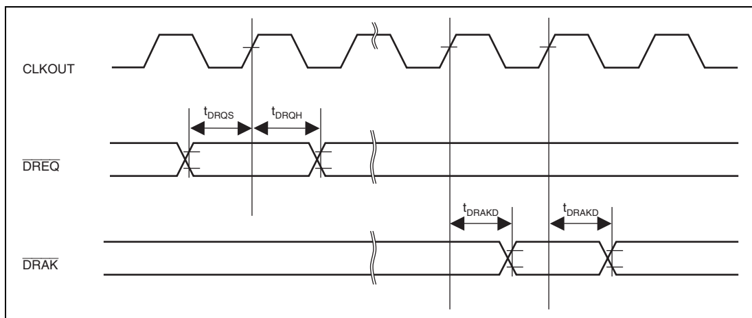
Figure 32.40 \overline{\text{DREQ}}/\overline{\text{DRAK}} Signal Timing
