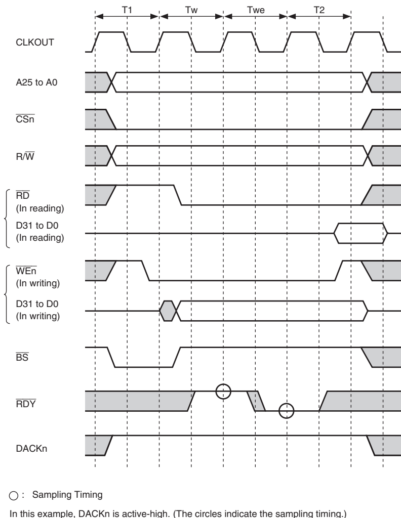
Figure 11.10 SRAM Interface Wait Timing (Wait Cycle Insertion by \overline{\text{RDY}} Signal, \overline{\text{RDY}} Signal Is Synchronous Input)
