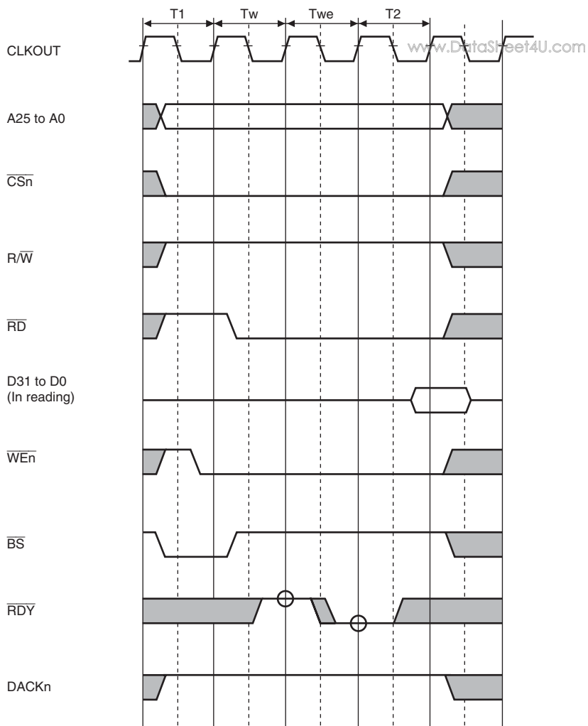
Figure 11.40 Wait State Timing of Byte Control SRAM (One Internal Wait + One External Wait)
