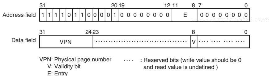
Figure 7.28 Memory-Mapped PMB Address Array
