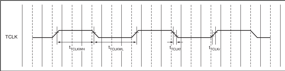
Figure 32.41 TCLK Input Timing
