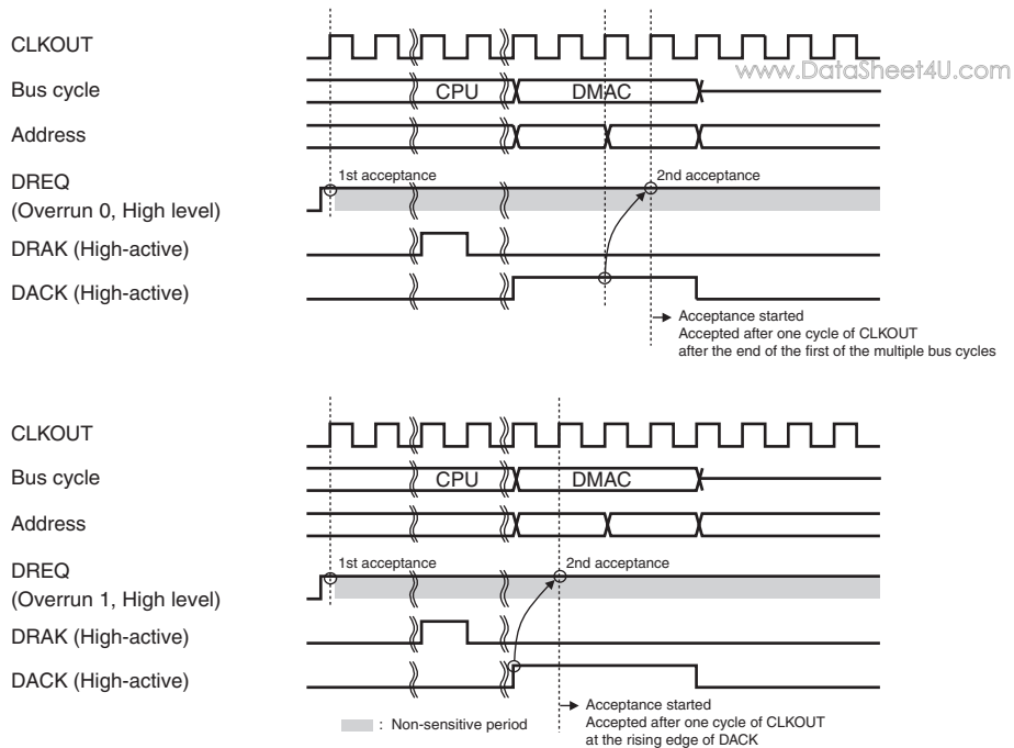
Figure 14.22 Example 3 of DREQ Input Detection in Burst Mode Level Detection (Word Transfer in 8-Bit Bus Width, Longword Transfer in 8/16-Bit Bus Width, or 16/32-Byte Transfer in 8/16/32/64-Bit Bus Width: DACK of DMA1 Transfer Is Connected)
