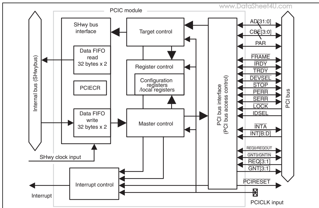
Figure 13.1 Block Diagram of PCIC
