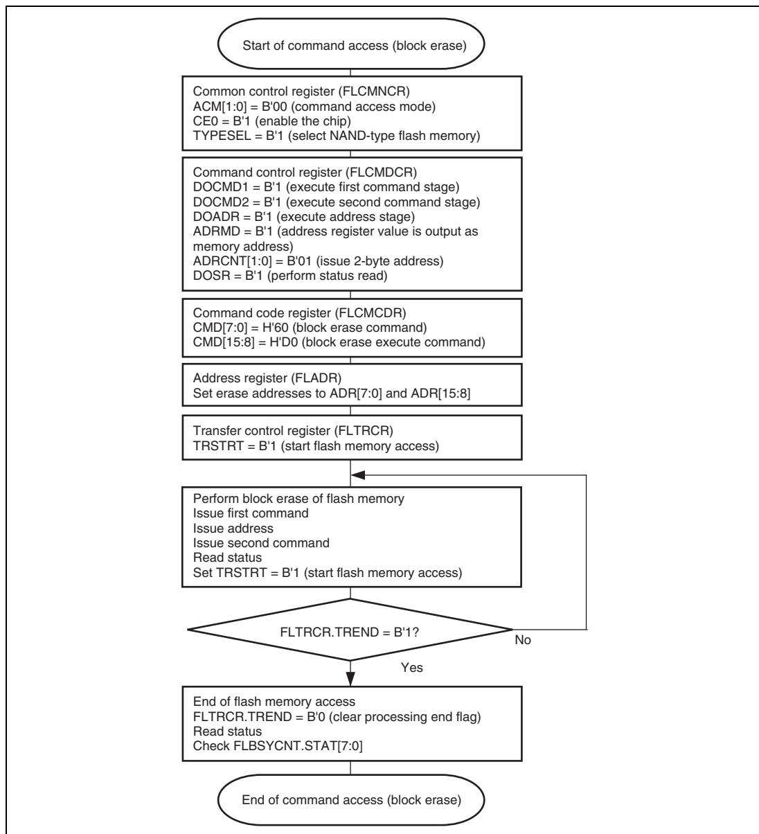
Figure 27.11 NAND Command Access (Block Erase)
