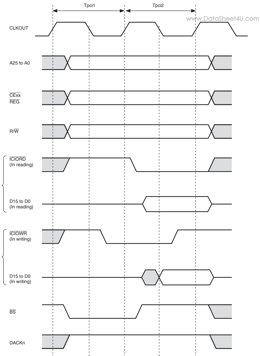
Figure 11.19 Basic Timing for PCMCIA I/O Card Interface
