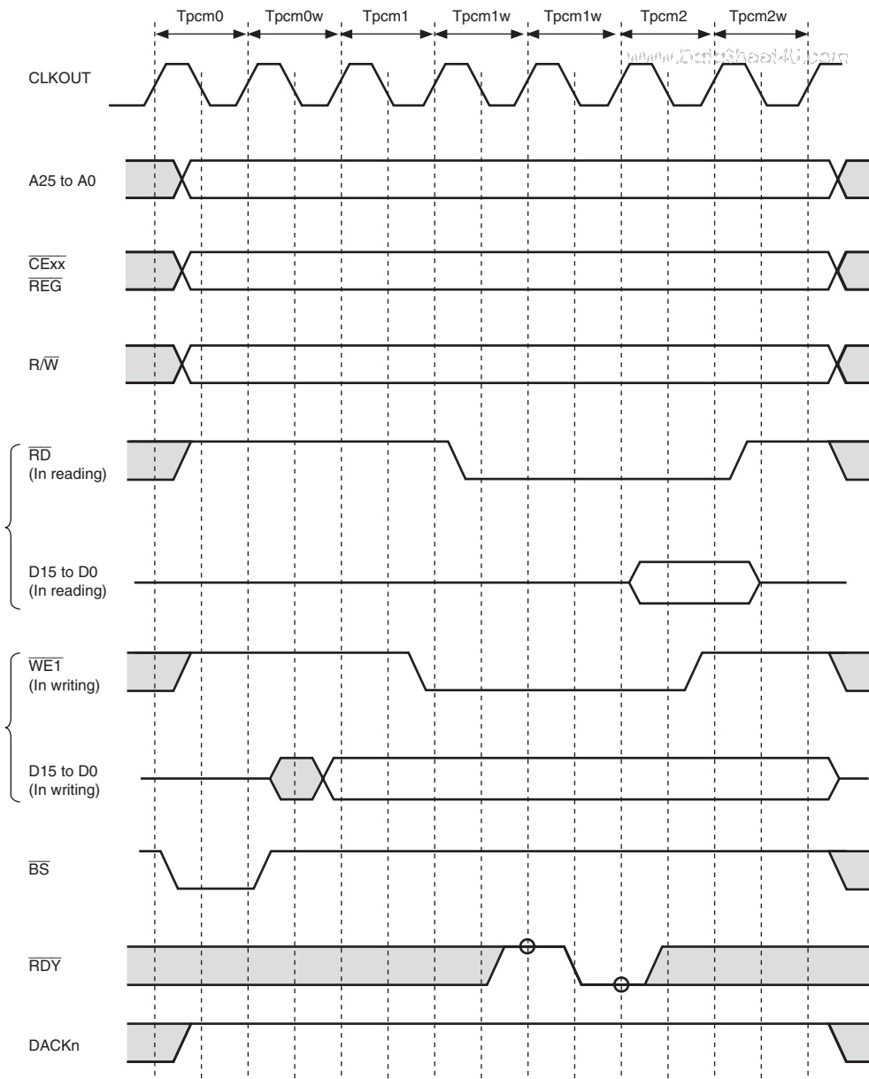
Figure 11.18 Wait Timing for PCMCIA Memory Card Interface
