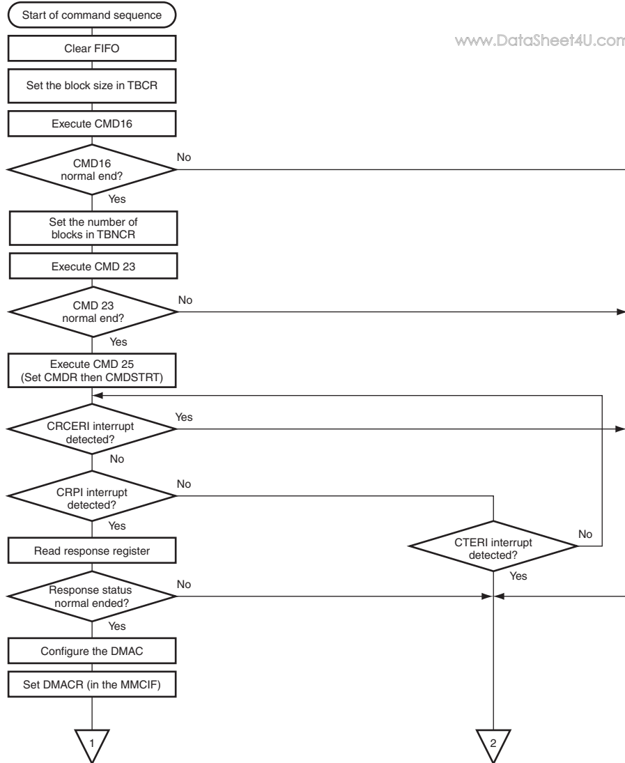
Figure 24.29 (1) Example of Operational Flow for Auto-mode Pre-defined Multiple Block Write Transfer
