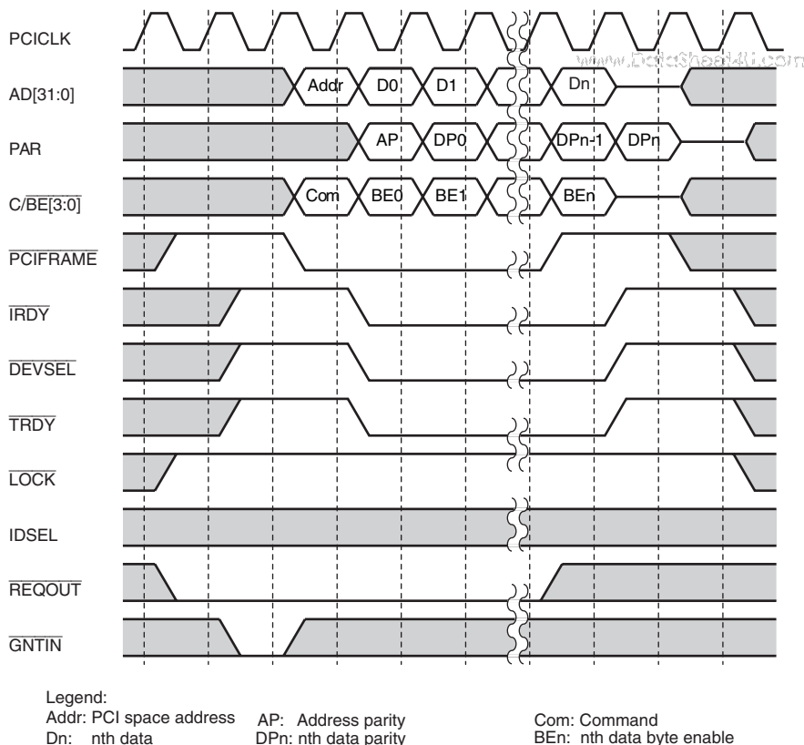
Figure 13.21 Master Write Cycle in Normal Mode (Burst)
