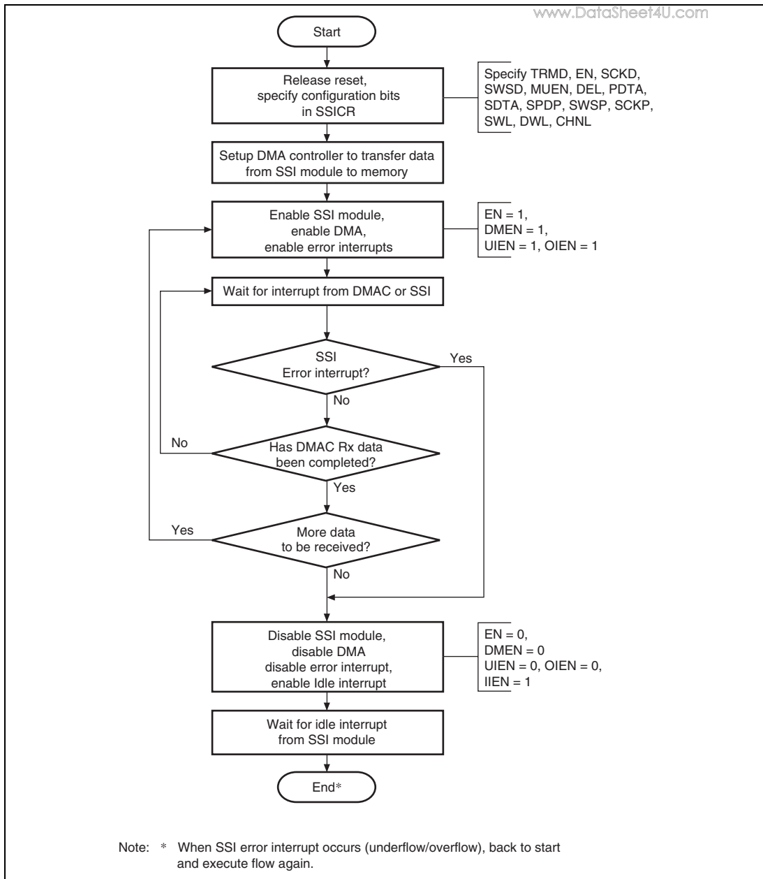
Figure 26.23 Reception Using DMA Controller
