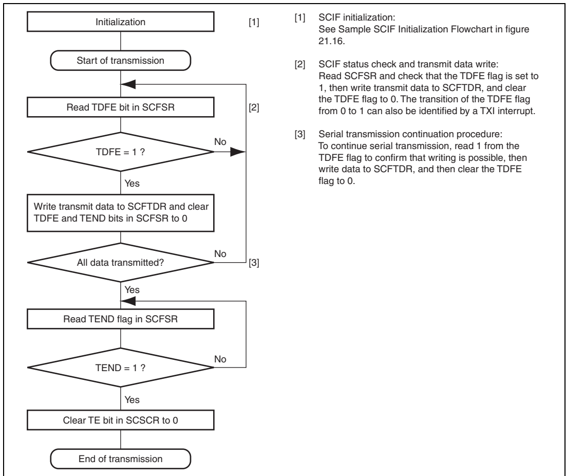
Figure 21.17 Sample Serial Transmission Flowchart
