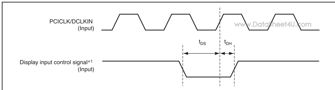
Figure 32.73 Display Timing (with Respect to PCICLK/DCLKIN)
