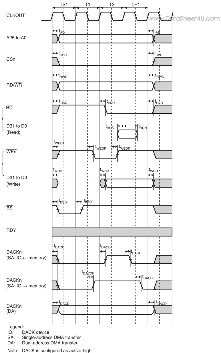
Figure 32.12 SRAM Bus Cycle: Basic Bus Cycle (CSnWCR.IW = 0000, CSnWCR.RDS = 001, CSnWCR.WTS = 001, CSnWCR.RDH = 001, CSnWCR.WTH = 001)
