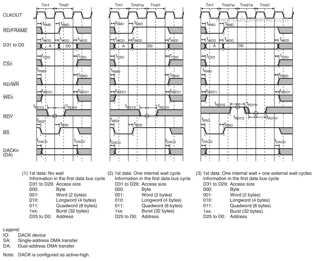
Figure 32.21 MPX Basic Bus Cycle (Write)
