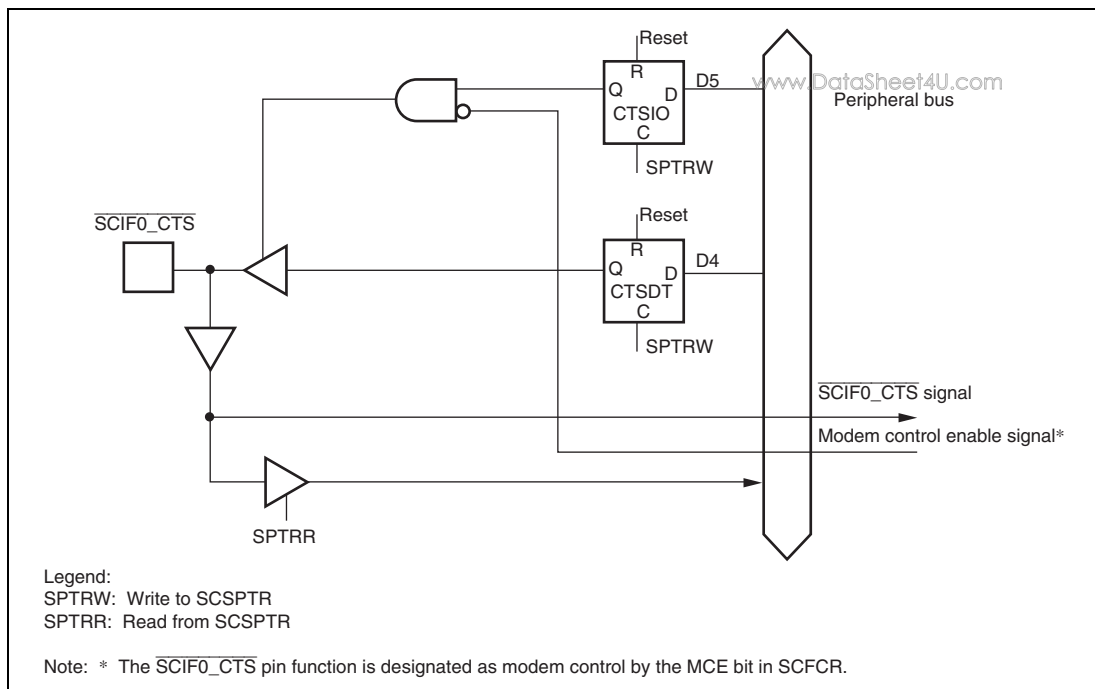
Figure 21.3 SCIF0_CTS Pin
