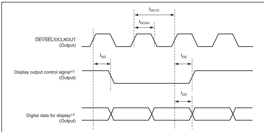
Figure 32.74 Display Timing (with Respect to DEVSEL/DCLKOUT)
