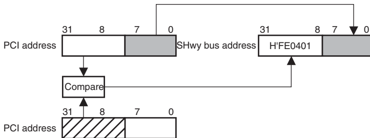
Figure 13.12 I/O Access from PCI Bus to SuperHyway Bus
