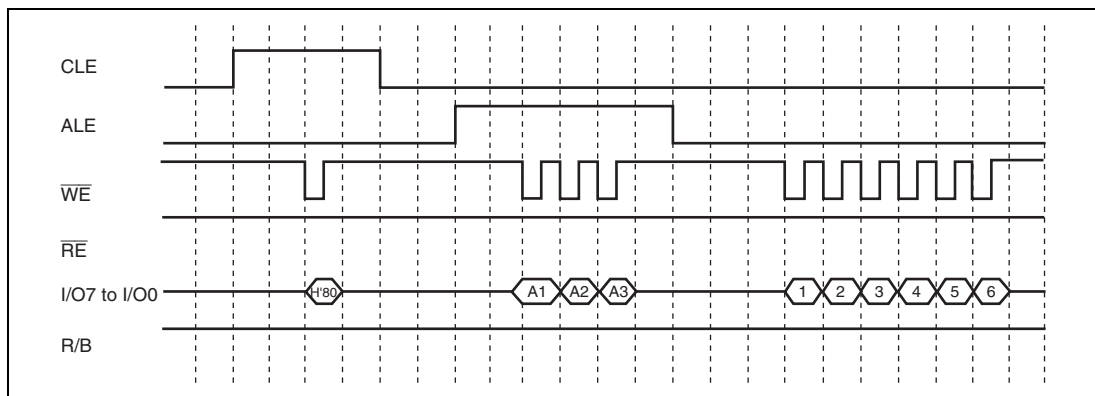
Figure 27.3 Writing Operation Timing for NAND-Type Flash Memory
