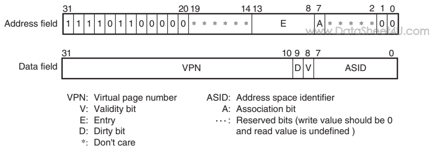
Figure 7.22 Memory-Mapped UTLB Address Array
