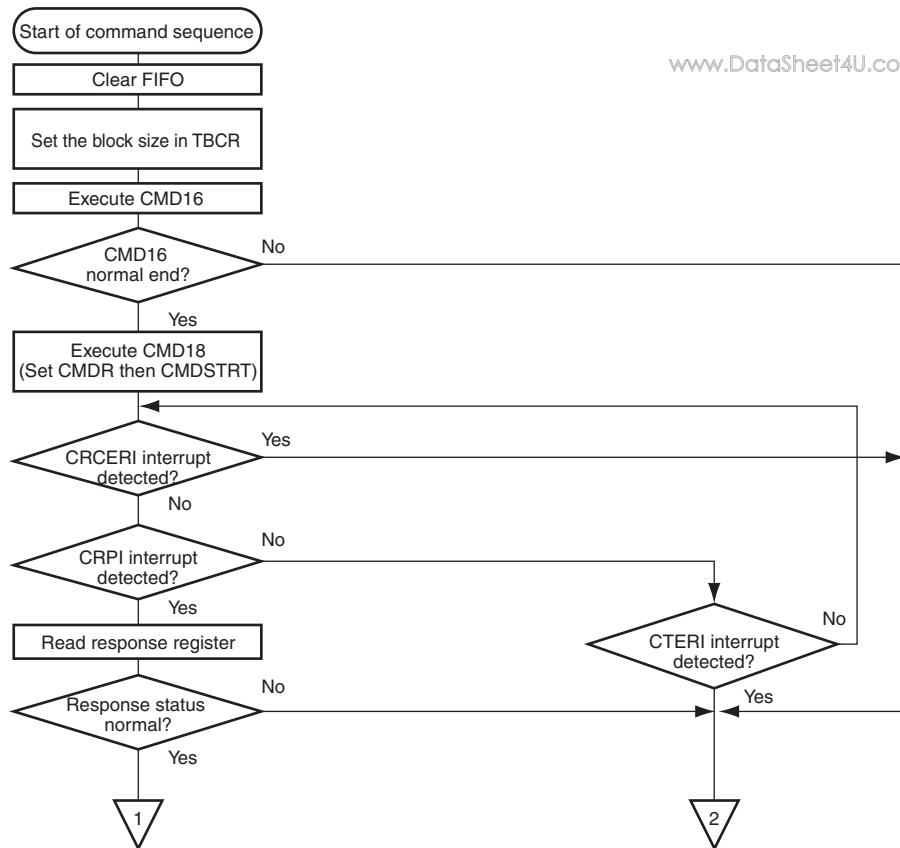
Figure 24.13 Example of Operational Flow for Commands with Read Data (1) (Open-ended Multiple Block Transfer)
