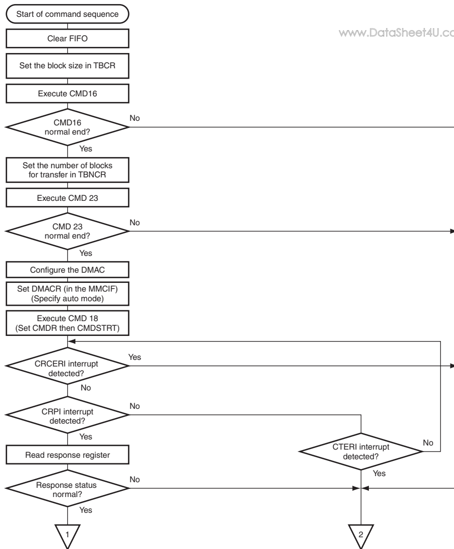
Figure 24.25 (1) Example of Operational Flow for Auto-mode Pre-defined Multiple Block Read Transfer
