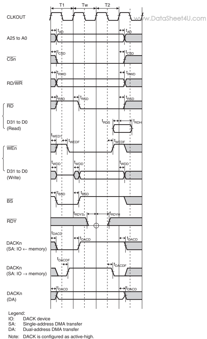
Figure 32.10 SRAM Bus Cycle: Basic Bus Cycle (One Internal Wait Cycle)
