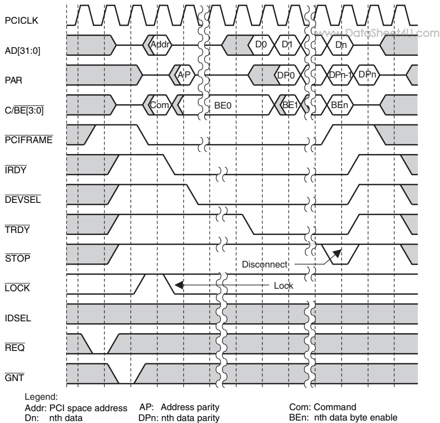
Figure 13.25 Target Memory Read Cycle in Host Mode (Burst)
