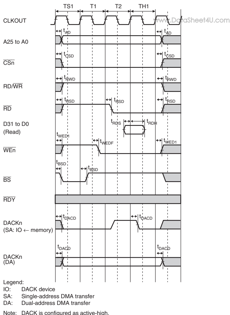
Figure 32.25 Memory Byte Control SRAM Bus Cycle: Basic Read Cycle (CSnWCR.IW = 0000, CSnWCR.RDS = 001, CSnWCR.WTS = 001, CSnWCR.RDH = 001, CSnWCR.WTH = 001)
