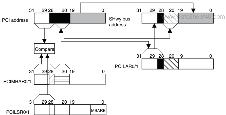
Figure 13.11 PCI Bus to SuperHyway Bus Address Translation
