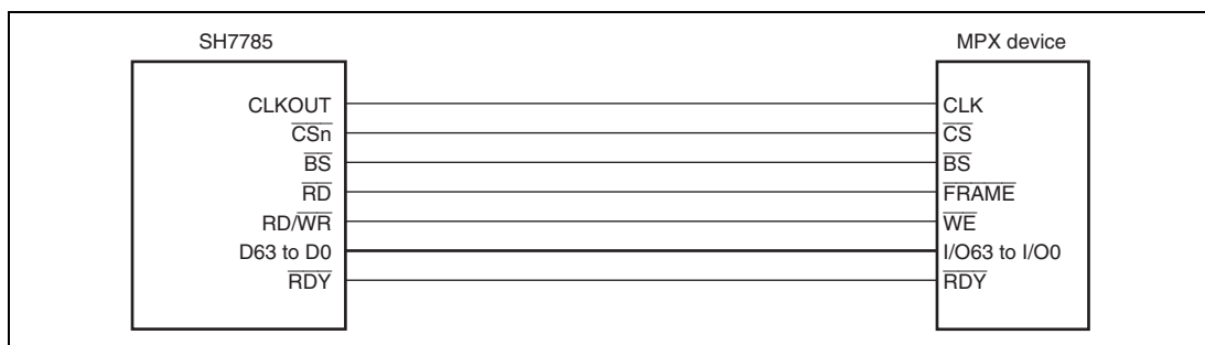
Figure 11.23 Example of 64-Bit Data Width MPX Connection
