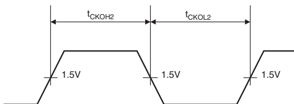
Figure 32.3 CLKOUT Clock Output Timing (2)
