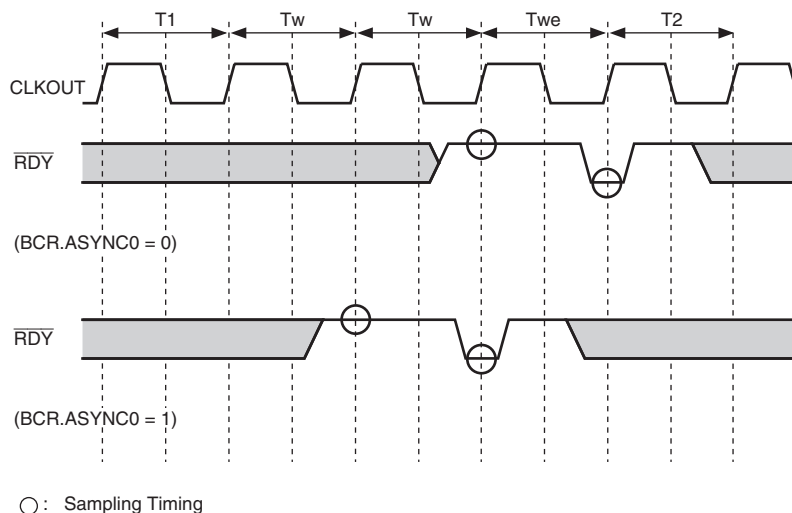
Figure 11.4 \overline{\text{RDY}} Sampling Timings with ASYN Cn Settings (Two Wait Cycles Inserted by CSnWCR.)
