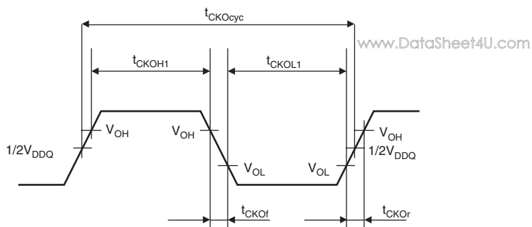
Figure 32.2 CLKOUT Clock Output Timing (1)
