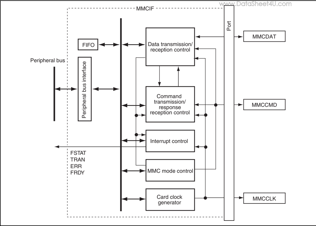
Figure 24.1 Block Diagram of MMCIF
