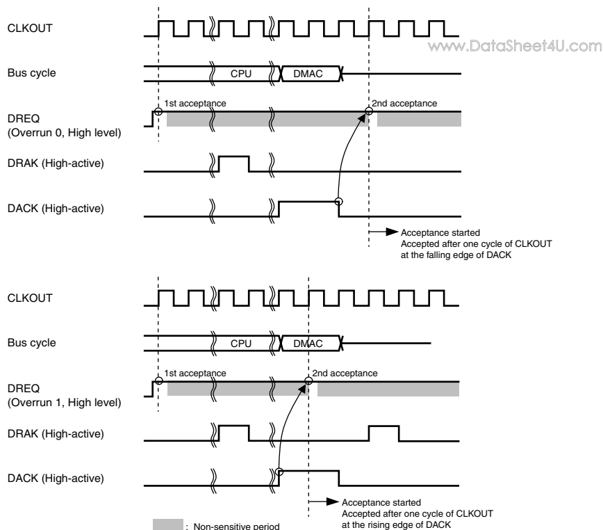
Figure 14.20 Example 1 of DREQ Input Detection in Burst Mode Level Detection (Byte Transfer in 8/16/32/64-Bit Bus Width, Word Transfer in 16/32/64-Bit Bus Width, or Longword Transfer in 32/64-Bit Bus Width)
