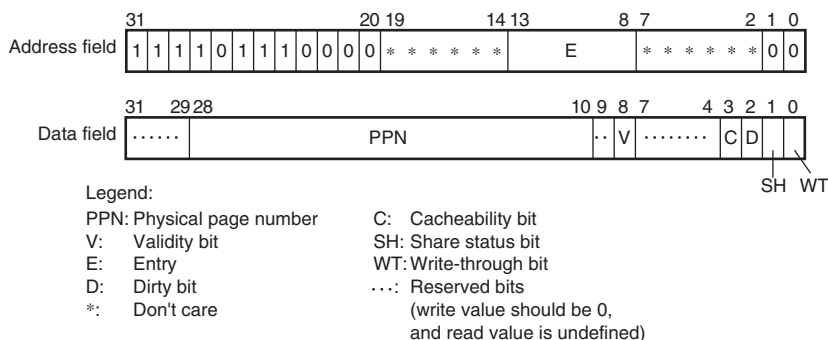
Figure 7.24 Memory-Mapped UTLB Data Array 1 (TLB Extended Mode)
