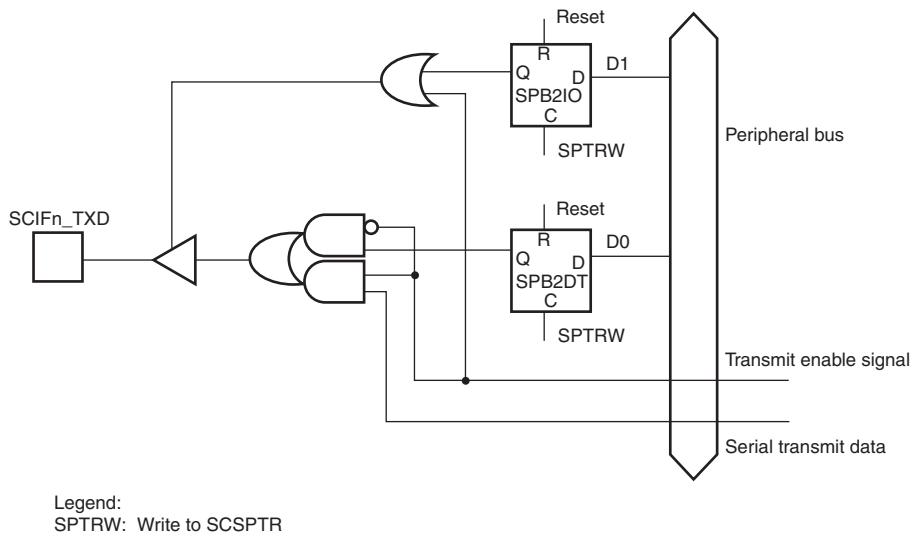
Figure 21.5 SCIF n _TXD Pin (n = 0 to 5)
