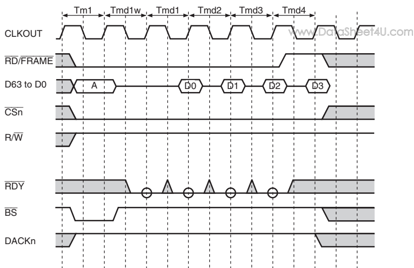
Figure 11.28 MPX Interface Timing 5 (Burst Read Cycle, IW = 0000, No External Wait, 64-Bit Bus Width, 32-Byte Data Transfer)
