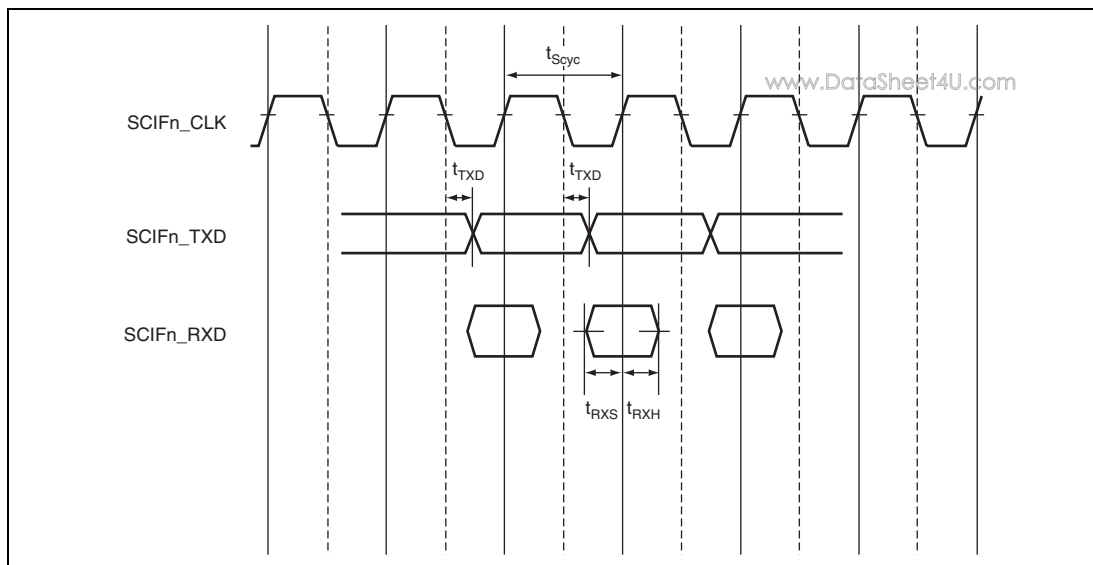
Figure 32.43 Clock Timing in SCIF I/O Synchronous Mode
