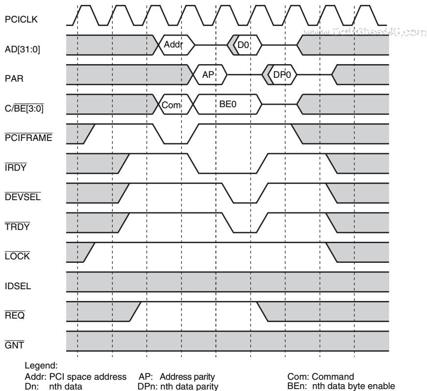
Figure 13.20 Master Read Cycle in Host Mode (Single)
