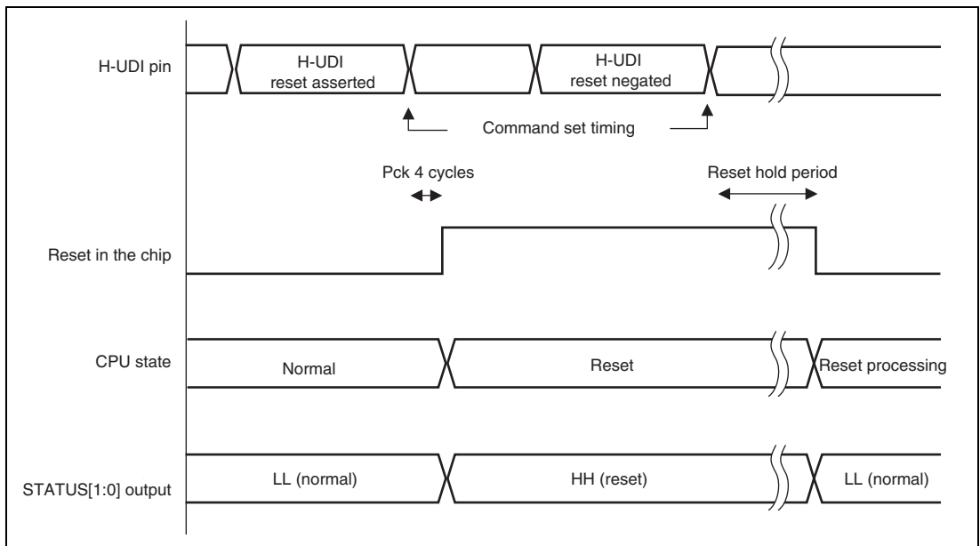
Figure 30.4 H-UDI Reset
