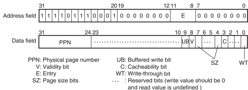
Figure 7.29 Memory-Mapped PMB Data Array
