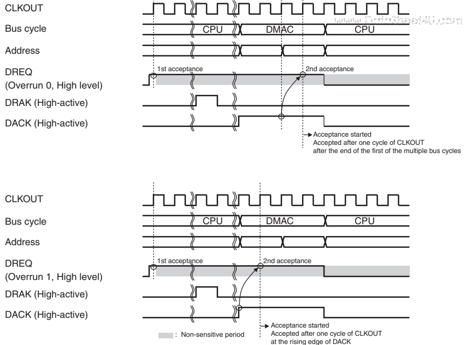
Figure 14.18 Example 3 of DREQ Input Detection in Cycle Steal Mode Level Detection (Word Transfer in 8-Bit Bus Width, Longword Transfer in 8/16-Bit Bus Width, or 16/32-Byte Transfer in 8/16/32/64-Bit Bus Width: DACK of DMA1 Transfer Is Connected)
