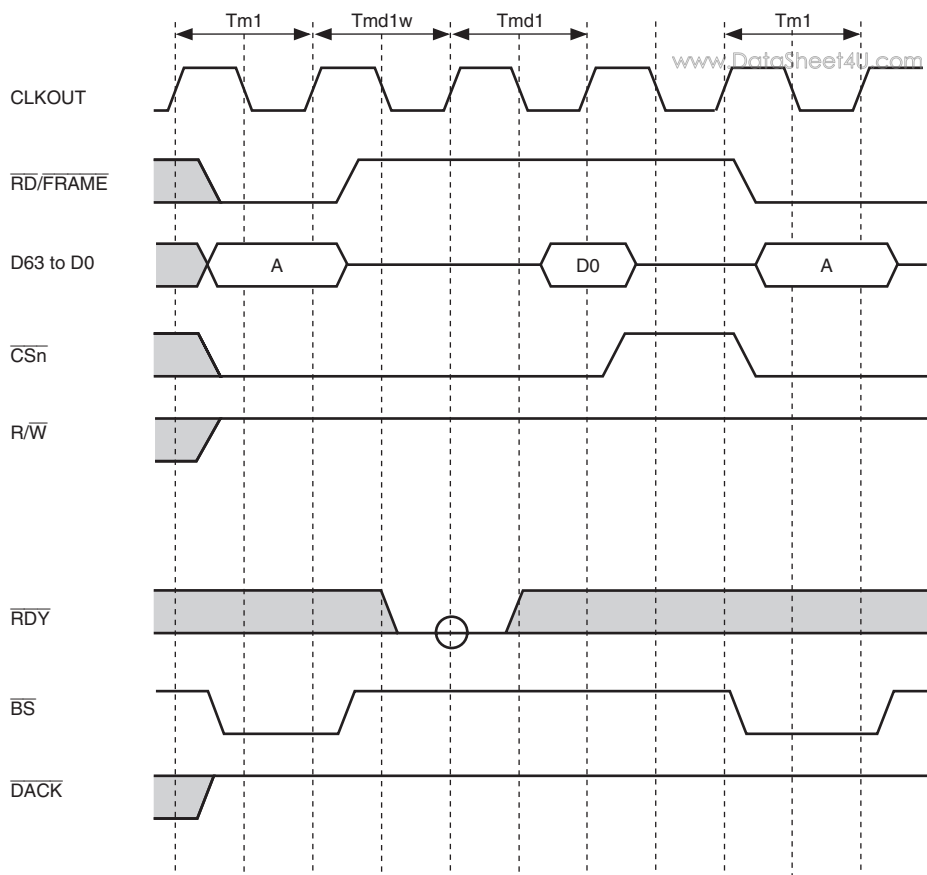
Figure 11.24 MPX Interface Timing 1 (Single Read Cycle, IW = 0000, No External Wait, 64-Bit Bus Width)
