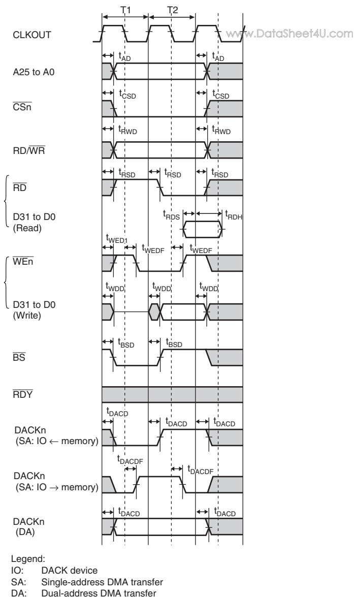
Figure 32.9 SRAM Bus Cycle: Basic Bus Cycle (No Wait)
