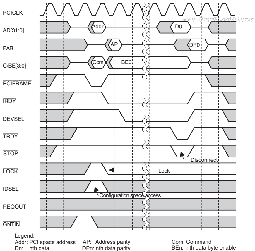
Figure 13.23 Target Read Cycle in Normal Mode (Single)
