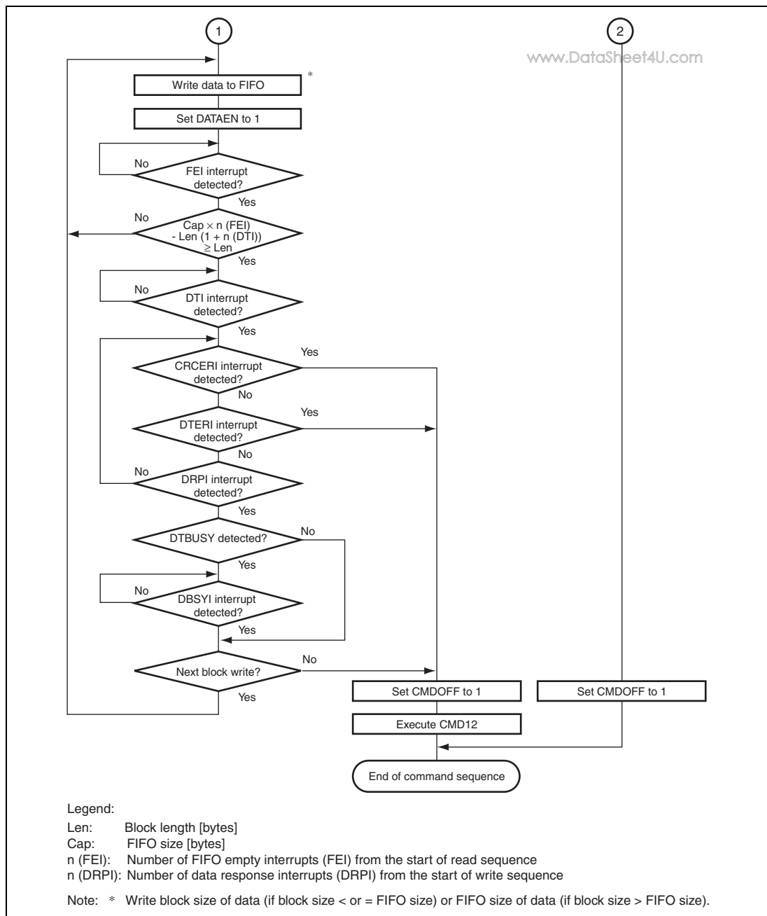
Figure 24.20 (2) Example of Operational Flow for Commands with Write Data (Open-ended Multiple Block Transfer)
