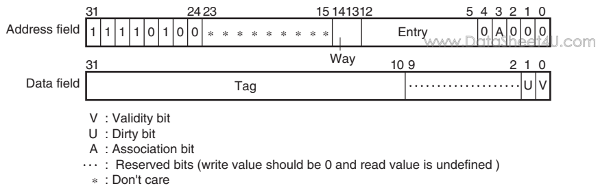
Figure 8.7 Memory-Mapped OC Address Array (Cache size = 32 Kbytes)
