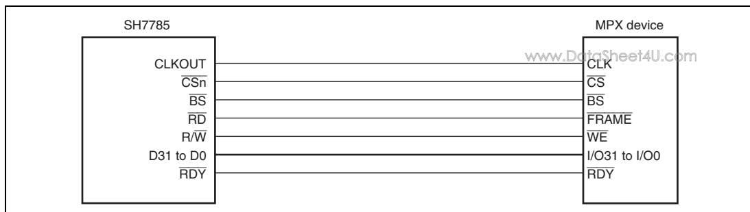
Figure 11.22 Example of 32-Bit Data Width MPX Connection
