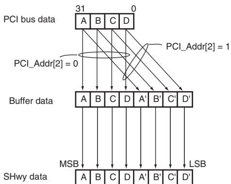
Figure 13.13 Endian Conversion from PCI Bus to SuperHyway Bus (Non-Byte Swapping: TBS = 0)
