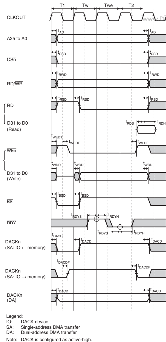
Figure 32.11 SRAM Bus Cycle: Basic Bus Cycle (One Internal Wait Cycle + One External Wait Cycle)
