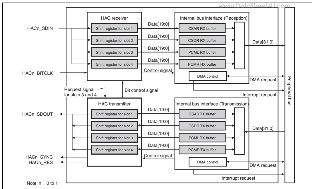
Figure 25.1 Block Diagram
