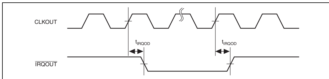
Figure 32.36 \overline{\text{IRQOUT}} Timing
