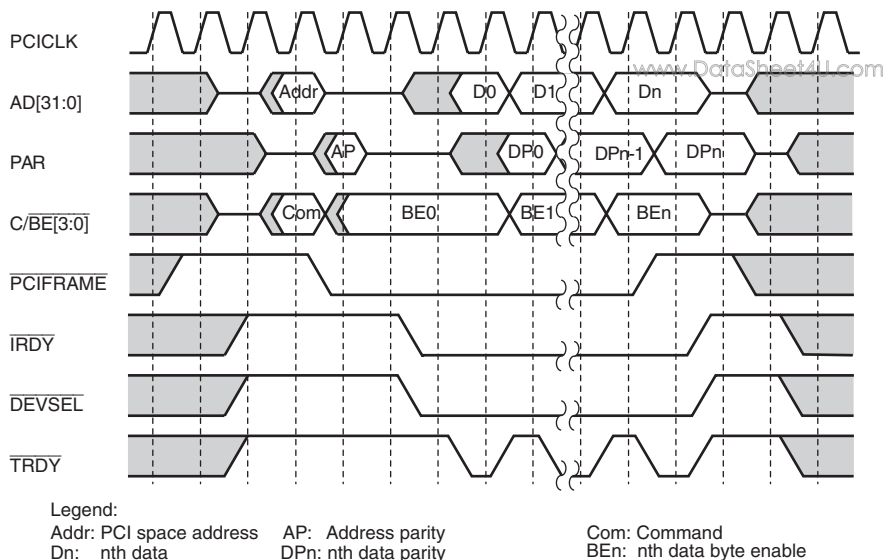
Figure 13.28 Target Memory Read Cycle in Host Bus Bridge Mode (Burst, with Stepping)
