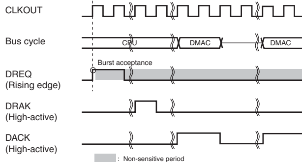
Figure 14.19 Example of DREQ Input Detection in Burst Mode Edge Detection
