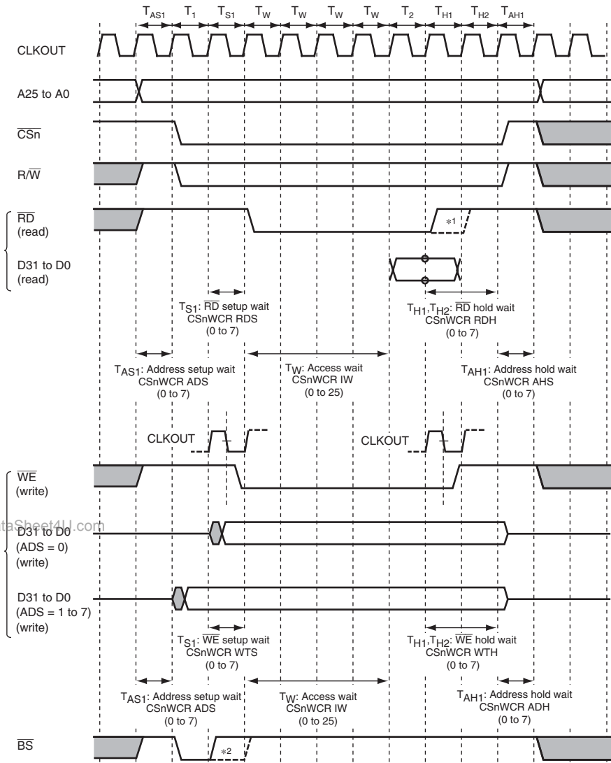
Figure 11.9 SRAM Interface Wait State Timing (Read-Strobe Negate Timing Setting)
