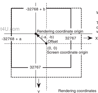
Figure 23.4 Rendering Coordinates
