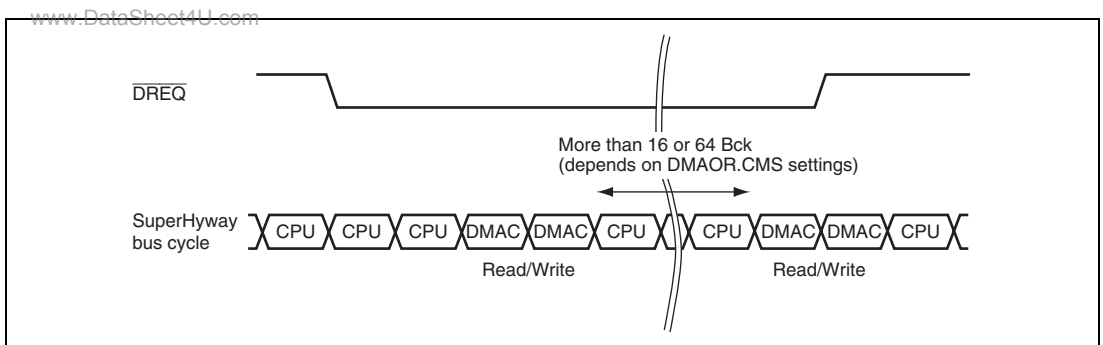
Figure 12.8 Example of DMA Transfer Timing in Cycle Steal Intermittent Mode (DREQ Low Level Detection)
