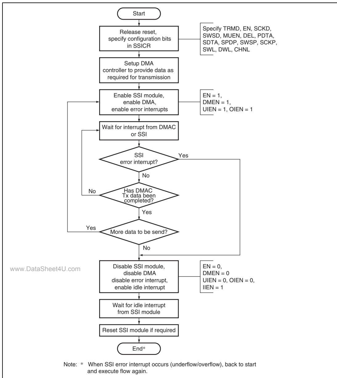
Figure 18.19 Transmission Using SSI_DMACH0 and SSI_DMACH1
