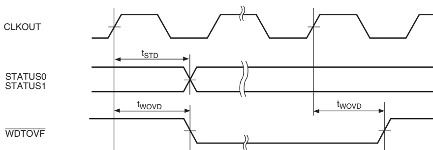
Figure 33.6 Pin Drive Timing in Standby
