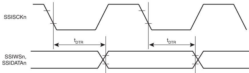
Figure 33.34 SSI Transmit Timing (2)
