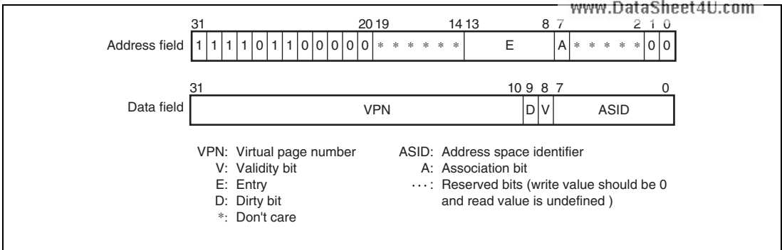
Figure 7.22 Memory-Mapped UTLB Address Array
