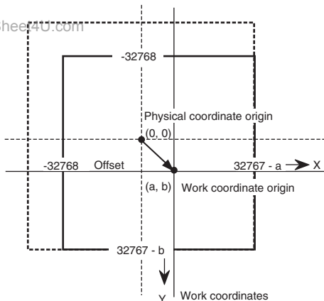
Figure 23.5 Work Coordinates
