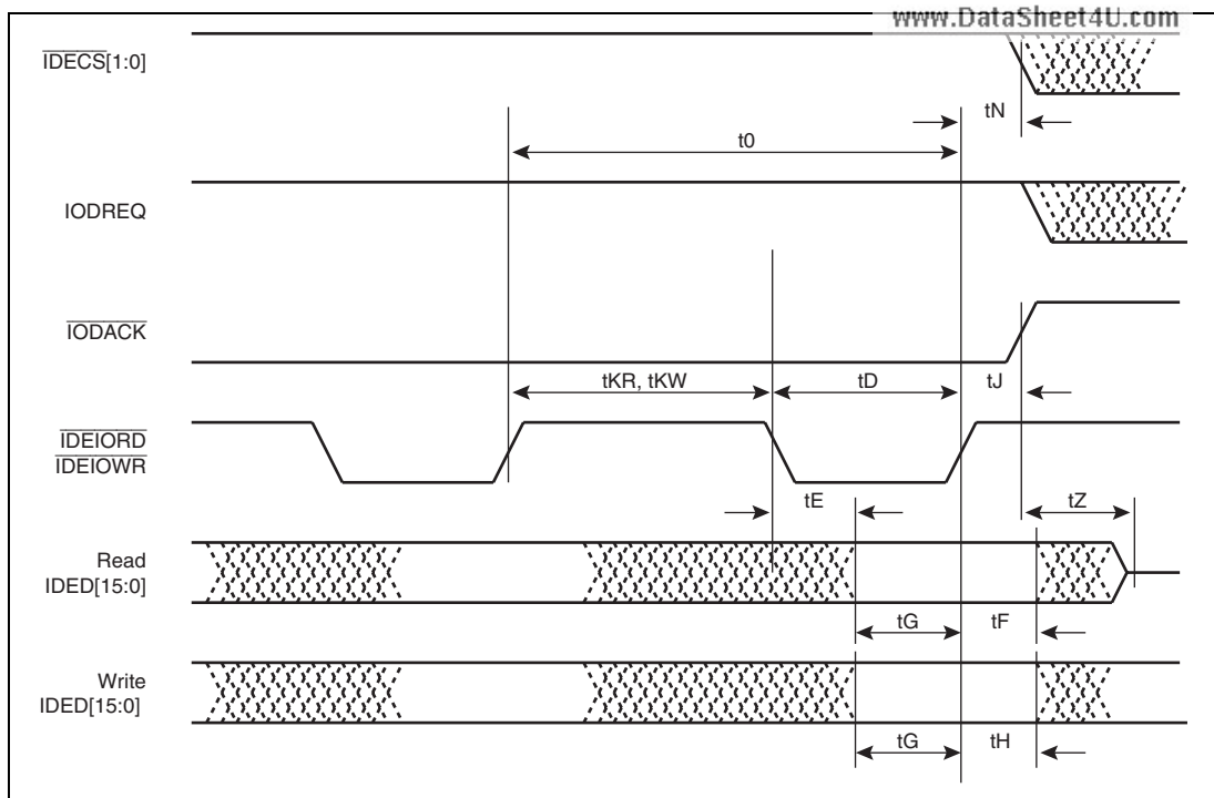
Figure 33.42 End of Multiword Data Transmission from Host
