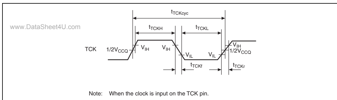
Figure 33.64 TCK Input Timing
