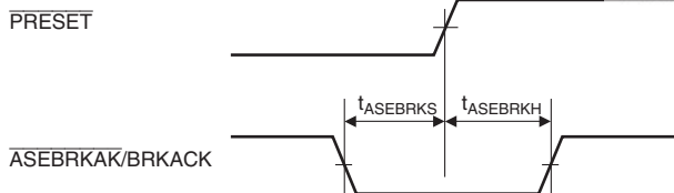
Figure 33.65 PRESET Hold Timing
