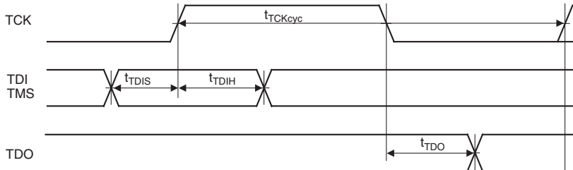
Figure 33.66 H-UDI Data Transmission Timing
