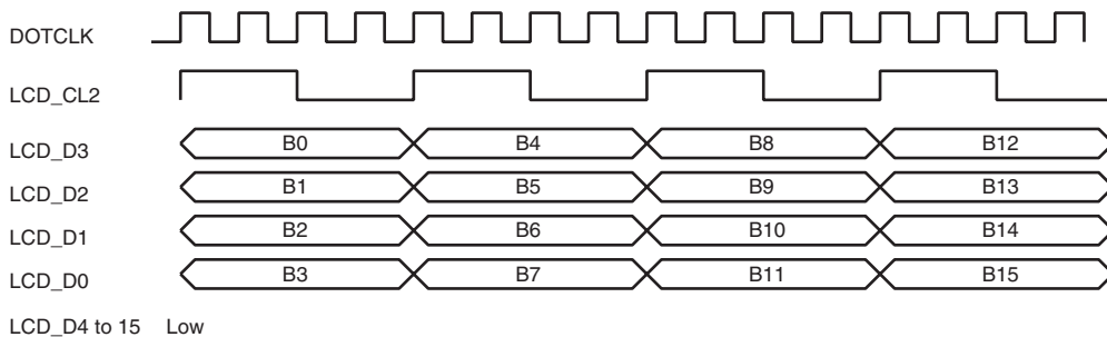
Figure 22.8 Clock and LCD Data Signal Example
