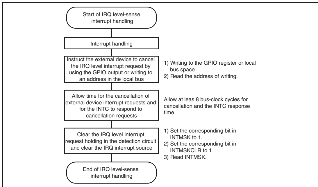
www.DataSheet4U.com Figure 13.4 Example of Interrupt Handling Routine
