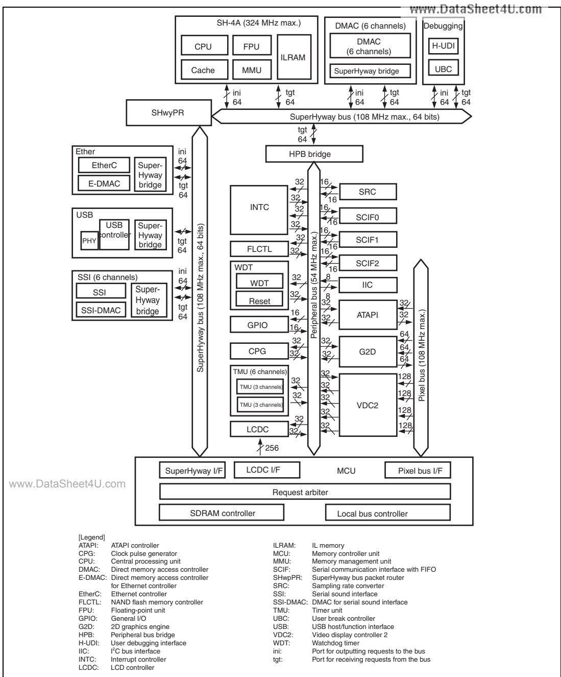
Figure 1.1 Block Diagram
