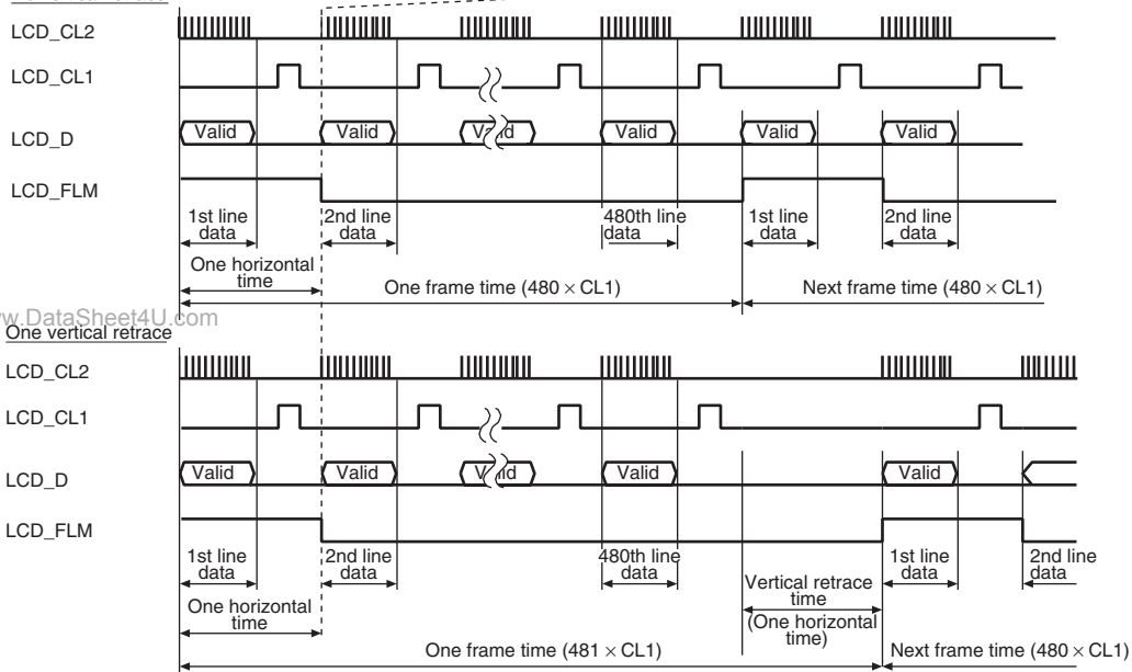
Figure 22.21 Clock and LCD Data Signal Example (8-Bit Interface Color 640 × 480)
