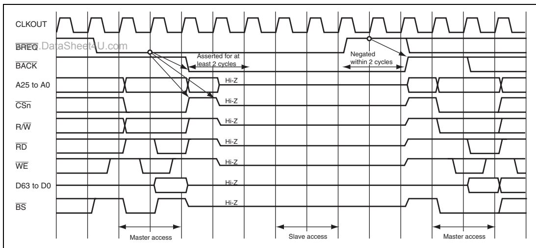
Figure 11.23 Arbitration Sequence
