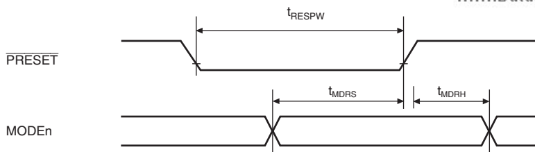
Figure 33.5 MODE Pin Setup / Hold Timing
