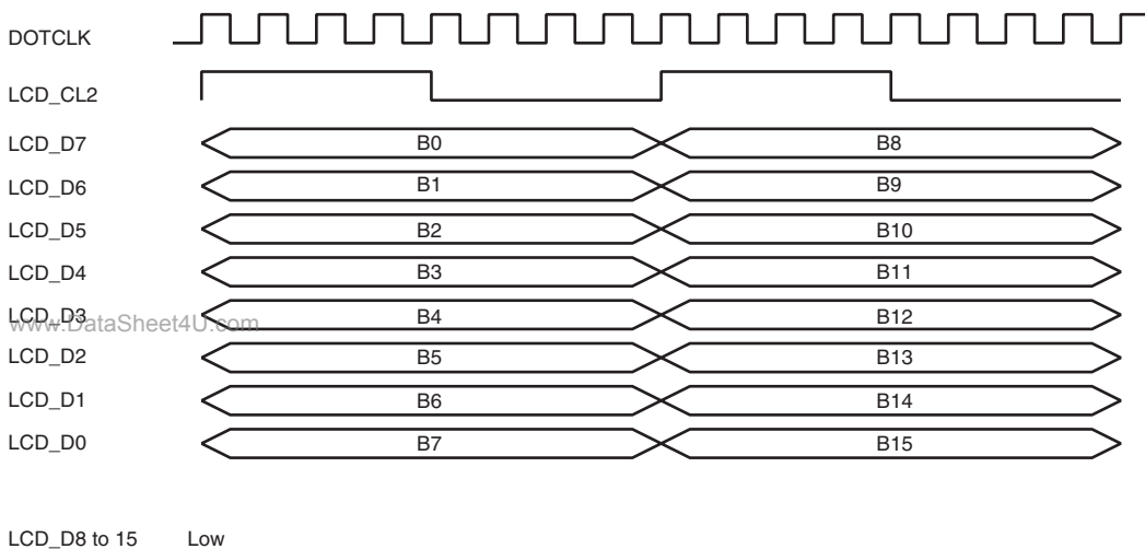
Figure 22.9 Clock and LCD Data Signal Example (STN Monochrome 8-Bit Data Bus Module)
