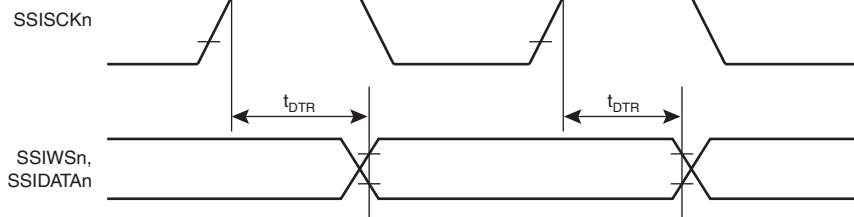
Figure 33.33 SSI Transmit Timing (1)
