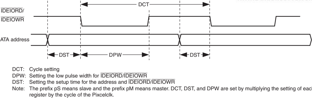
Figure 17.2 PIO Timing Register
