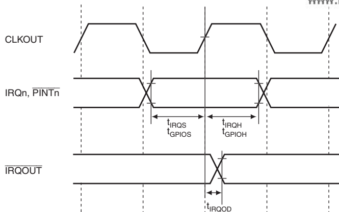
Figure 33.25 IRQ, \overline{\text{PINTn}} Input, \overline{\text{IRQOUT}} Output Timing
