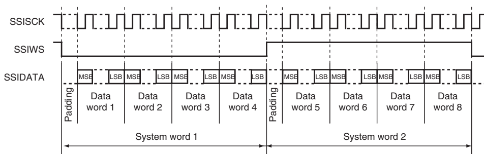
Figure 18.8 Multichannel Format (4 Channels, with Padding Bits First, Followed by Serial Data, with Padding)
