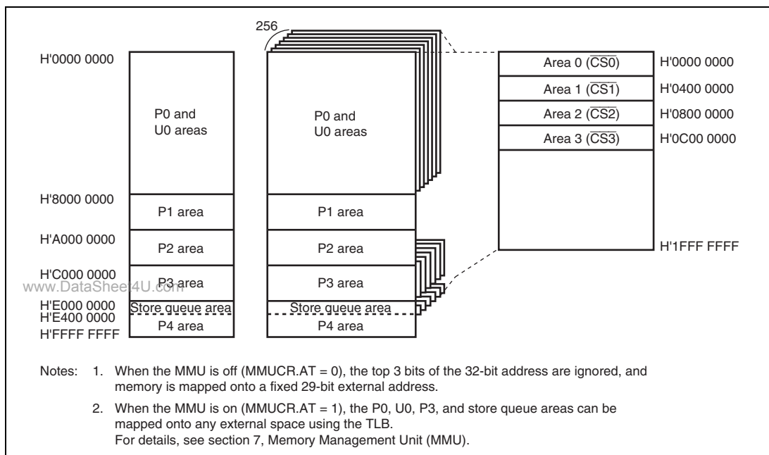
Figure 11.2 Correspondence between Virtual Address Space and External Memory Space
