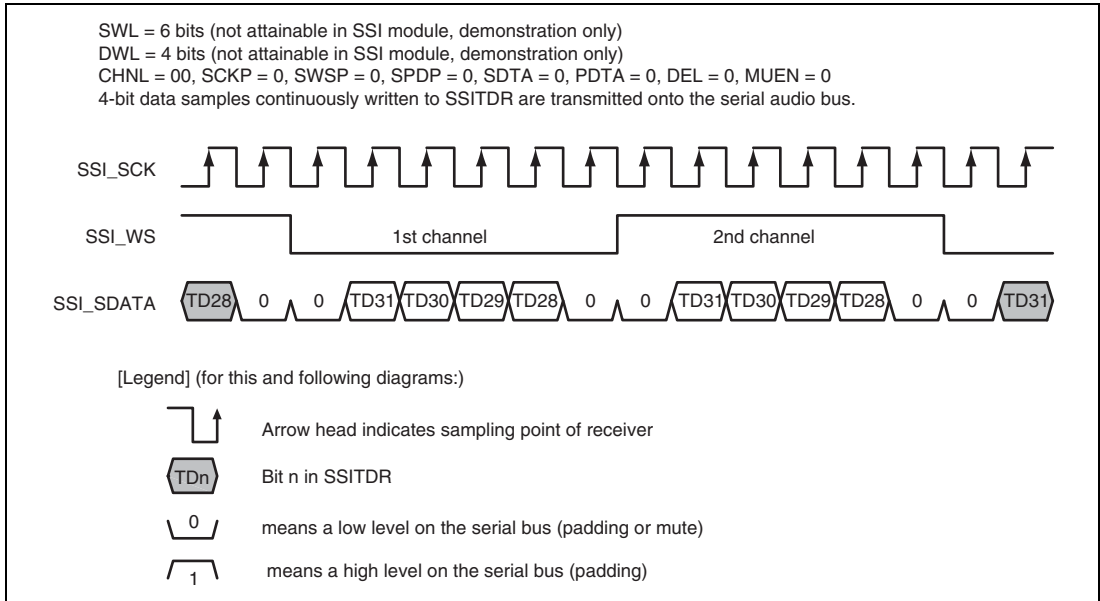
Figure 18.9 Basic Sample Format
