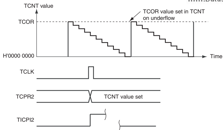
Figure 14.6 Operation Timing when Using Input Capture Function
