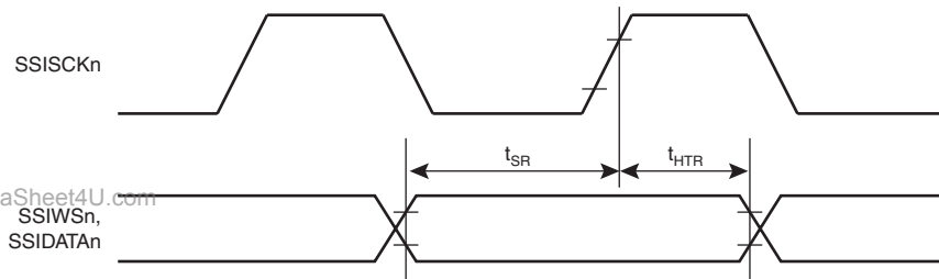
Figure 33.35 SSI Receive Timing (1)
