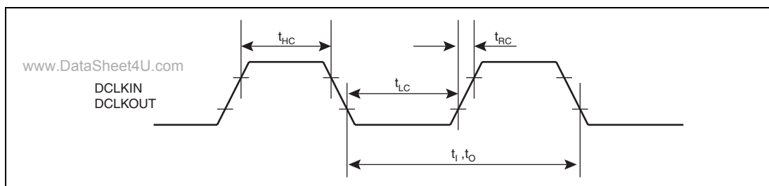
Figure 33.82 Clock Input/Output Timing
