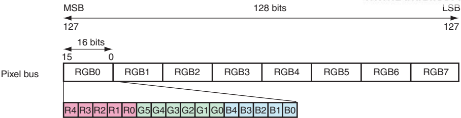
Figure 24.8 Pixel Bus Endian (ENDIAN = 1)
