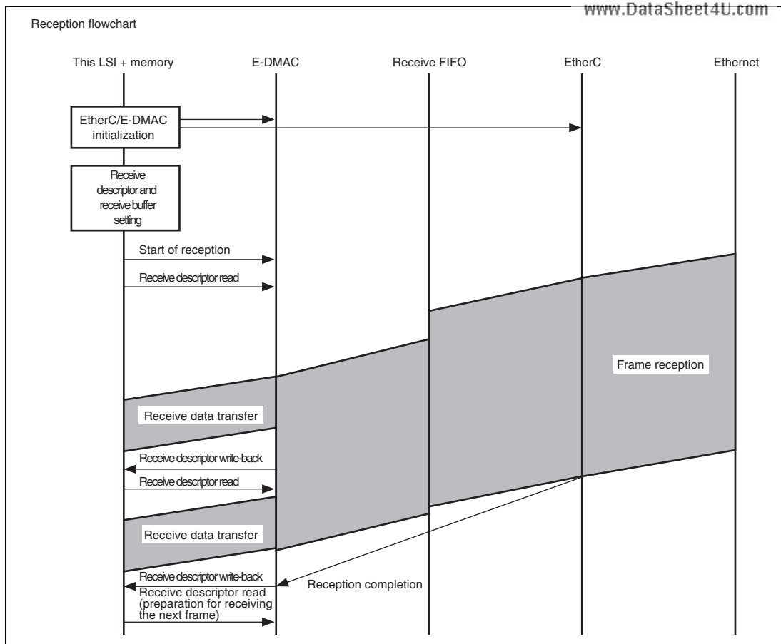
www.DataSheet4U.com Figure 20.5 Sample Reception Flowchart (Single-Frame/Two-Descriptor)
