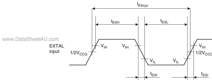
Figure 33.2 EXTAL Clock Input Timing
