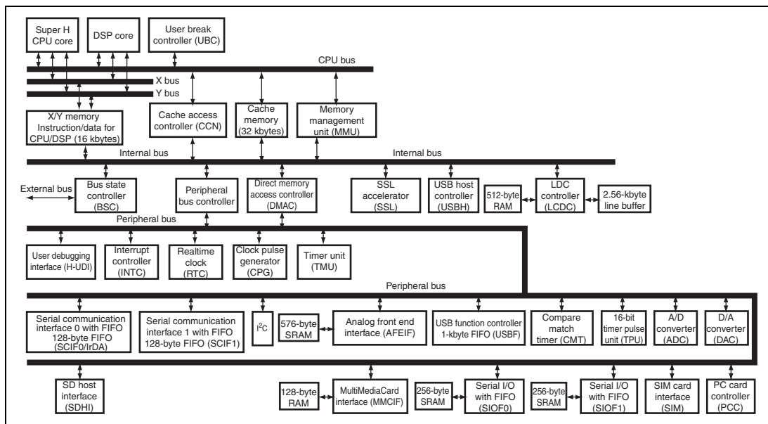
Figure 1.1 Block Diagram
