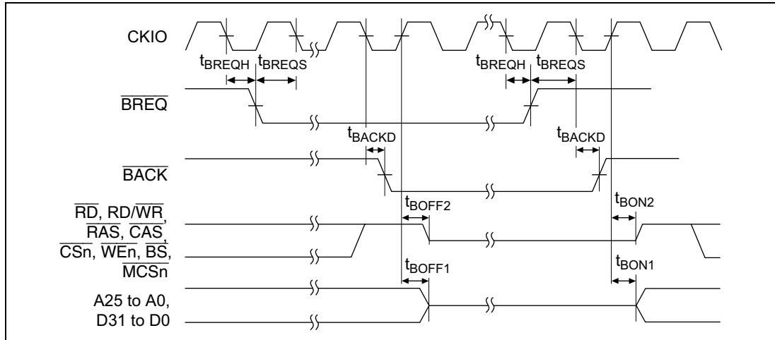
Figure 23.14 Bus Release Timing
