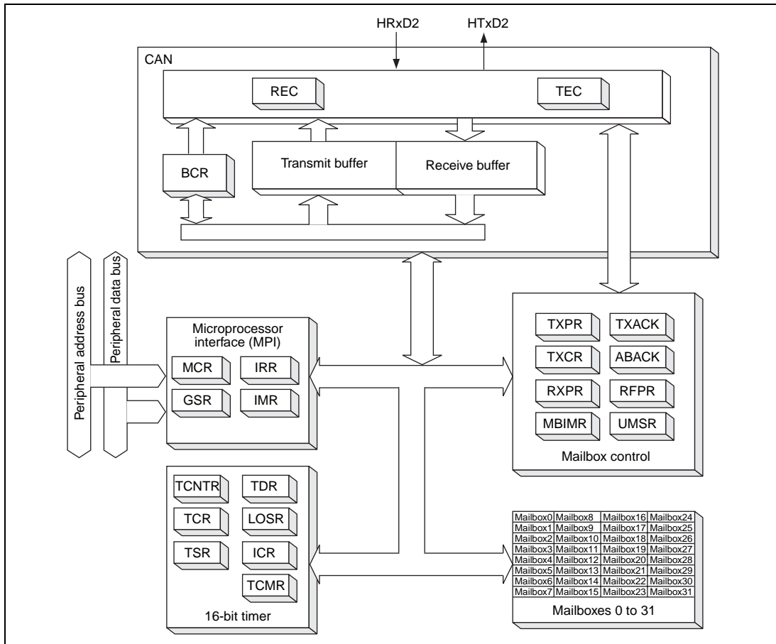
Figure 15.1 HCAN2 Block Diagram
