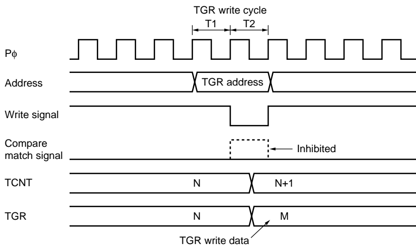
Figure 10.74 Contention between TGR Write and Compare Match
