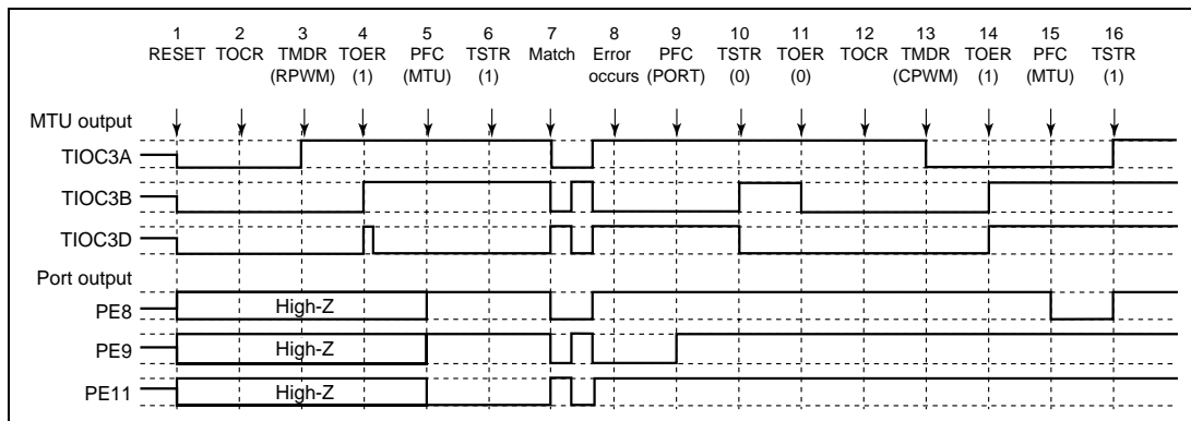
Figure 10.113 Error Occurrence in Reset-Synchronous PWM Mode, Recovery in Complementary PWM Mode
