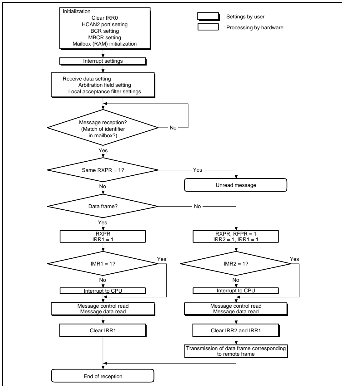
Figure 15.10 Reception Flowchart
