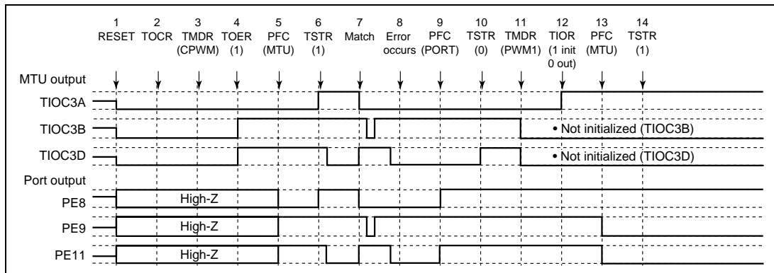
Figure 10.107 Error Occurrence in Complementary PWM Mode, Recovery in PWM Mode 1
