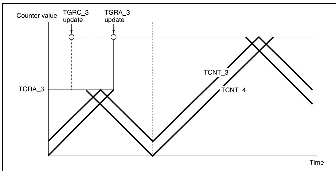
Figure 10.37 Example of PWM Cycle Updating
