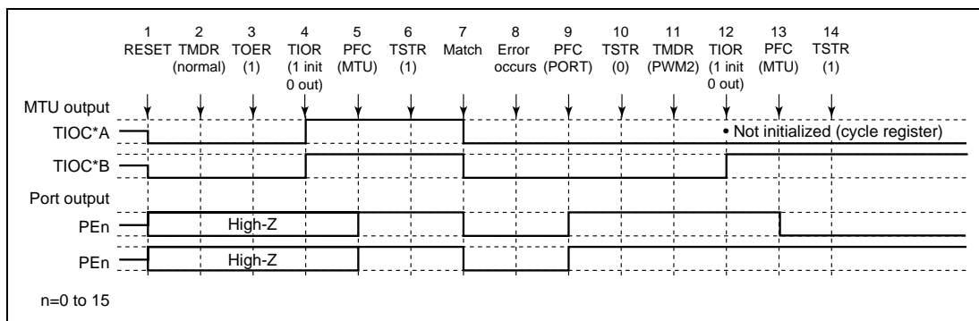
Figure 10.88 Error Occurrence in Normal Mode, Recovery in PWM Mode 2
