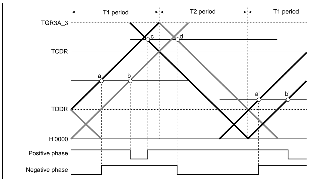
Figure 10.41 Example of Complementary PWM Mode Waveform Output (1)
