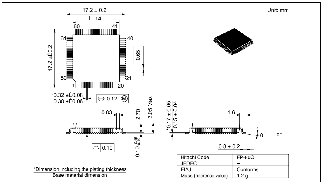
Figure D.2 FP-80Q
