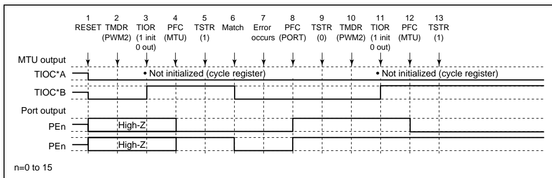
Figure 10.100 Error Occurrence in PWM Mode 2, Recovery in PWM Mode 2
