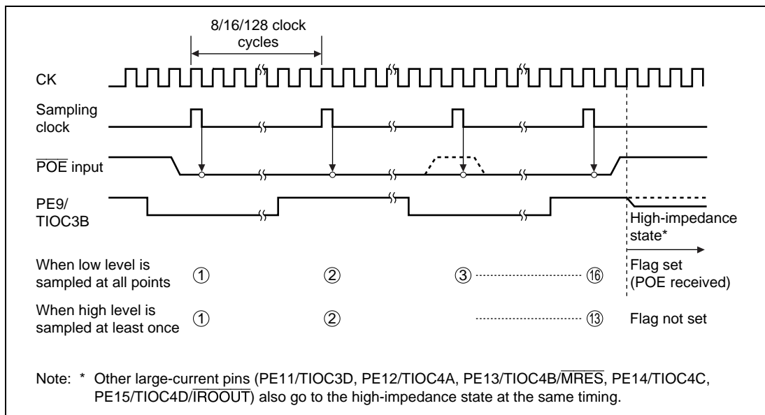
Figure 10.116 Low-Level Detection Operation
