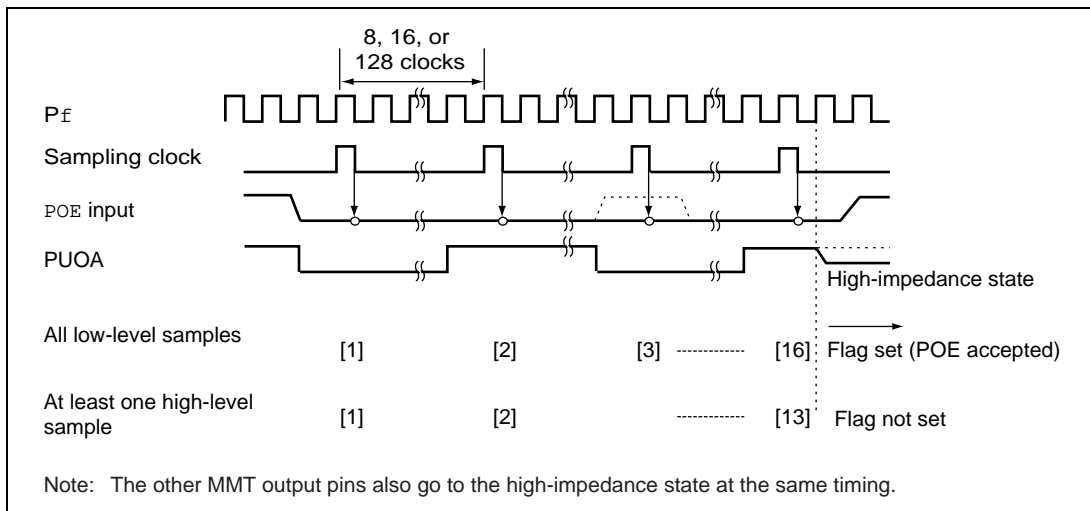
Figure 16.18 Low Level Detection Operation
