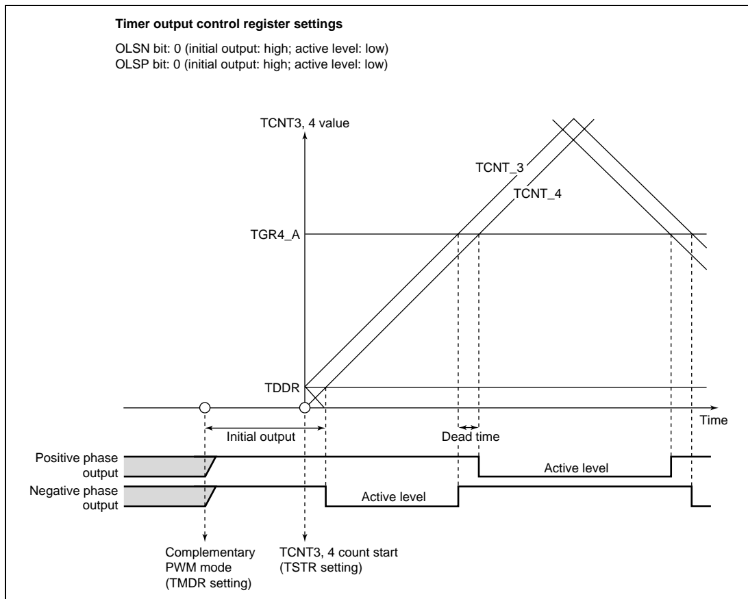
Figure 10.39 Example of Initial Output in Complementary PWM Mode (1)
