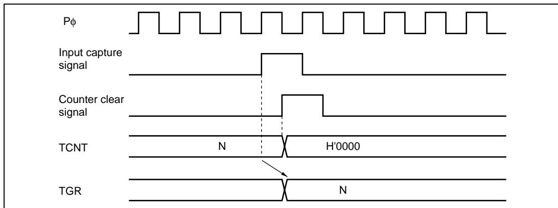
Figure 10.62 Counter Clear Timing (Input Capture)
