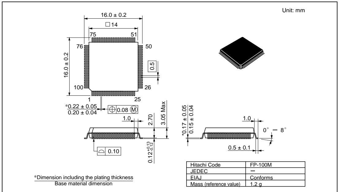
Figure D.1 FP-100M
