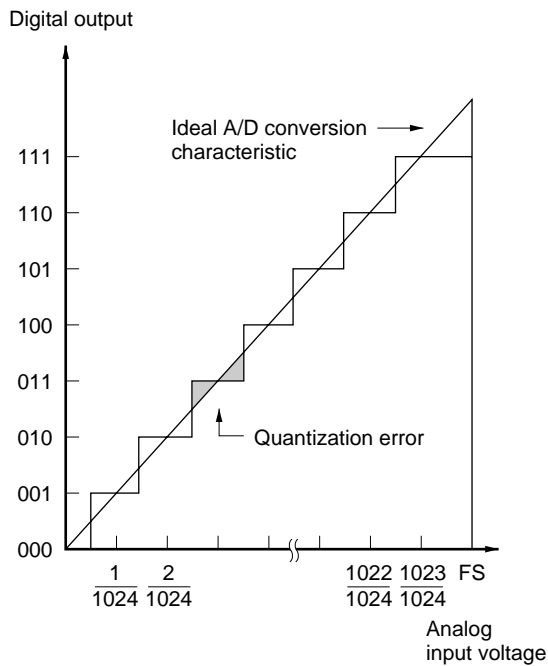
Figure 13.4 A/D Conversion Precision Definitions
