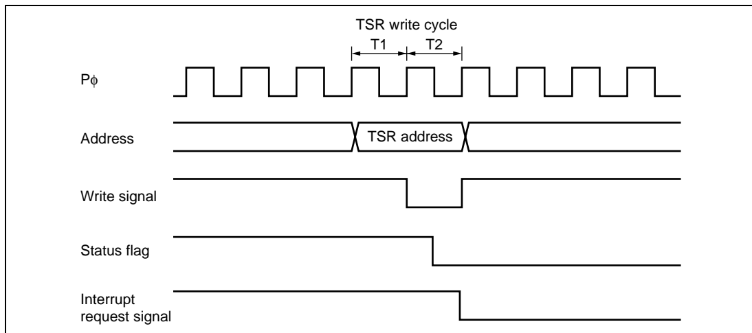
Figure 10.69 Timing for Status Flag Clearing by the CPU
