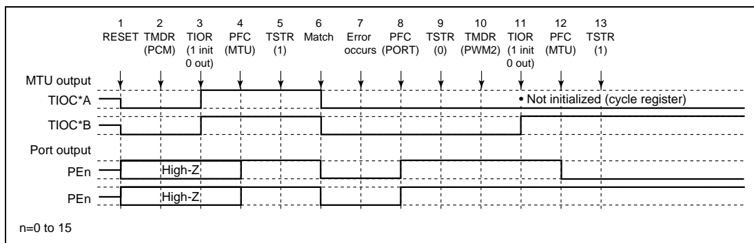
Figure 10.104 Error Occurrence in Phase Counting Mode, Recovery in PWM Mode 2
