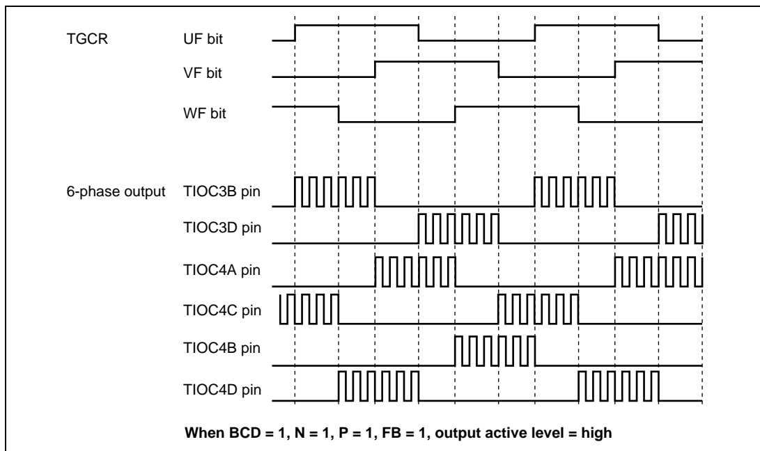
Figure 10.54 Example of Output Phase Switching by Means of UF, VF, WF Bit Settings (2)
