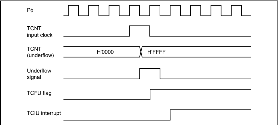
Figure 10.68 TCIU Interrupt Setting Timing
