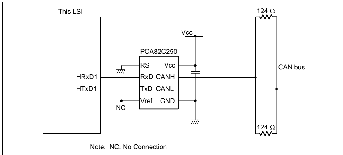
Figure 15.15 High-Speed Interface Using PCA82C250
