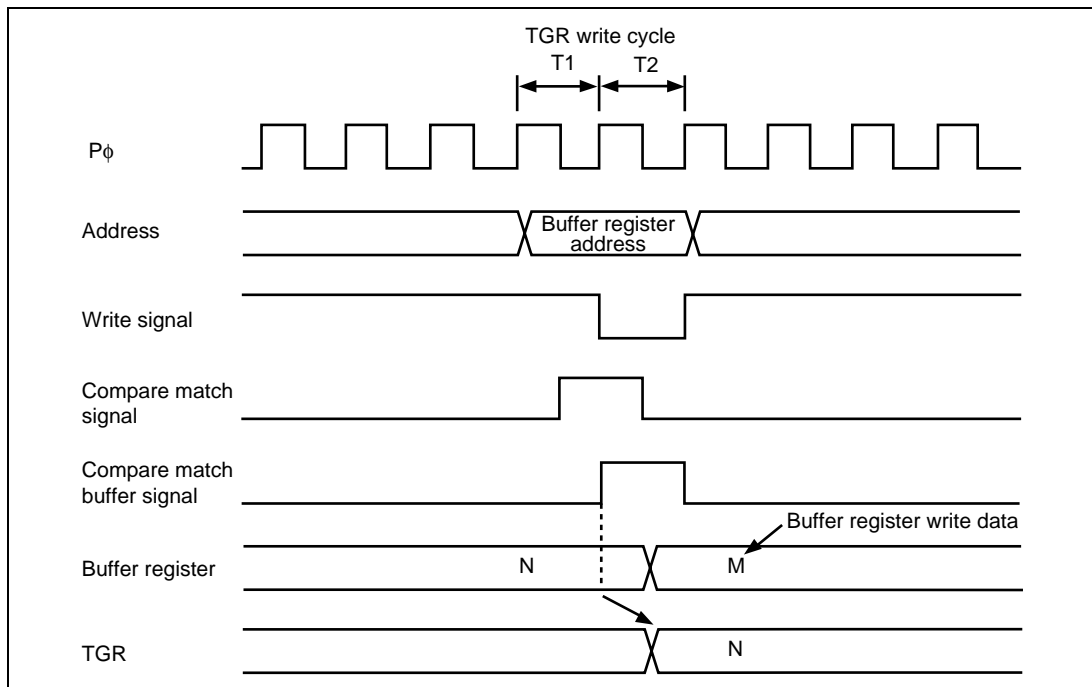
Figure 10.76 Contention between Buffer Register Write and Compare Match (Channels 3 and 4)
