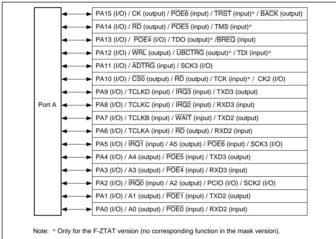
Figure 18.2 Port A (SH7047)
