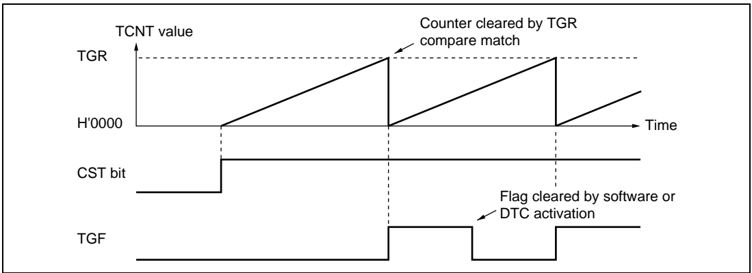
Figure 10.5 Periodic Counter Operation
