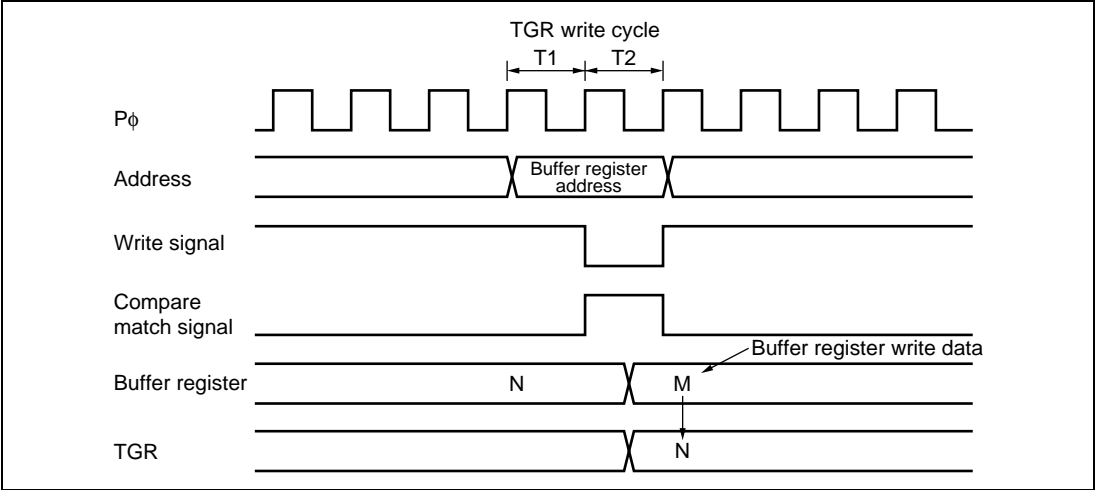
Figure 10.75 Contention between Buffer Register Write and Compare Match (Channel 0)
