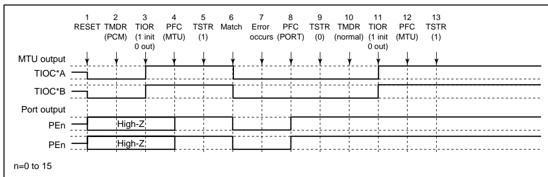
Figure 10.102 Error Occurrence in Phase Counting Mode, Recovery in Normal Mode
