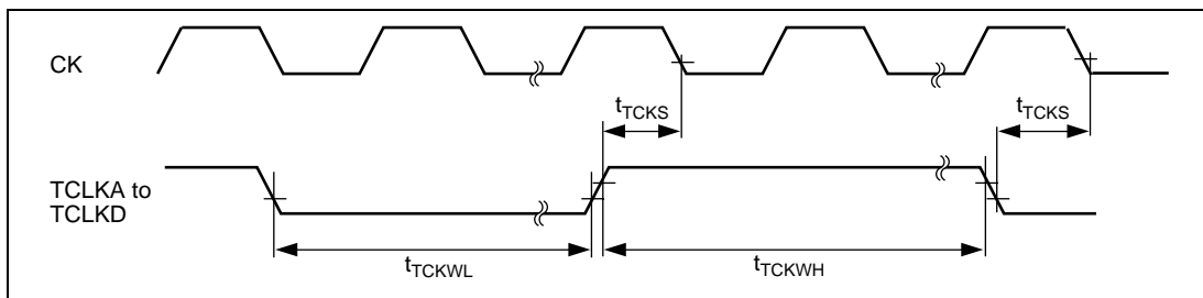
Figure 25.14 MPU Clock Input Timing
