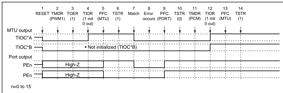
Figure 10.95 Error Occurrence in PWM Mode 1, Recovery in Phase Counting Mode
