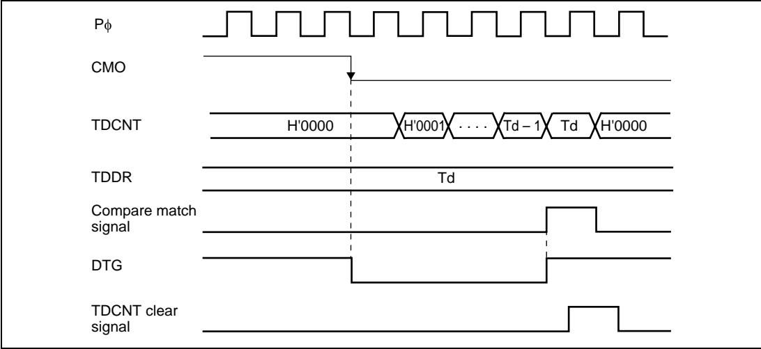
Figure 16.10 TDCNT Operation Timing
