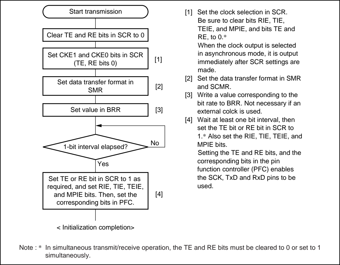
Figure 12.5 Sample SCI Initialization Flowchart
