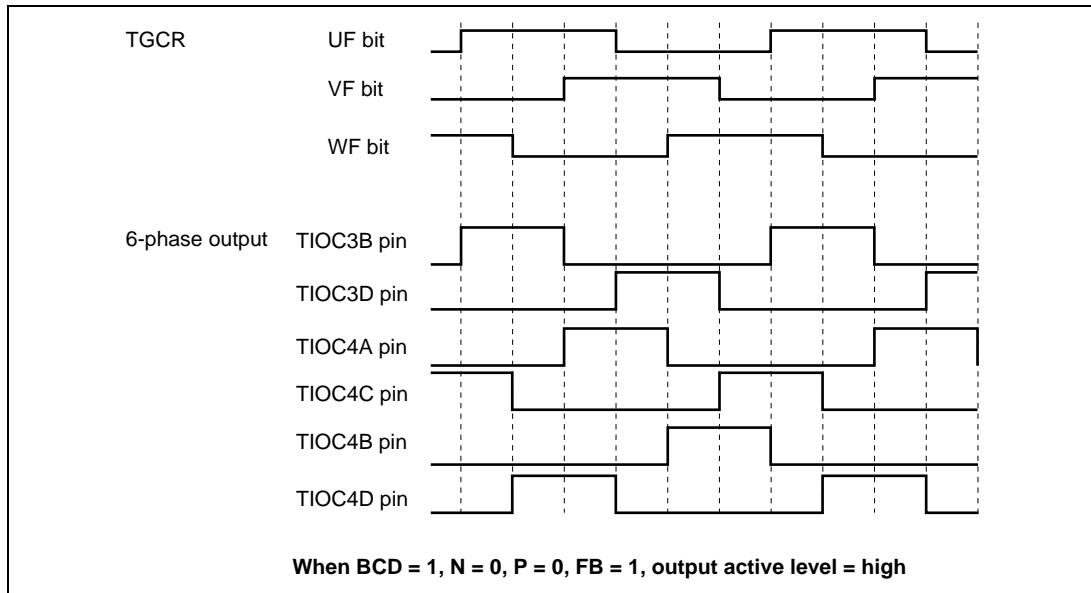
Figure 10.53 Example of Output Phase Switching by Means of UF, VF, WF Bit Settings (1)
