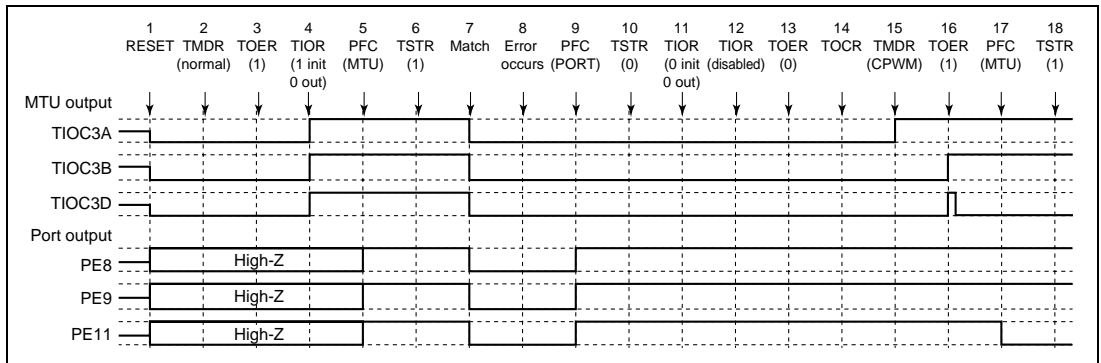
Figure 10.91 Error Occurrence in Normal Mode, Recovery in Reset-Synchronous PWM Mode
