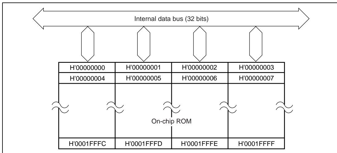
Figure 20.2 Mask ROM Block Diagram (SH7047)
