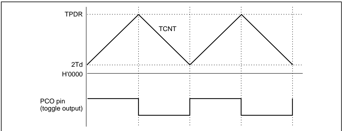
Figure 16.7 Example of Toggle Output Waveform Synchronized with PWM Period
