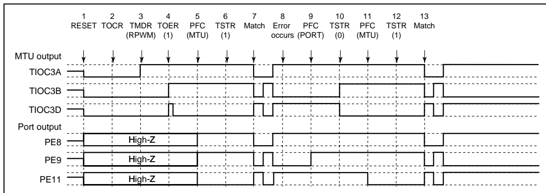
Figure 10.114 Error Occurrence in Reset-Synchronous PWM Mode, Recovery in Reset-Synchronous PWM Mode
