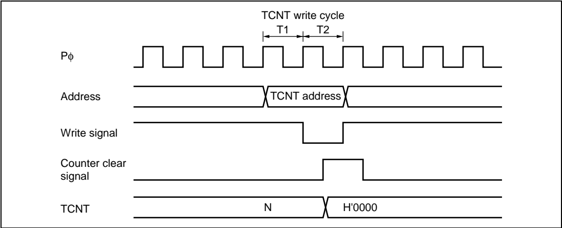
Figure 10.72 Contention between TCNT Write and Clear Operations
