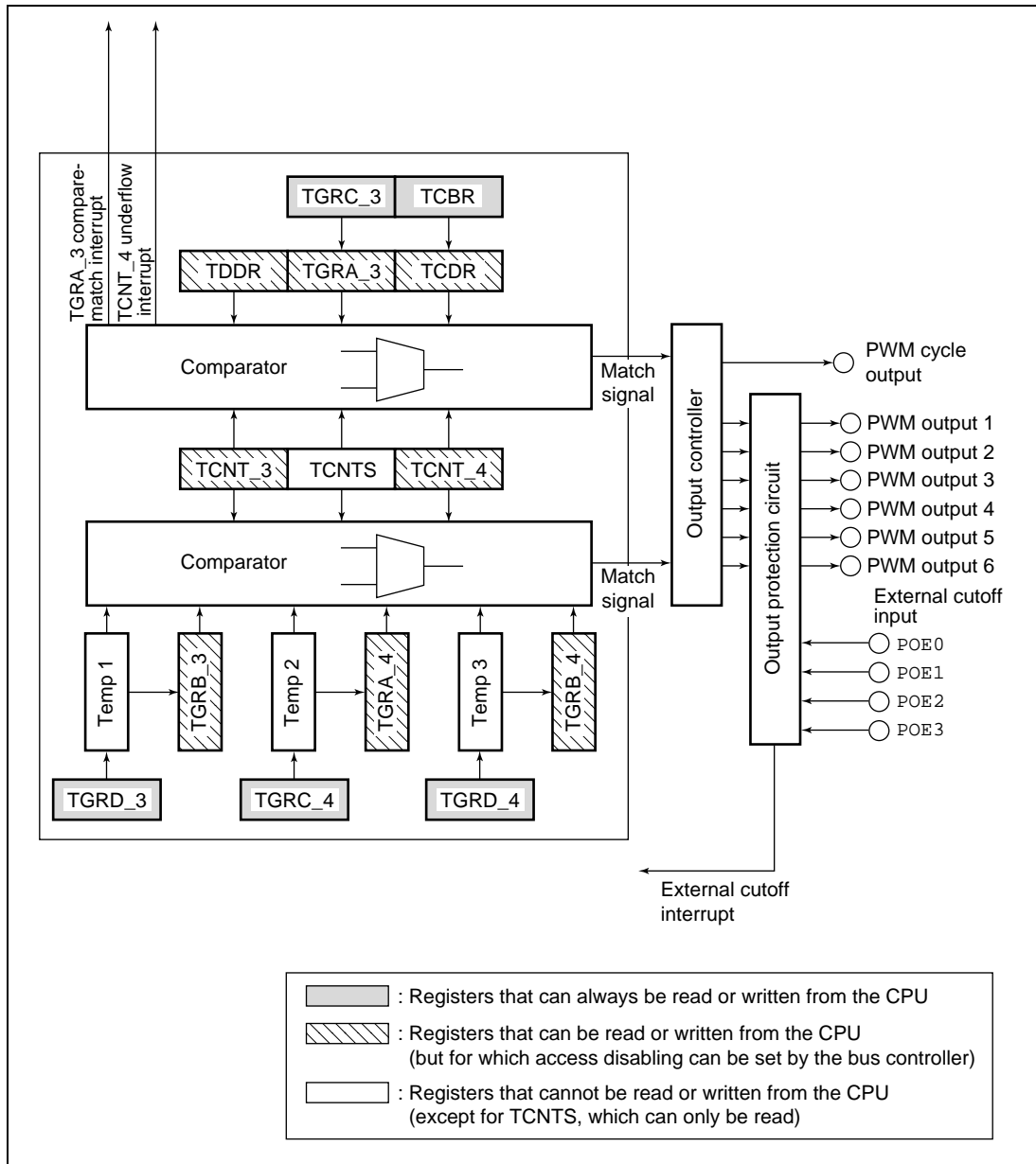
Figure 10.33 Block Diagram of Channels 3 and 4 in Complementary PWM Mode
