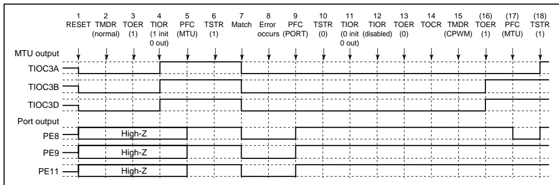
Figure 10.90 Error Occurrence in Normal Mode, Recovery in Complementary PWM Mode
