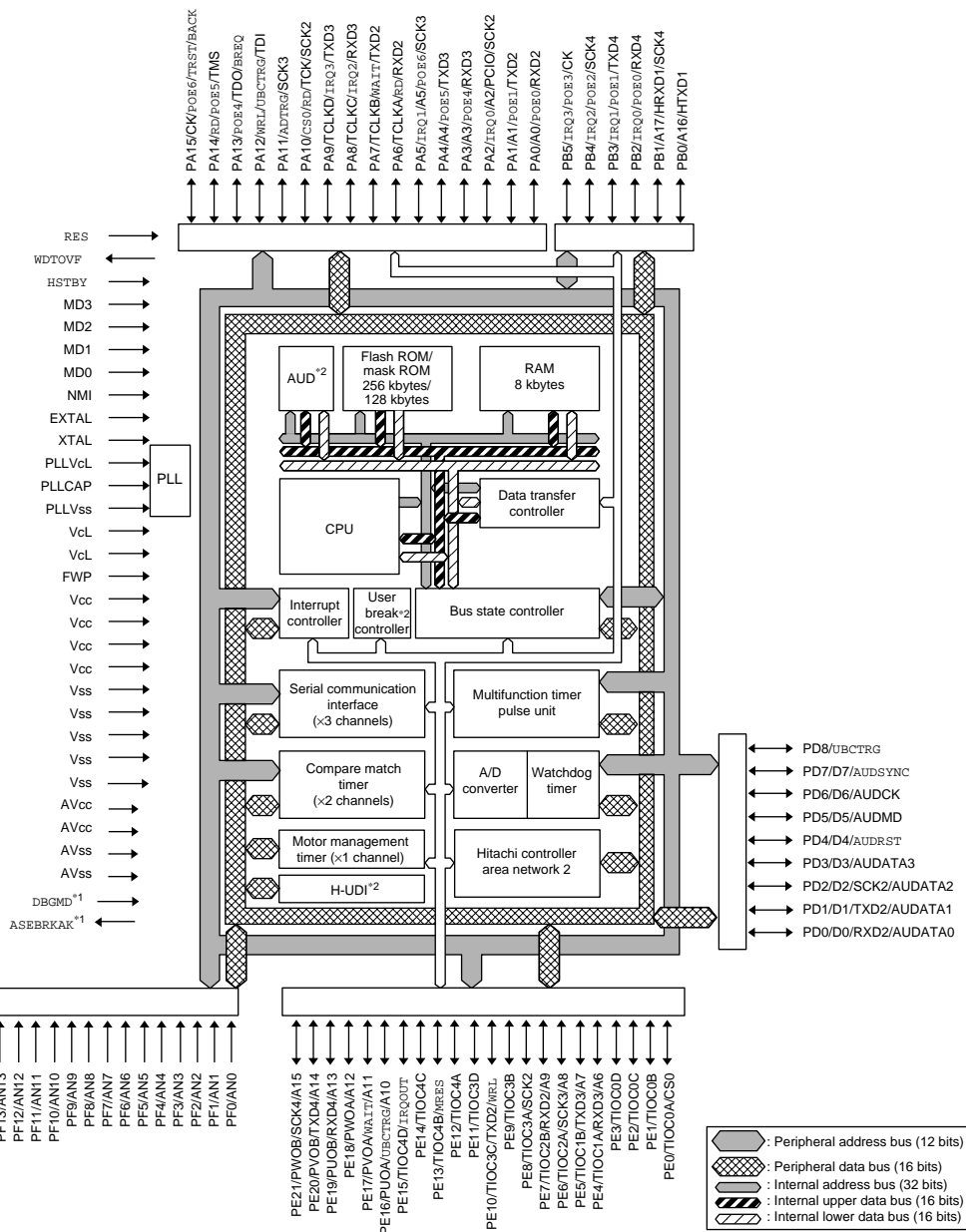
Figure1.2 Block Diagram of SH7047
