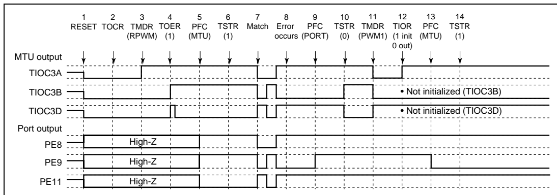
Figure 10.112 Error Occurrence in Reset-Synchronous PWM Mode, Recovery in PWM Mode 1
