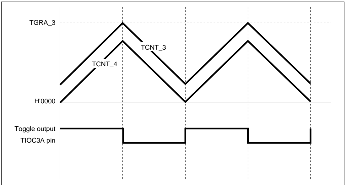
Figure 10.49 Example of Toggle Output Waveform Synchronized with PWM Output
