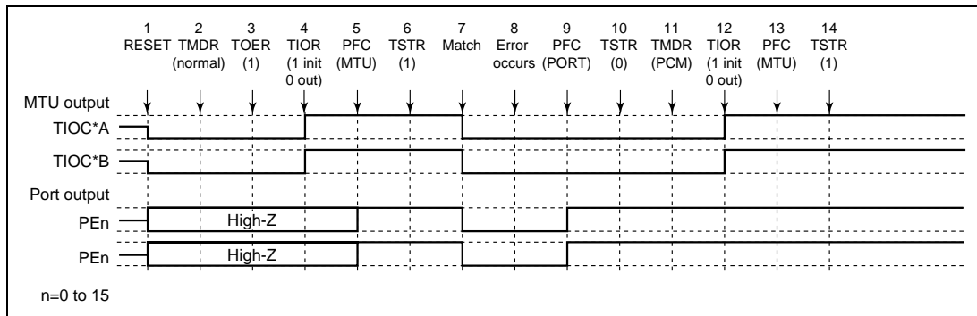
Figure 10.89 Error Occurrence in Normal Mode, Recovery in Phase Counting Mode
