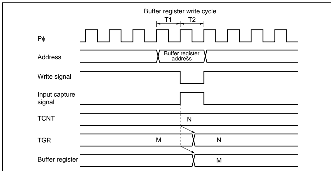
Figure 10.79 Contention between Buffer Register Write and Input Capture
