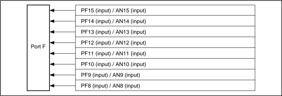
Figure 18.8 Port F (SH7046)
