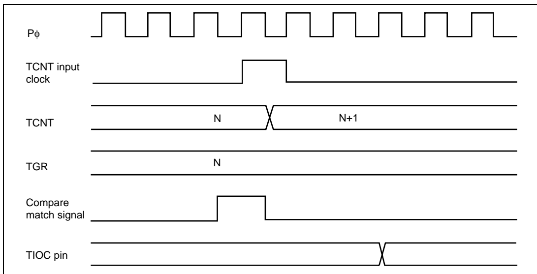
Figure 10.59 Output Compare Output Timing (Complementary PWM Mode/Reset Synchronous PWM Mode)
