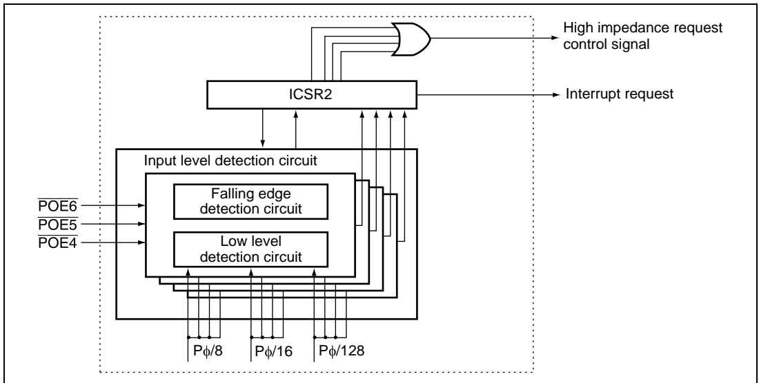
Figure 16.17 Block Diagram of POE
