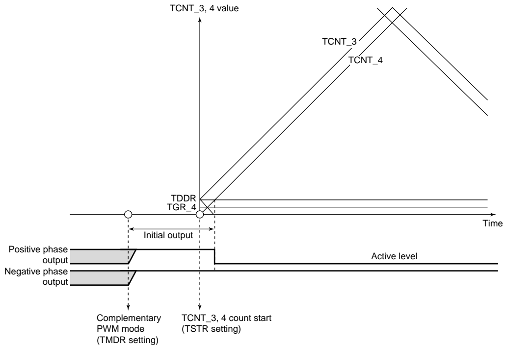
Figure 10.40 Example of Initial Output in Complementary PWM Mode (2)
