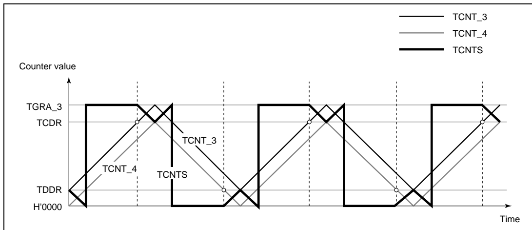
Figure 10.35 Complementary PWM Mode Counter Operation
