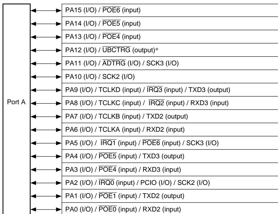
Figure 18.1 Port A (SH7046)
