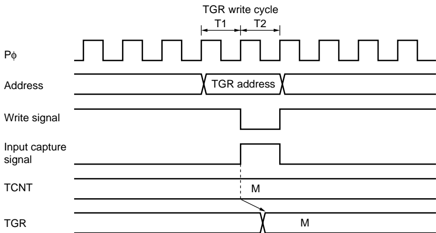
Figure 10.78 Contention between TGR Write and Input Capture
