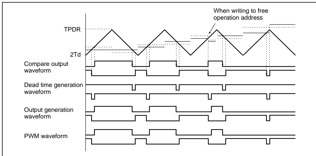
Figure 16.5 Example of PWM Waveform Generation
