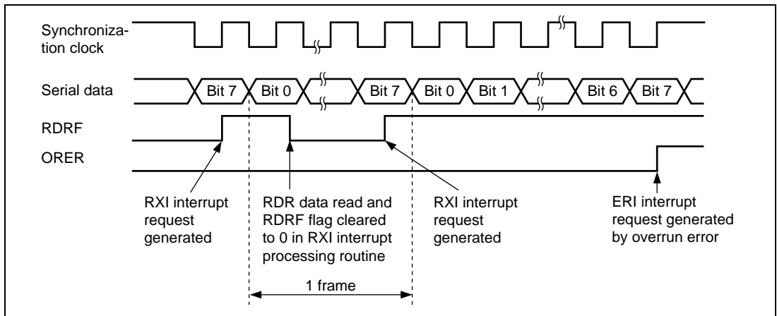
Figure 12.18 Example of SCI Operation in Reception
