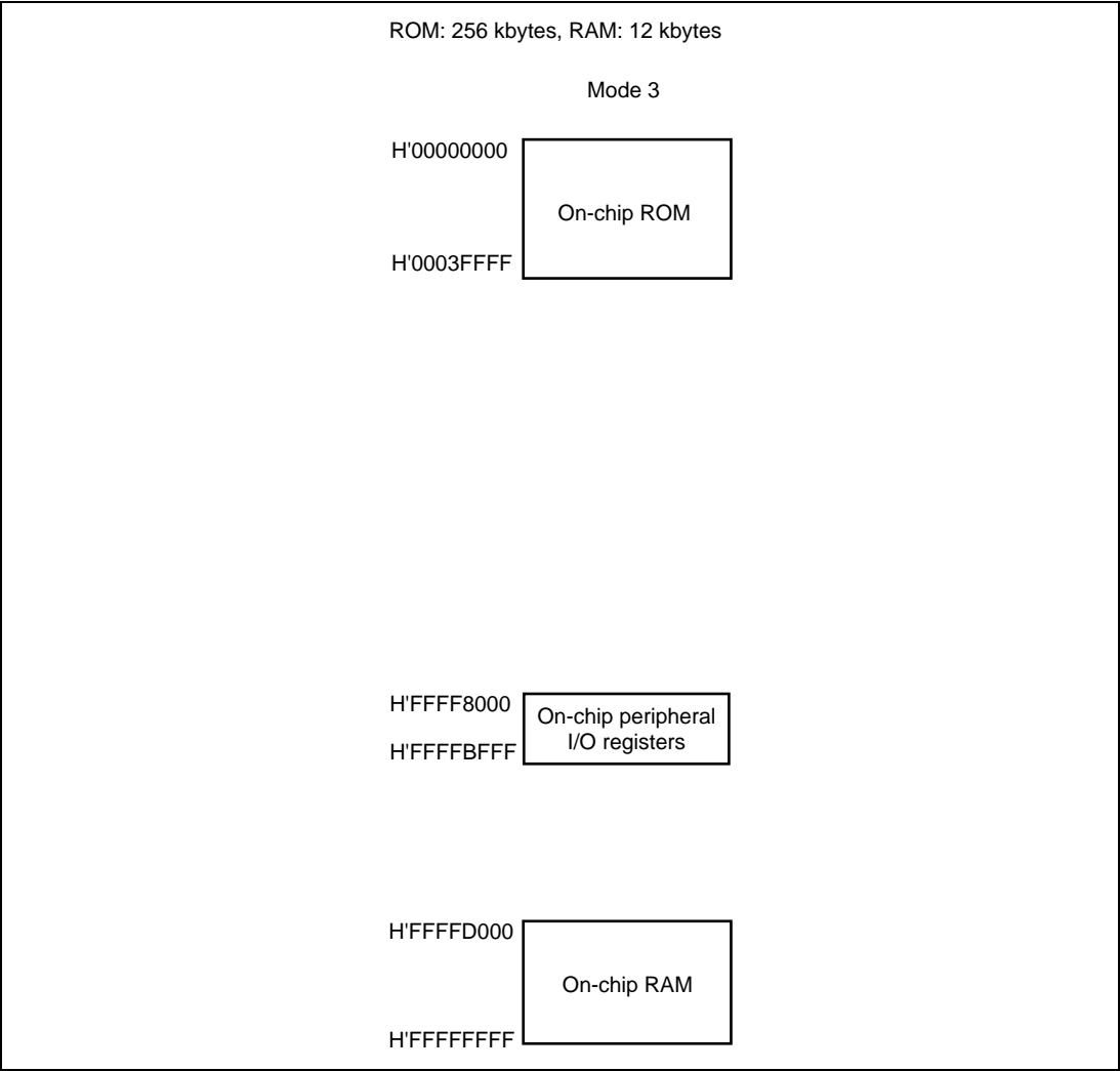
Figure 3.1 The Address Map for the Operating Mode of SH7046 Flash Memory Version
