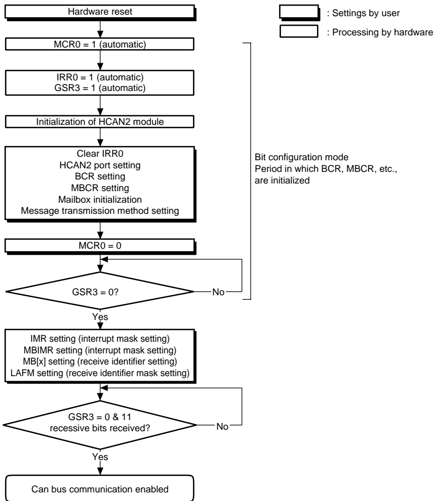
Figure 15.5 Hardware Reset Flowchart
