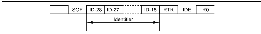
Figure 15.3 Standard Format
