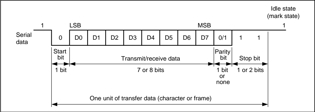
Figure 12.2 Data Format in Asynchronous Communication (Example with 8-Bit Data, Parity, Two Stop Bits)
