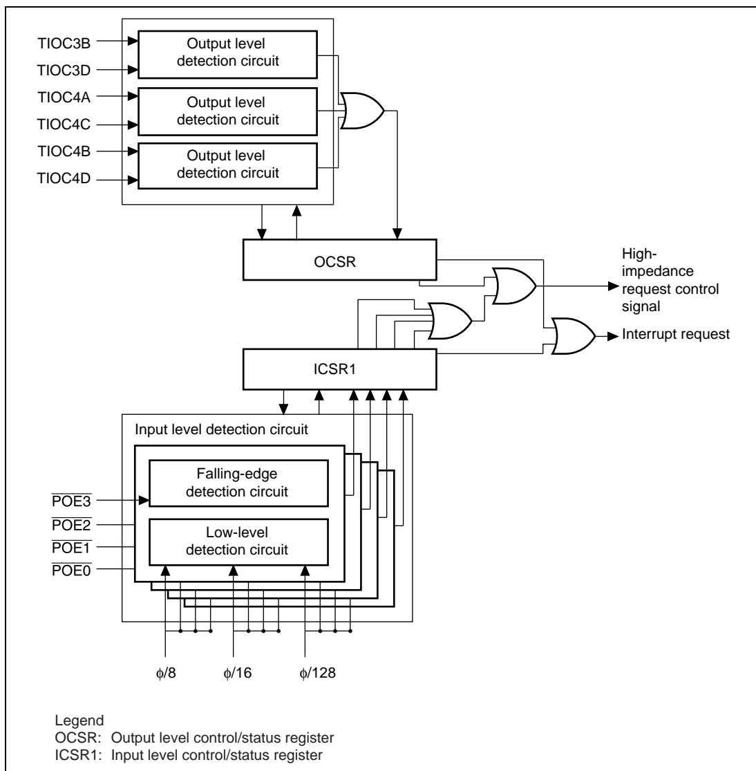
Figure 10.115 POE Block Diagram
