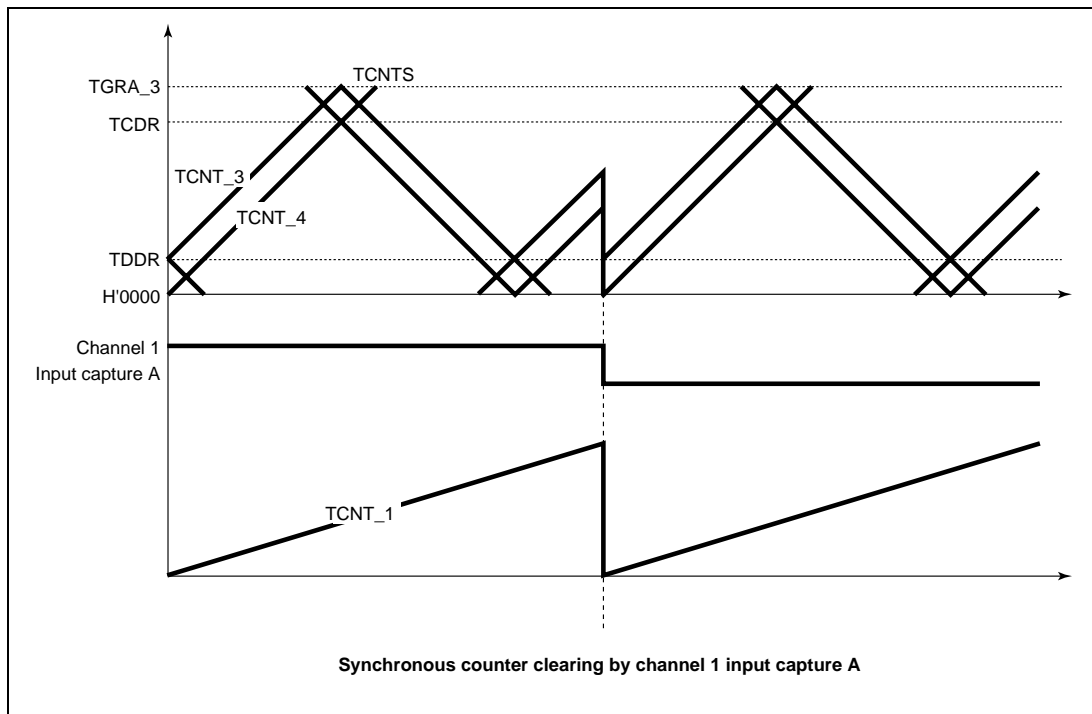
Figure 10.50 Counter Clearing Synchronized with Another Channel
