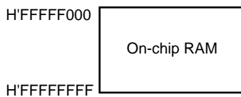
Figure 3.3 The Address Map for the Operating Mode of SH7046 Mask ROM Version
