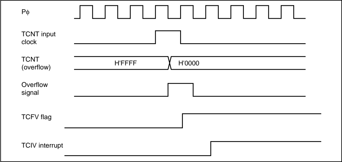
Figure 10.67 TCIV Interrupt Setting Timing
