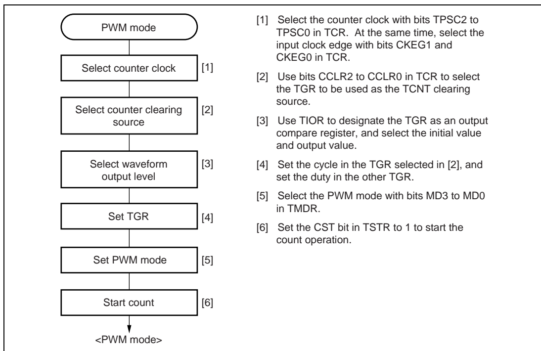
Figure 10.21 Example of PWM Mode Setting Procedure
