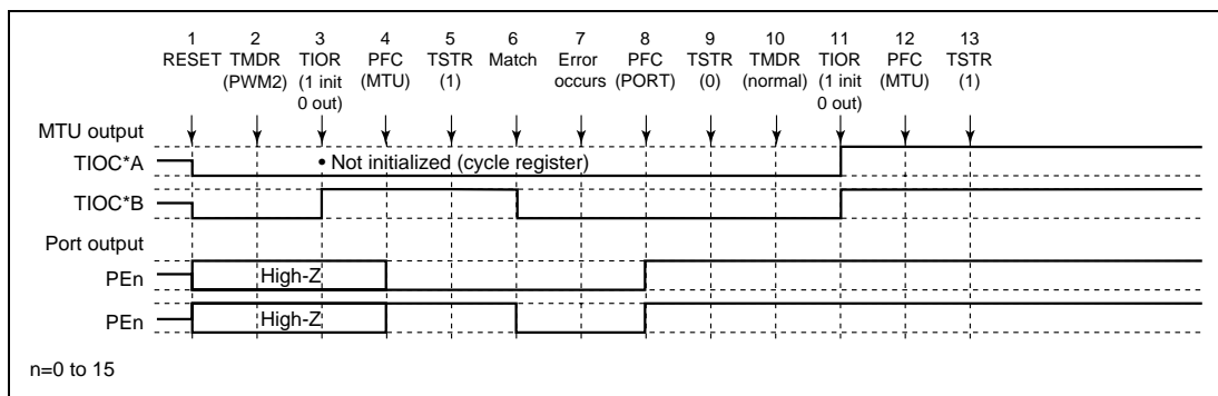
Figure 10.98 Error Occurrence in PWM Mode 2, Recovery in Normal Mode
