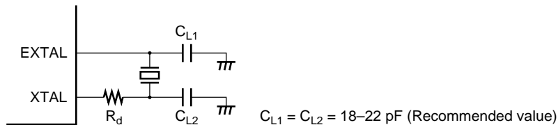
Figure 4.2 Connection of the Crystal Oscillator (Example)
