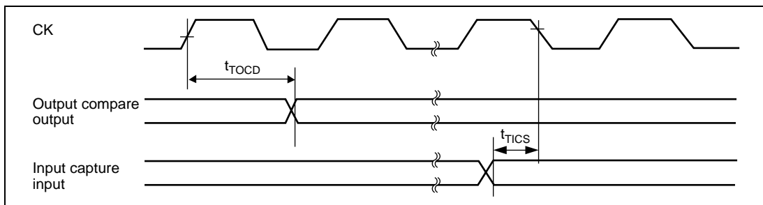
Figure 25.13 MPU Input/Output timing
