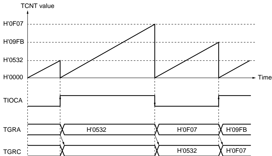
Figure 10.17 Example of Buffer Operation (2)
