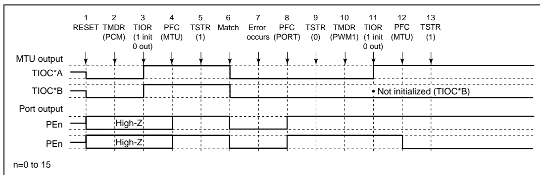
Figure 10.103 Error Occurrence in Phase Counting Mode, Recovery in PWM Mode 1
