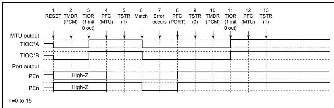
Figure 10.105 Error Occurrence in Phase Counting Mode, Recovery in Phase Counting Mode
