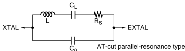
Figure 4.3 Crystal Oscillator Equivalent Circuit
