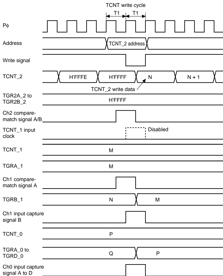
Figure 10.80 TCNT_2 Write and Overflow/Underflow Contention with Cascade Connection
