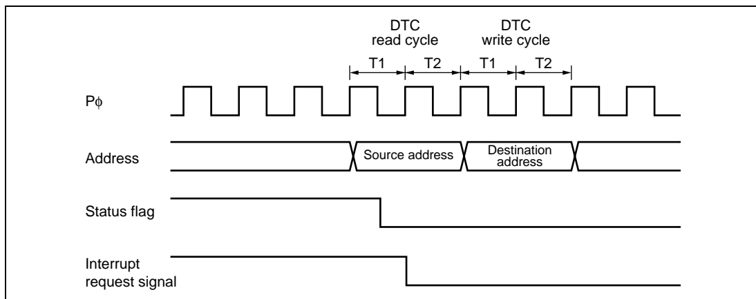
Figure 10.70 Timing for Status Flag Clearing by DTC Activation
