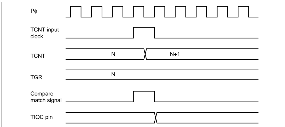
Figure 10.58 Output Compare Output Timing (Normal Mode/PWM Mode)
