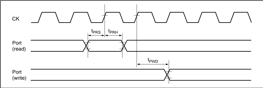
Figure 25.15 I/O Port Input/Output timing
