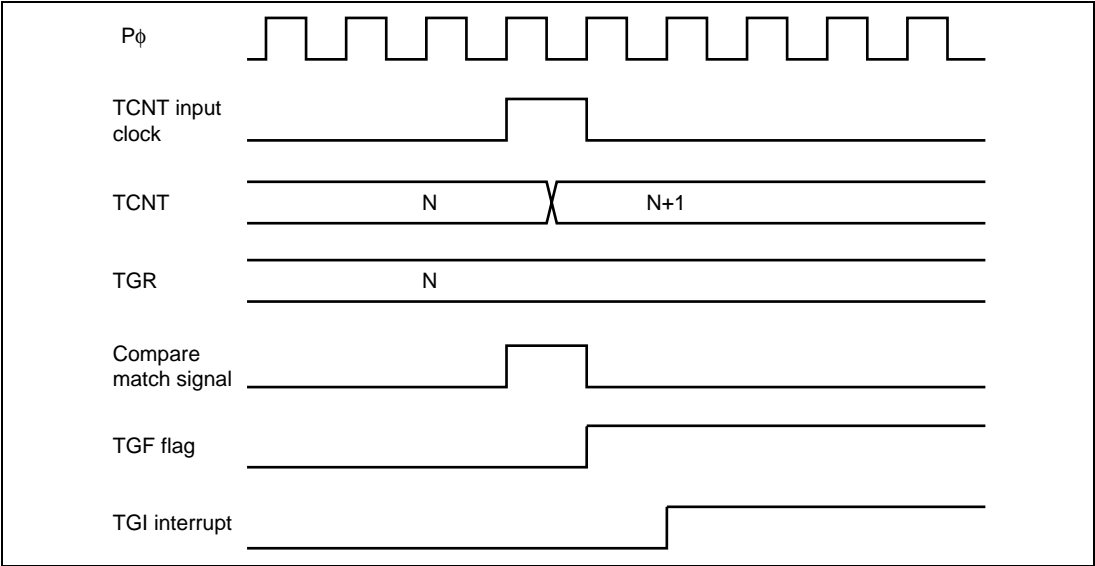
Figure 10.65 TGI Interrupt Timing (Compare Match)
