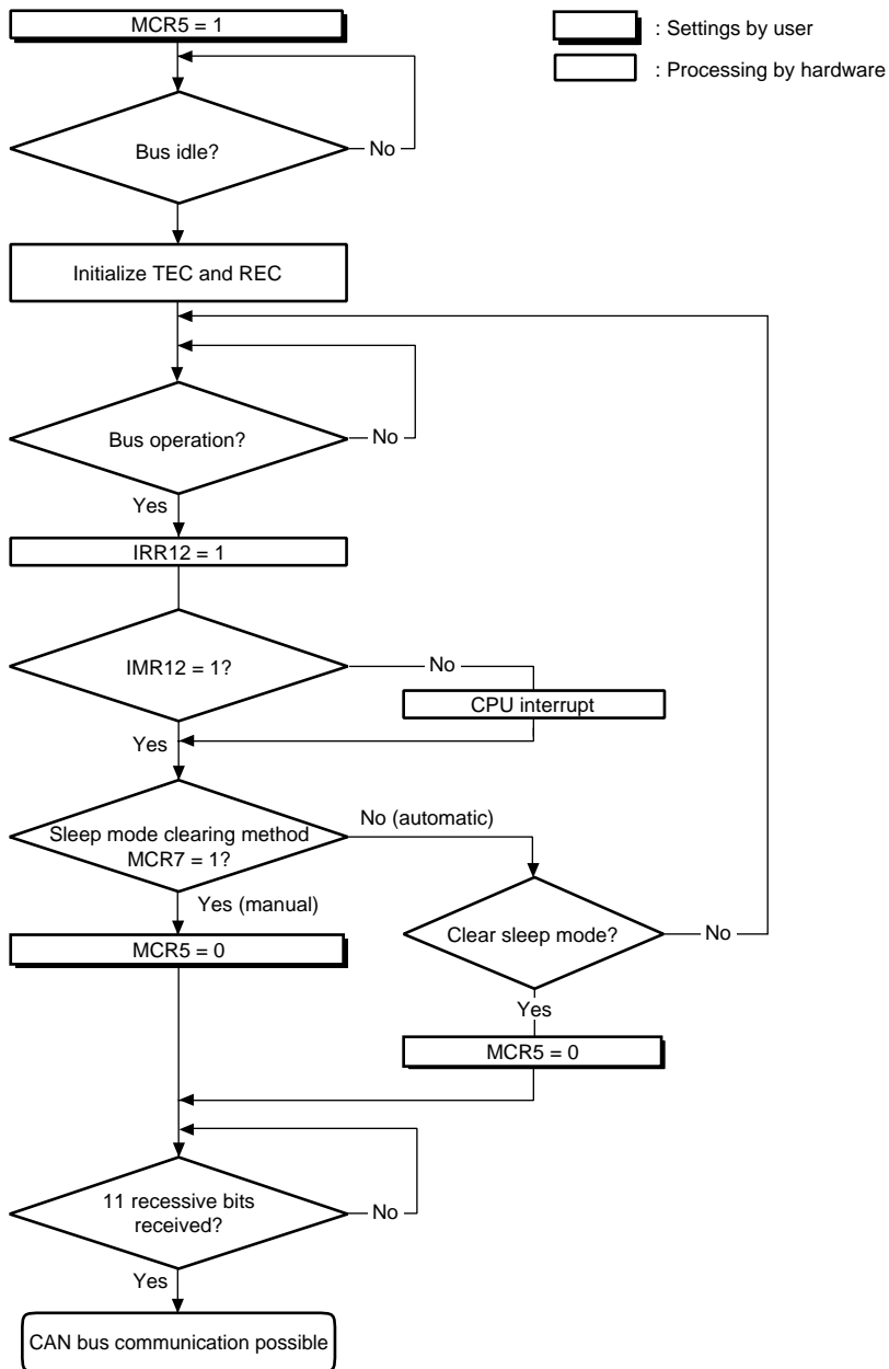
Figure 15.12 HCAN Sleep Mode Flowchart
