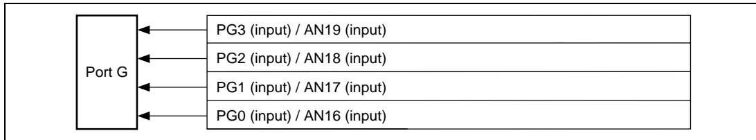
Figure 18.10 Port G (SH7046)
