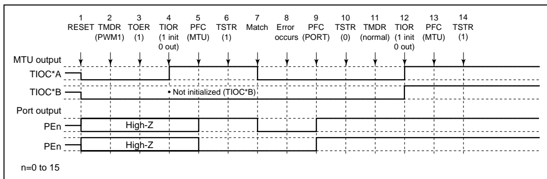
Figure 10.92 Error Occurrence in PWM Mode 1, Recovery in Normal Mode
