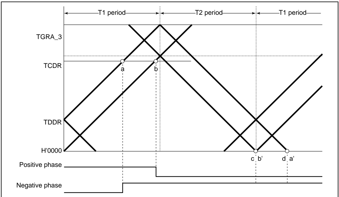
Figure 10.47 Example of Complementary PWM Mode 0% and 100% Waveform Output (4)
