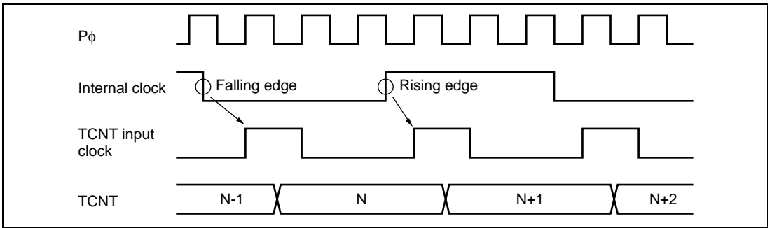
Figure 10.55 Count Timing in Internal Clock Operation
