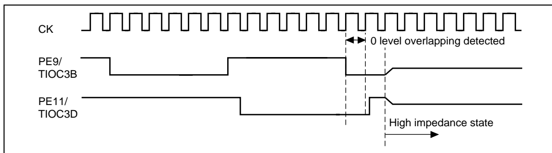
Figure 10.117 Output-Level Detection Operation
