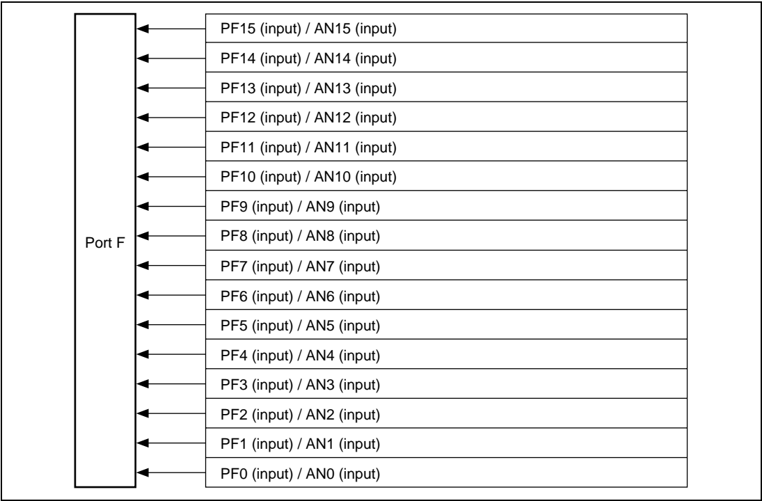
Figure 18.9 Port F (SH7047)
