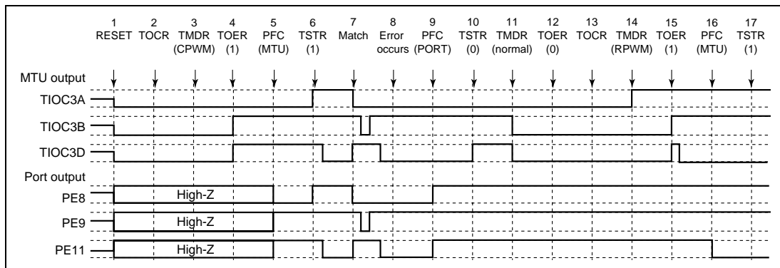
Figure 10.110 Error Occurrence in Complementary PWM Mode, Recovery in Reset-Synchronous PWM Mode
