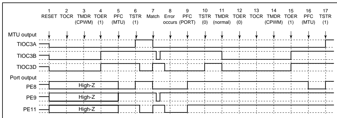
Figure 10.109 Error Occurrence in Complementary PWM Mode, Recovery in Complementary PWM Mode
