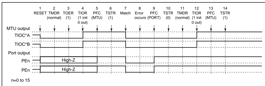
Figure 10.86 Error Occurrence in Normal Mode, Recovery in Normal Mode
