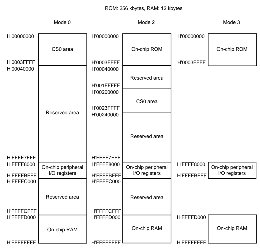
Figure 3.2 The Address Map for the Operating Modes of SH7047 Flash Memory Version
