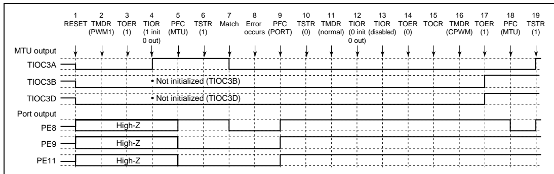
Figure 10.96 Error Occurrence in PWM Mode 1, Recovery in Complementary PWM Mode
