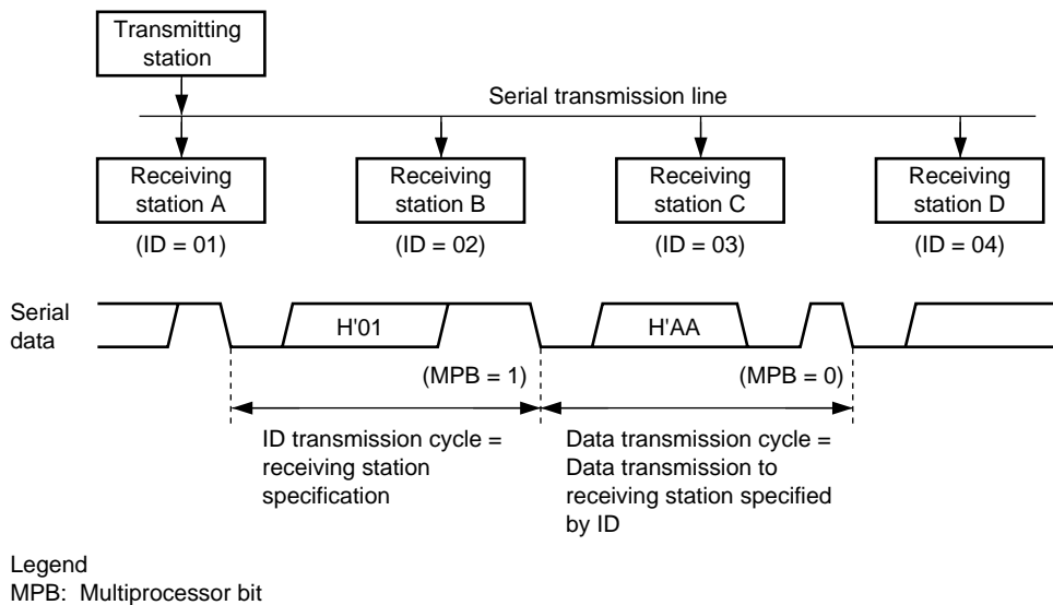
Figure 12.10 Example of Communication Using Multiprocessor Format (Transmission of Data H'AA to Receiving Station A)
