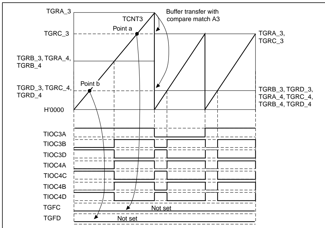
Figure 10.82 Buffer Operation and Compare-Match Flags in Reset Sync PWM Mode
