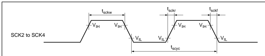
Figure 25.17 SCI Input Timing
