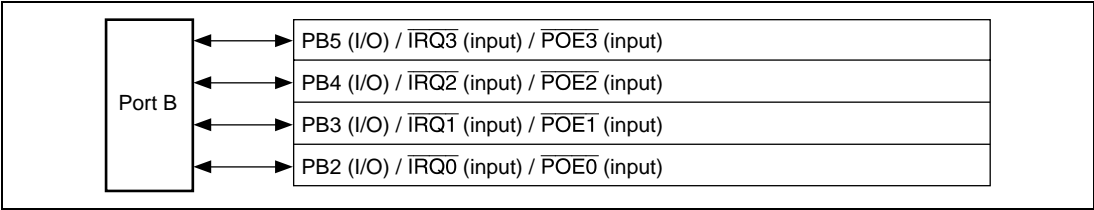
Figure 18.3 Port B (SH7046)
