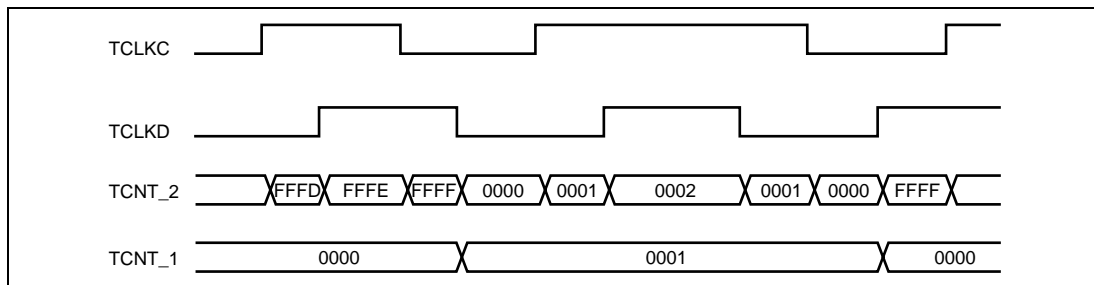
Figure 10.20 Example of Cascaded Operation (2)
