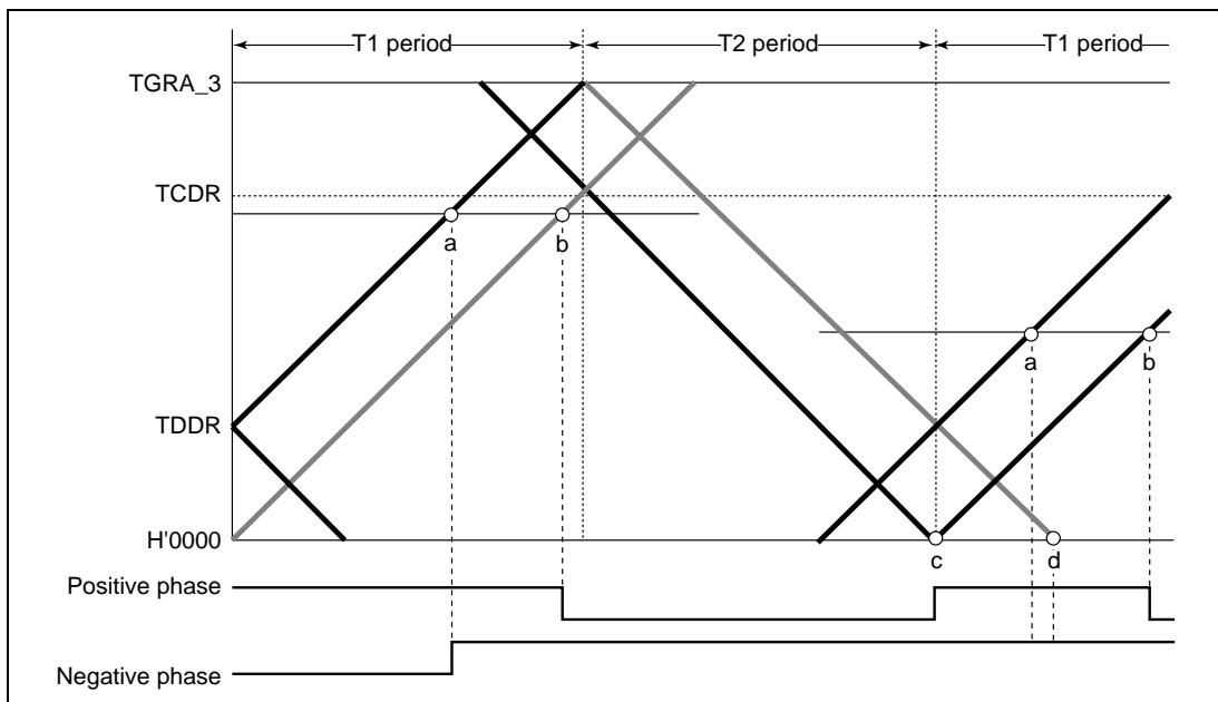
Figure 10.45 Example of Complementary PWM Mode 0% and 100% Waveform Output (2)
