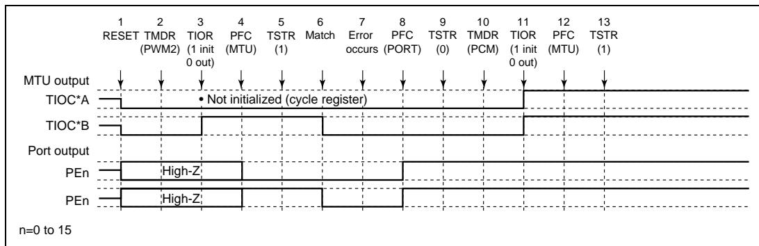
Figure 10.101 Error Occurrence in PWM Mode 2, Recovery in Phase Counting Mode
