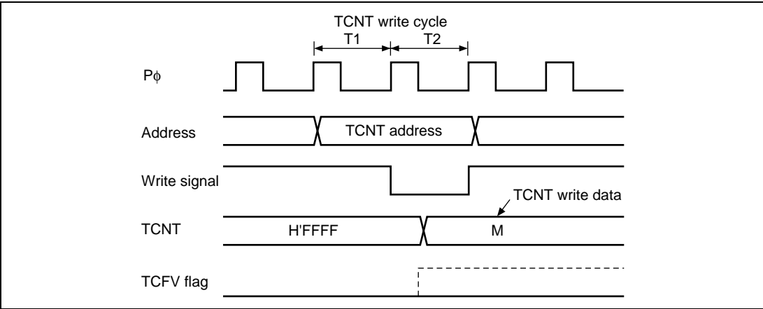
Figure 10.84 Contention between Overflow and Counter Clearing
