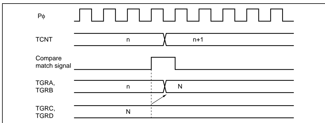
Figure 10.63 Buffer Operation Timing (Compare Match)
