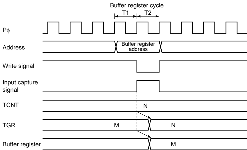
Figure 10.77 Contention between TGR Read and Input Capture
