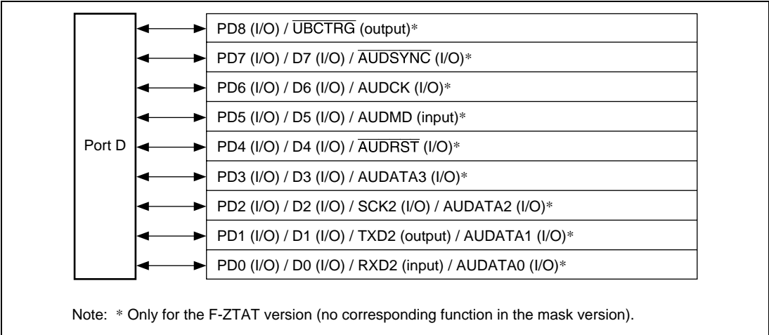
Figure 18.5 Port D (SH7047)
