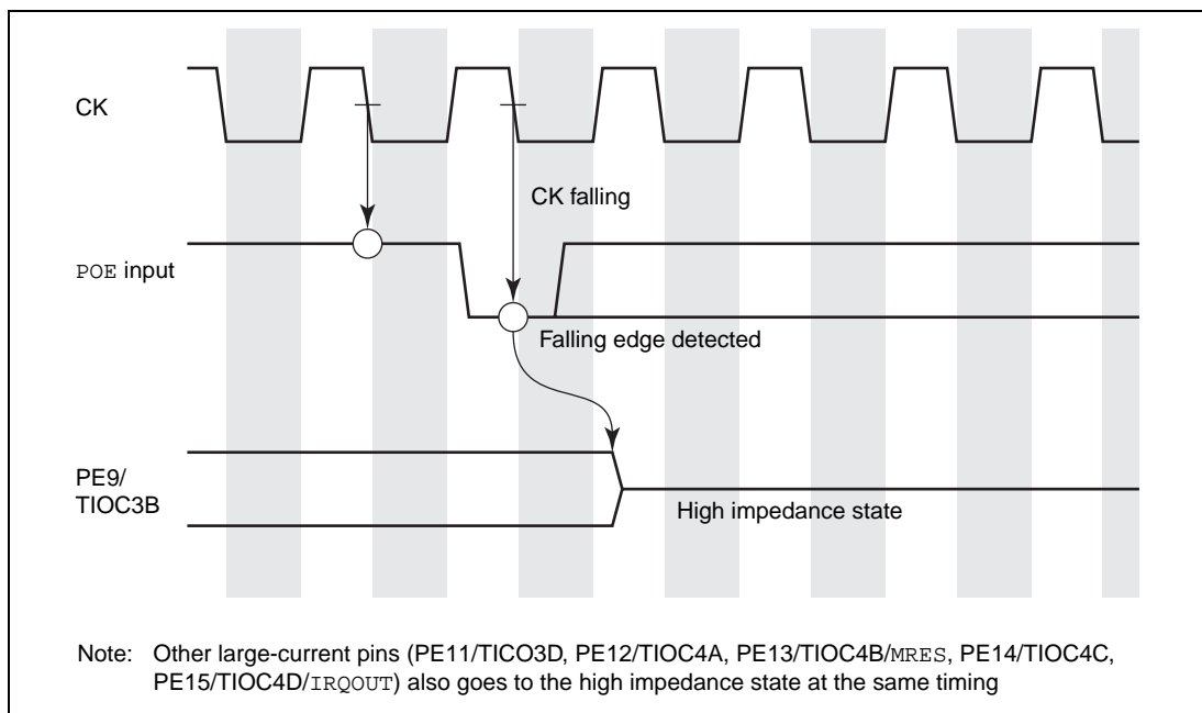
Figure 10.118 Falling Edge Detection Operation
