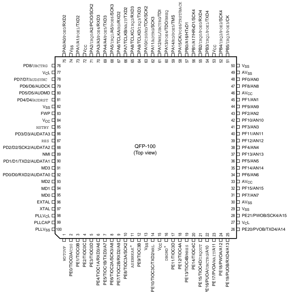
Figure1.4 SH7047 Pin Arrangement
