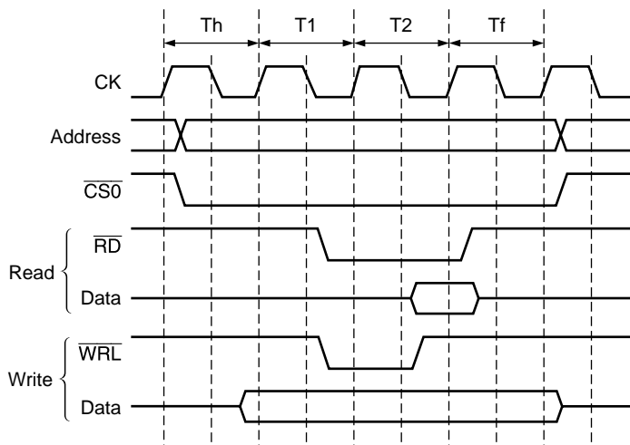
Figure 9.6 \overline{CS} Assert Period Extension Function
