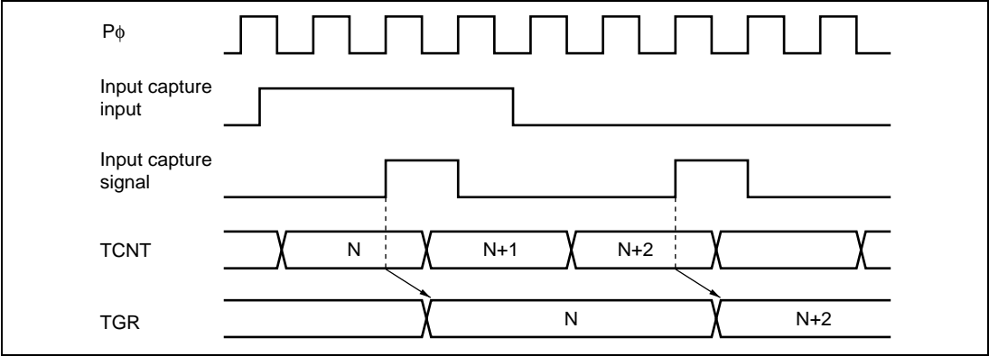
Figure 10.60 Input Capture Input Signal Timing
