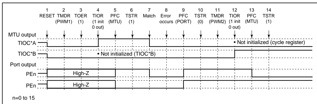
Figure 10.94 Error Occurrence in PWM Mode 1, Recovery in PWM Mode 2
