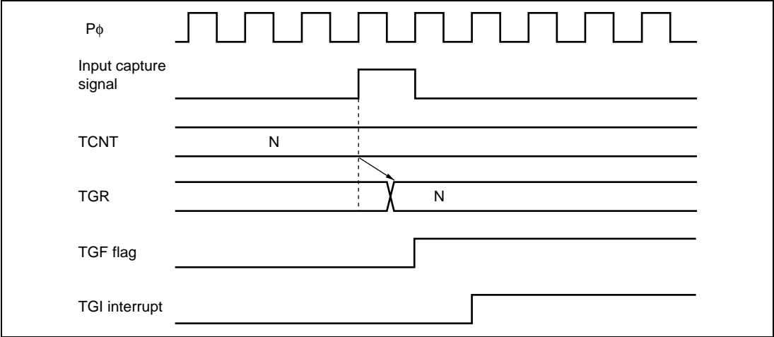
Figure 10.66 TGI Interrupt Timing (Input Capture)
