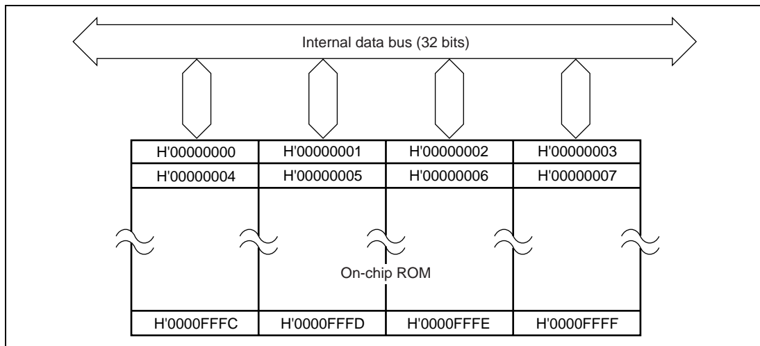
Figure 20.1 Mask ROM Block Diagram (SH7046)
