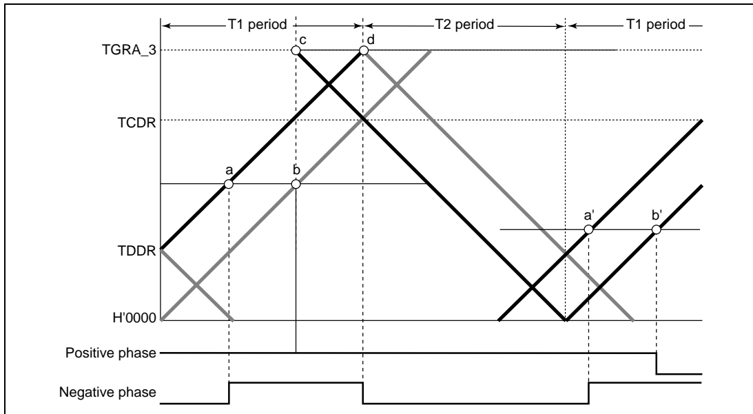
Figure 10.44 Example of Complementary PWM Mode 0% and 100% Waveform Output (1)
