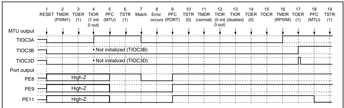
Figure 10.97 Error Occurrence in PWM Mode 1, Recovery in Reset-Synchronous PWM Mode
