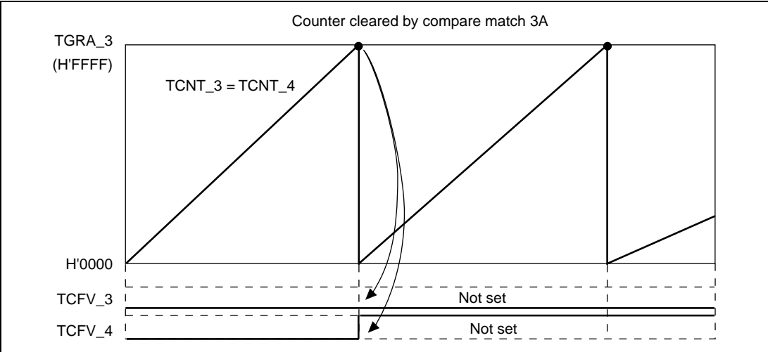
Figure 10.83 Reset Sync PWM Mode Overflow Flag
