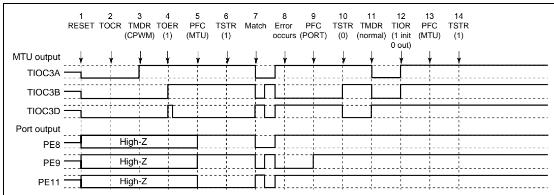
Figure 10.111 Error Occurrence in Reset-Synchronous PWM Mode, Recovery in Normal Mode
