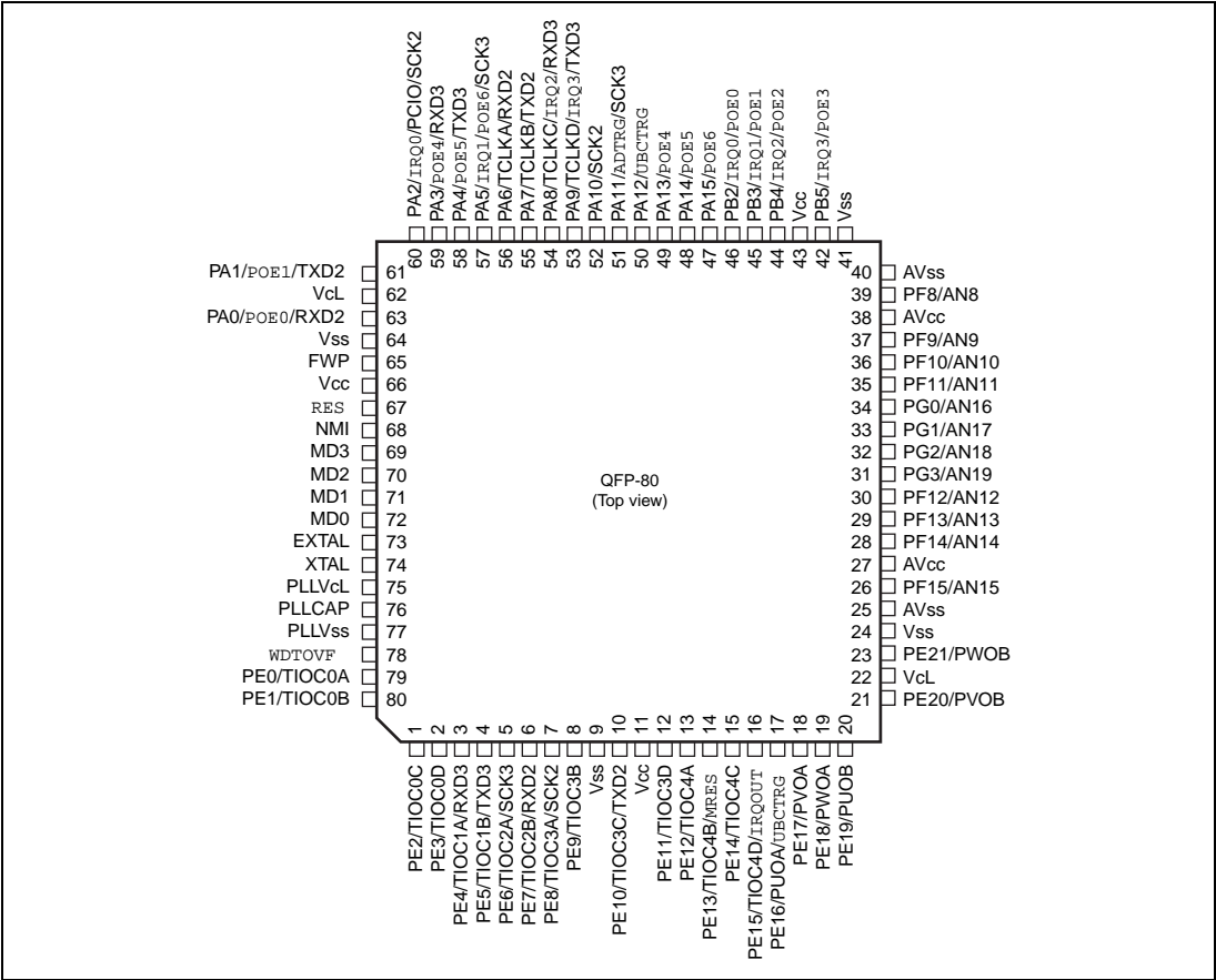
Figure1.3 SH7046 Pin Arrangement
