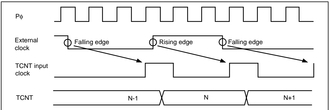
Figure 10.57 Count Timing in External Clock Operation (Phase Counting Mode)
