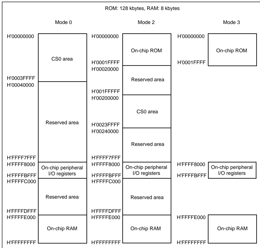
Figure 3.4 The Address Map for the Operating Modes of SH7047 Mask ROM Version
