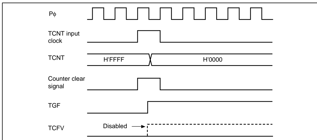
Figure 10.85 Contention between TCNT Write and Overflow
