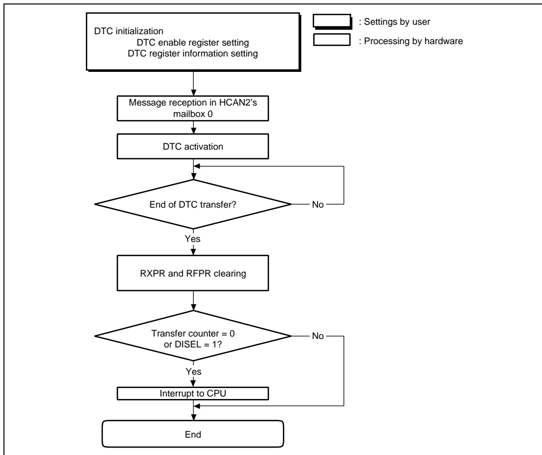
Figure 15.14 DTC Transfer Flowchart
