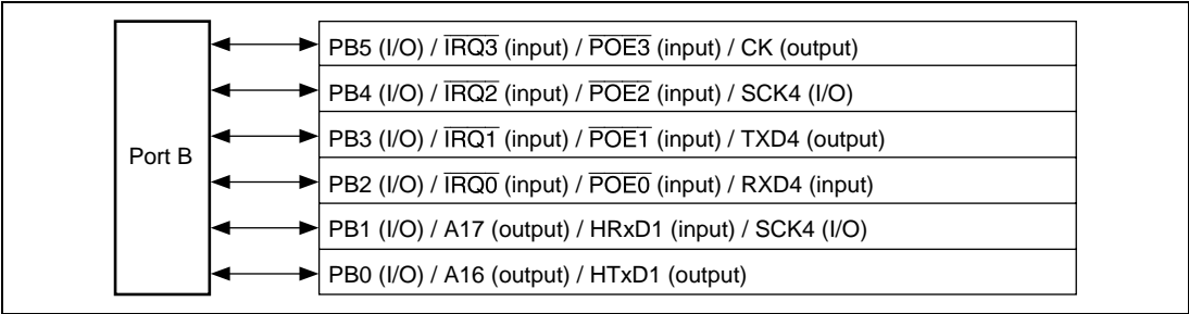
Figure 18.4 Port B (SH7047)
