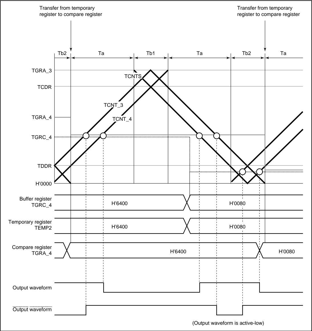
Figure 10.36 Example of Complementary PWM Mode Operation
