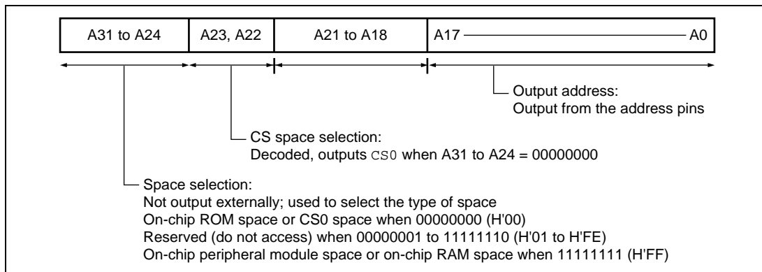
Figure 9.2 Address Format
