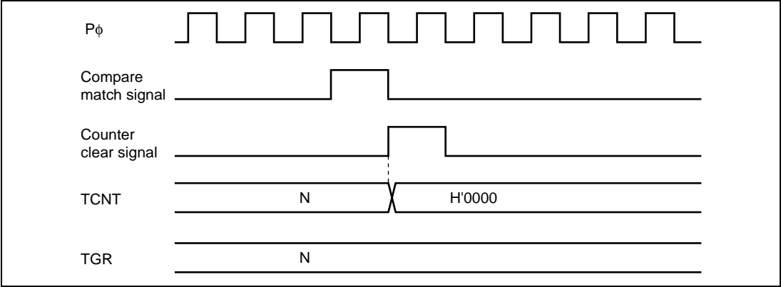
Figure 10.61 Counter Clear Timing (Compare Match)
