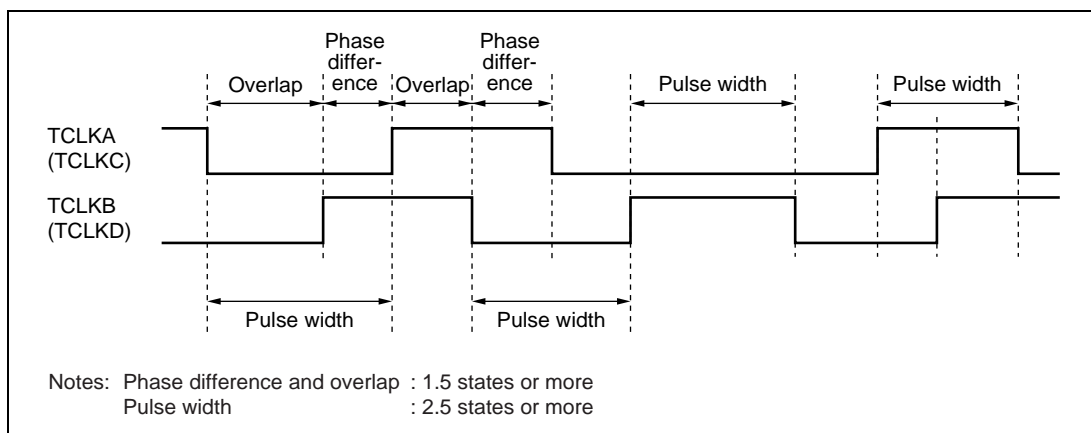
Figure 10.71 Phase Difference, Overlap, and Pulse Width in Phase Counting Mode
