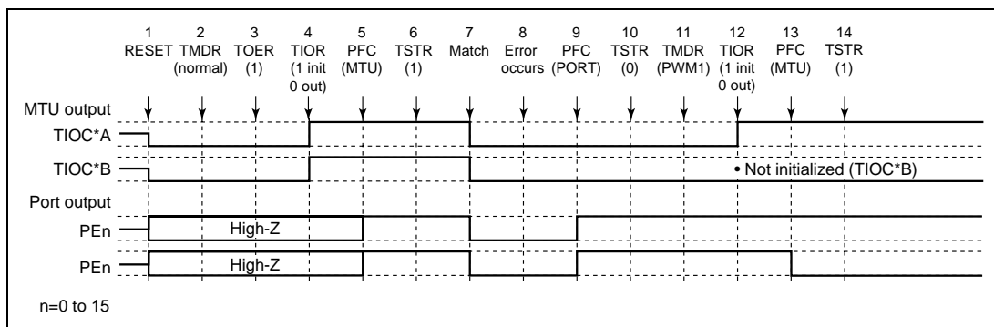
Figure 10.87 Error Occurrence in Normal Mode, Recovery in PWM Mode 1
