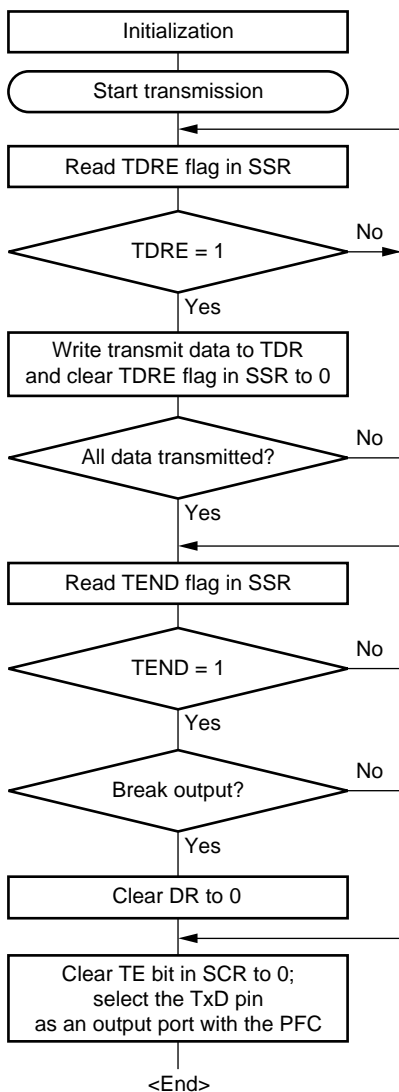
Figure 12.7 Sample Serial Transmission Flowchart
