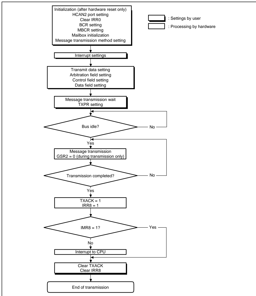
Figure 15.8 Transmission Flowchart
