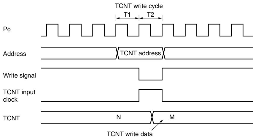
Figure 10.73 Contention between TCNT Write and Increment Operations
