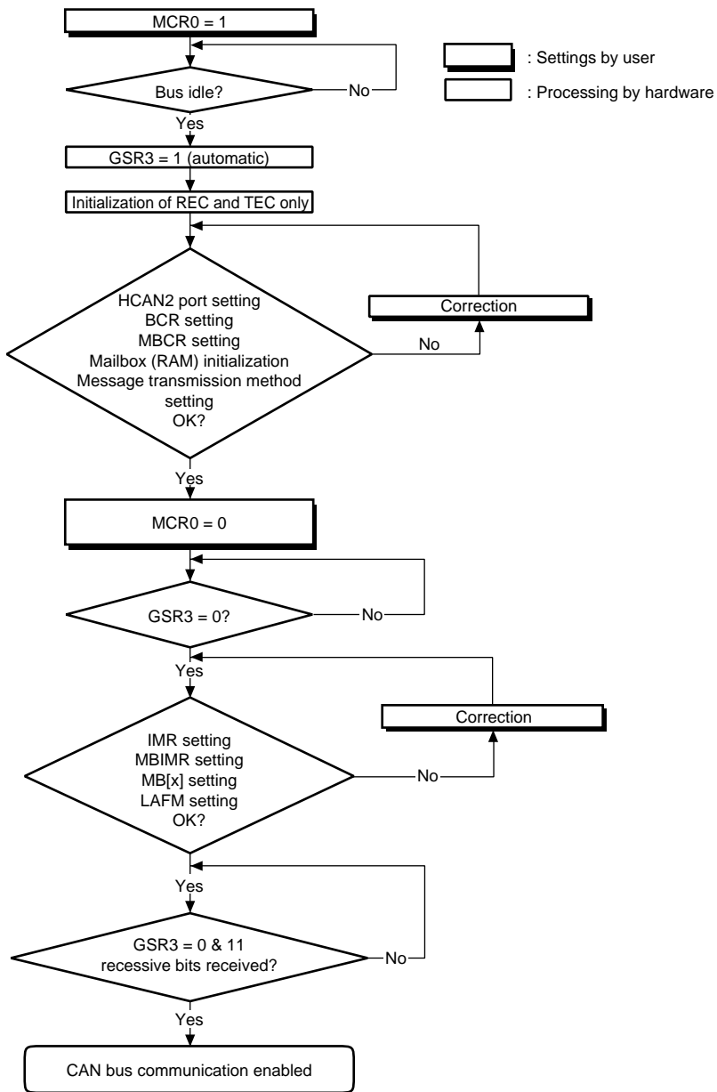
Figure 15.6 Software Reset Flowchart
