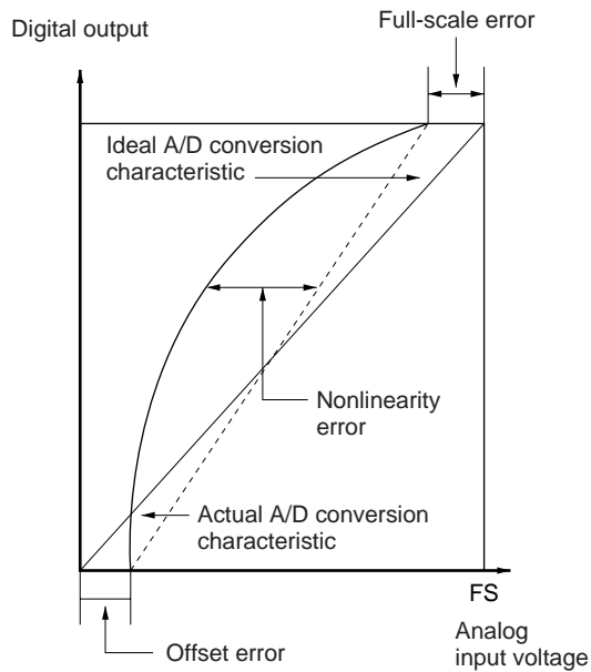
Figure 13.5 A/D Conversion Precision Definitions
