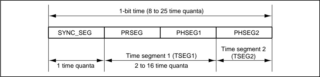
Figure 15.7 Detailed Description of 1-Bit Timer
