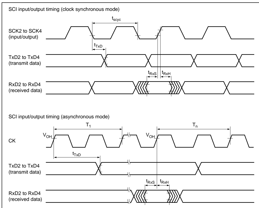
Figure 25.18 SCI Input/Output Timing
