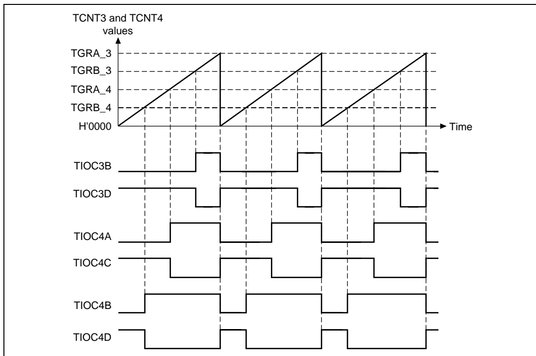
Figure 10.32 Reset-Synchronized PWM Mode Operation Example (When the TOCR's OLSN = 1 and OLSP = 1)
