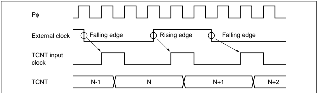
Figure 10.56 Count Timing in External Clock Operation
