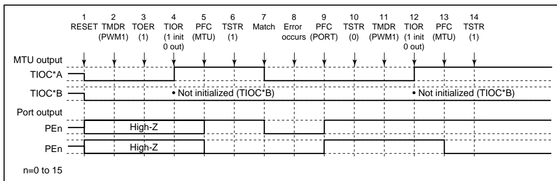
Figure 10.93 Error Occurrence in PWM Mode 1, Recovery in PWM Mode 1
