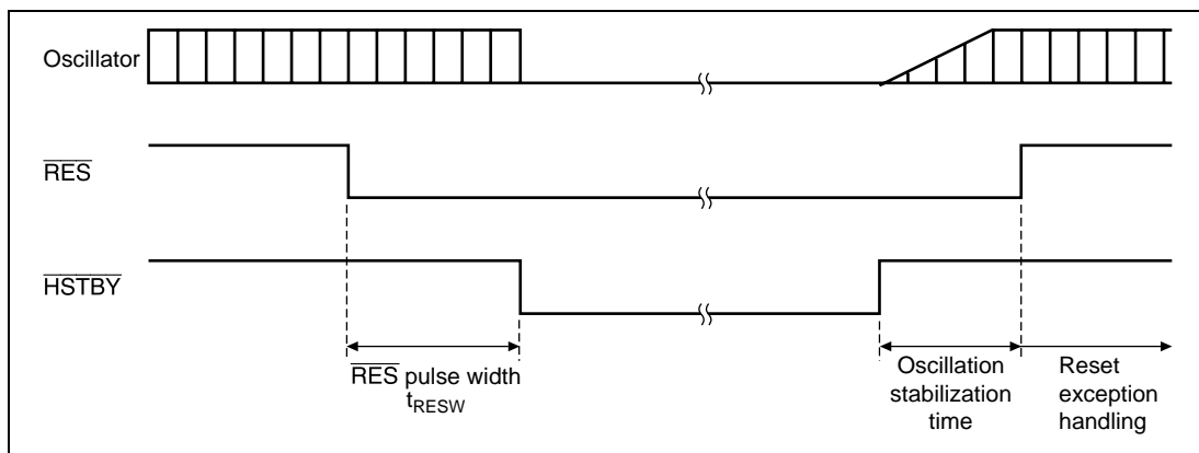
Figure 24.3 Transition Timing to Hardware Standby Mode
