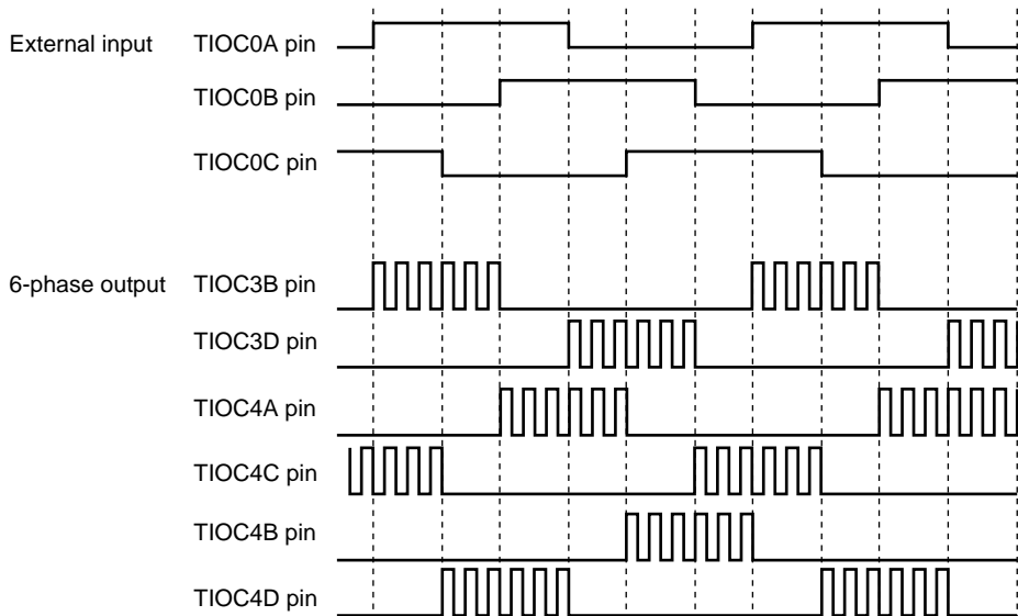
Figure 10.51 Example of Output Phase Switching by External Input (1)
