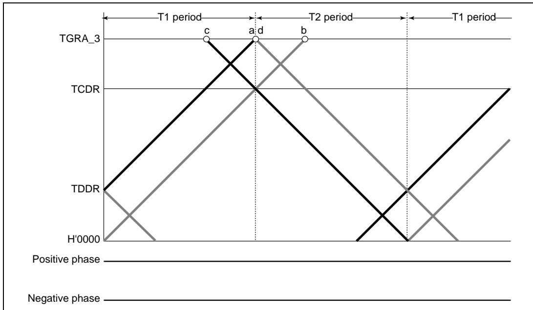
Figure 10.48 Example of Complementary PWM Mode 0% and 100% Waveform Output (5)
