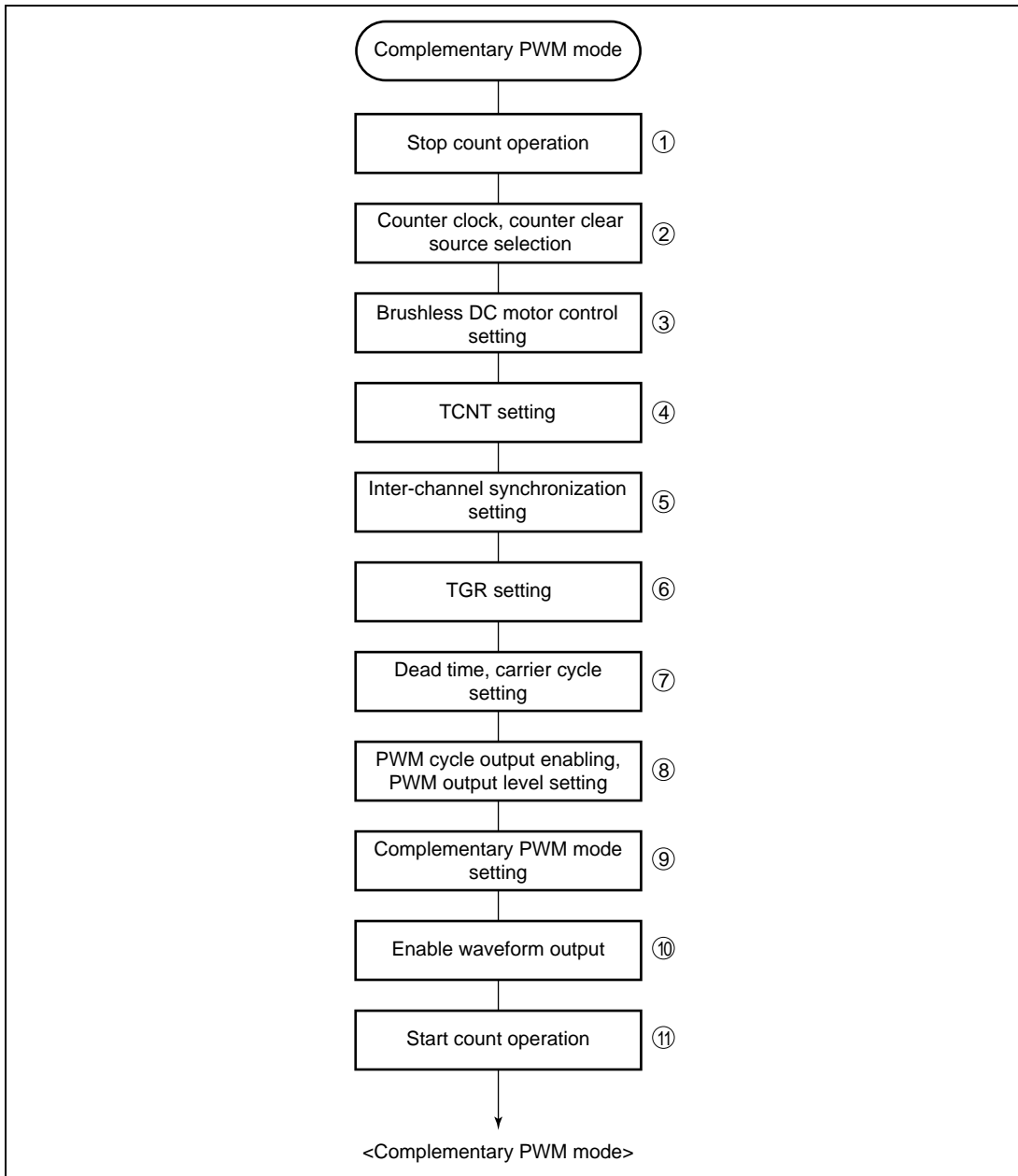
Figure 10.34 Example of Complementary PWM Mode Setting Procedure
