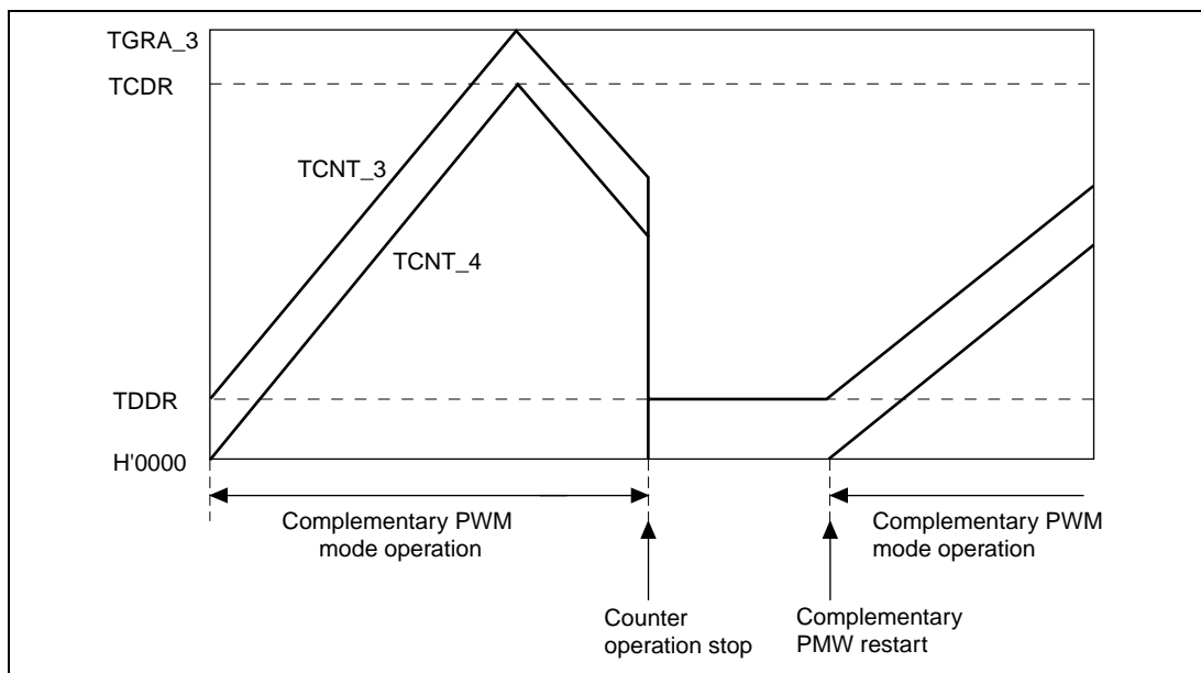
Figure 10.81 Counter Value during Complementary PWM Mode Stop
