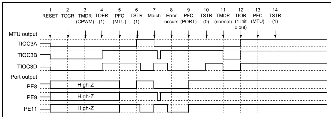
Figure 10.106 Error Occurrence in Complementary PWM Mode, Recovery in Normal Mode
