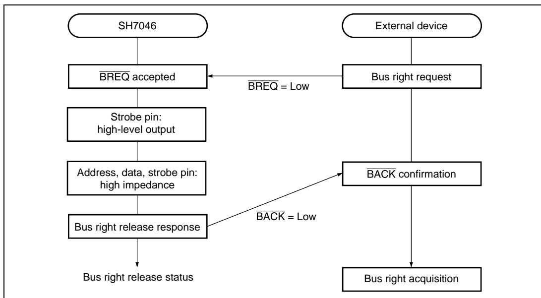
Figure 9.8 Bus Right Release Procedure
