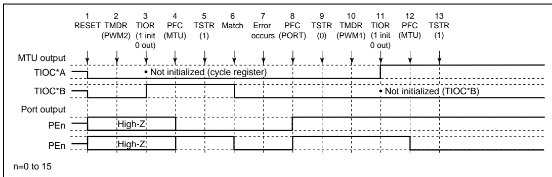
Figure 10.99 Error Occurrence in PWM Mode 2, Recovery in PWM Mode 1
