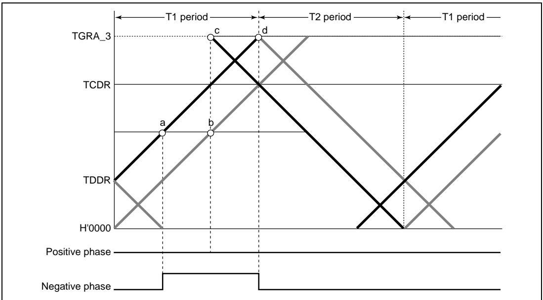
Figure 10.46 Example of Complementary PWM Mode 0% and 100% Waveform Output (3)
