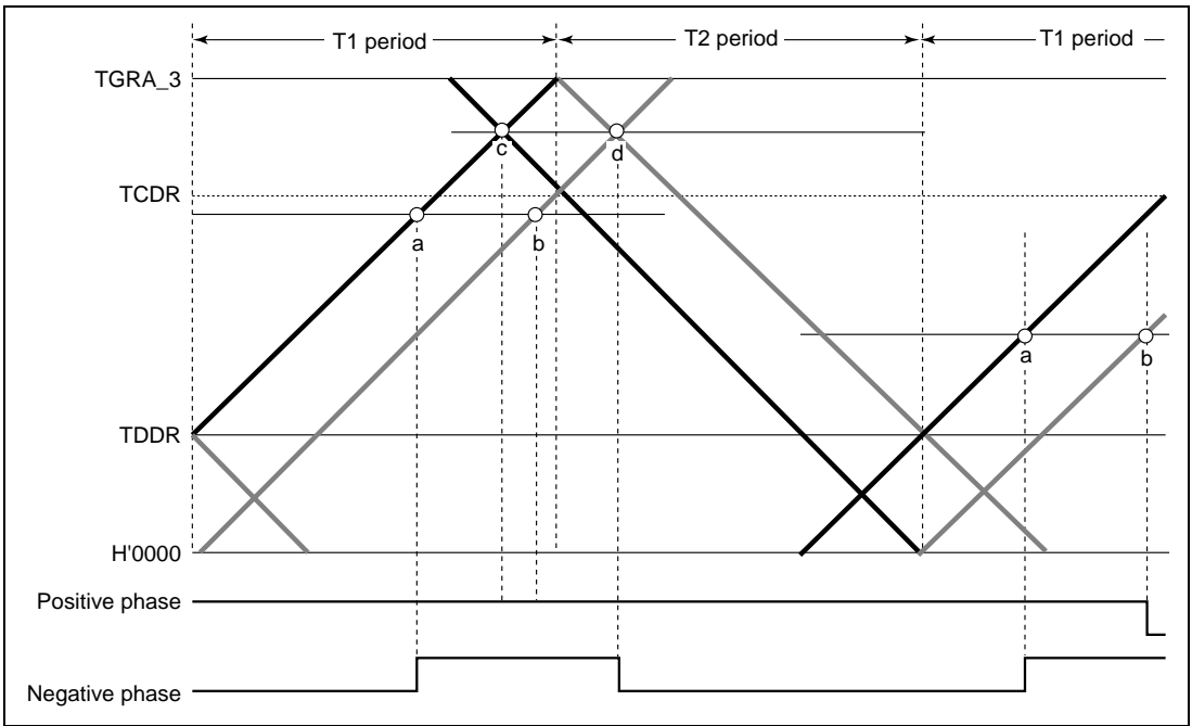
Figure 10.42 Example of Complementary PWM Mode Waveform Output (2)
