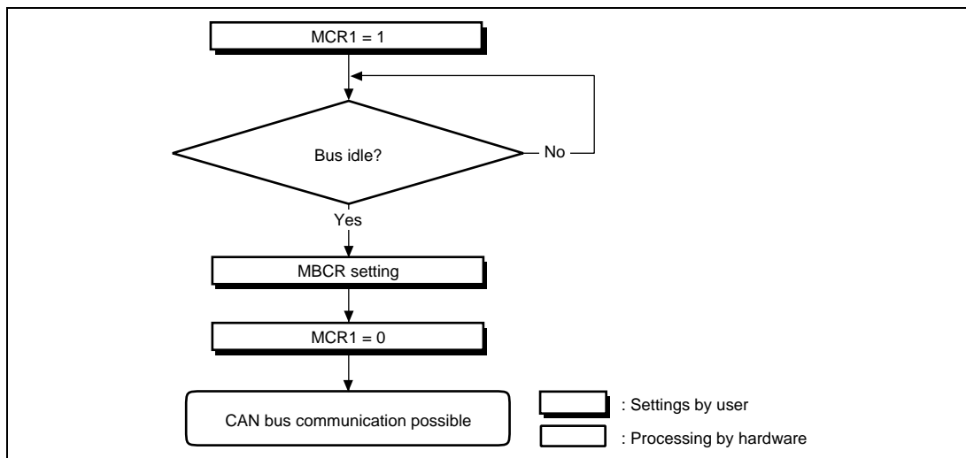
Figure 15.13 HCAN2 Halt Mode Flowchart
