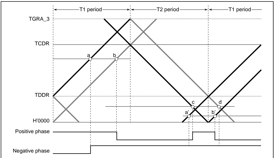
Figure 10.43 Example of Complementary PWM Mode Waveform Output (3)
