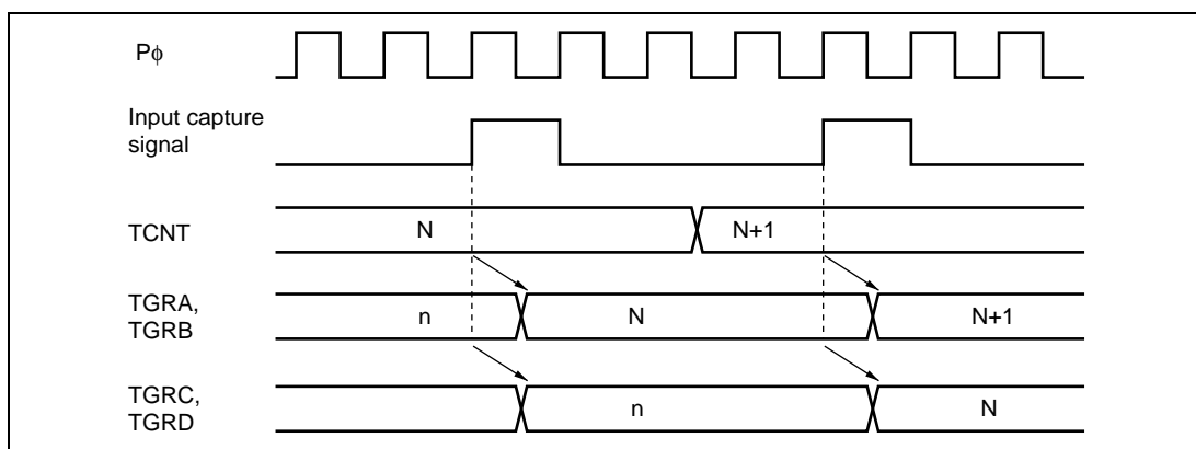
Figure 10.64 Buffer Operation Timing (Input Capture)
