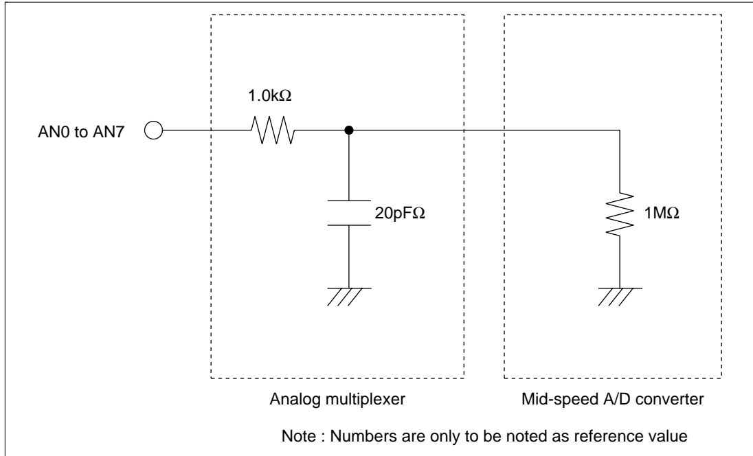
Figure 16.9 Equivalent Circuit for the Analog Input Pins
