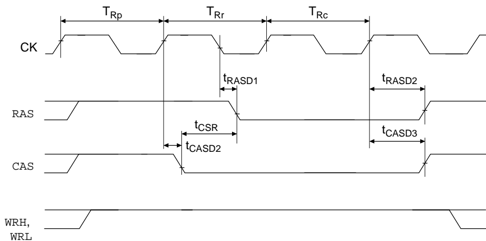
Figure 19.16 CAS-before-RAS Refresh (Short Pitch)
