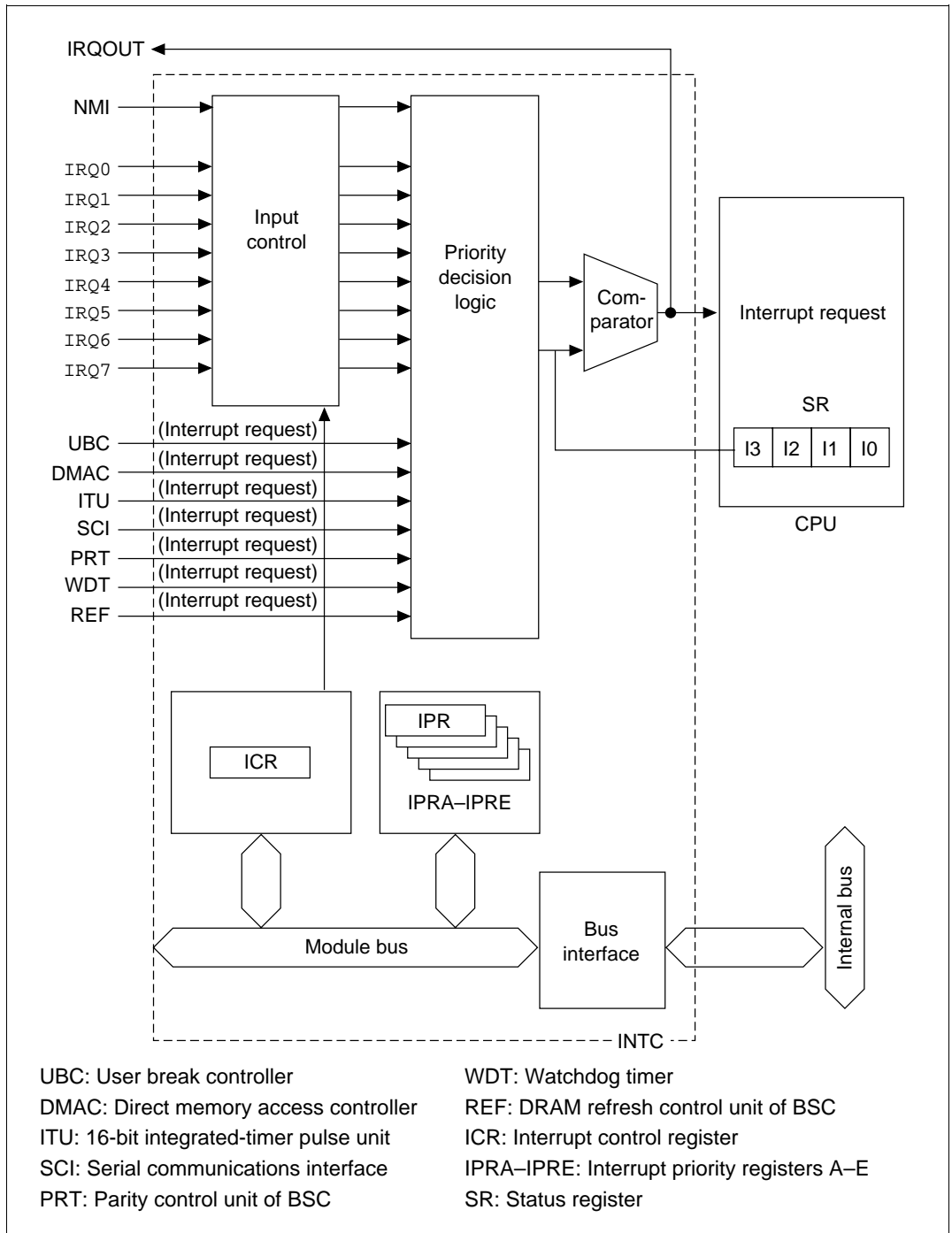
Figure 5.1 Block Diagram of the Interrupt Controller
