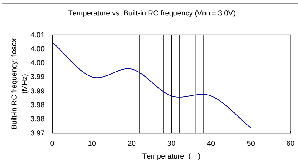
Temperature vs. Built-in RC fosc ( V_{DD} = 3.0V )
