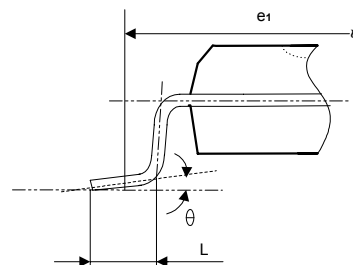
Detail F
