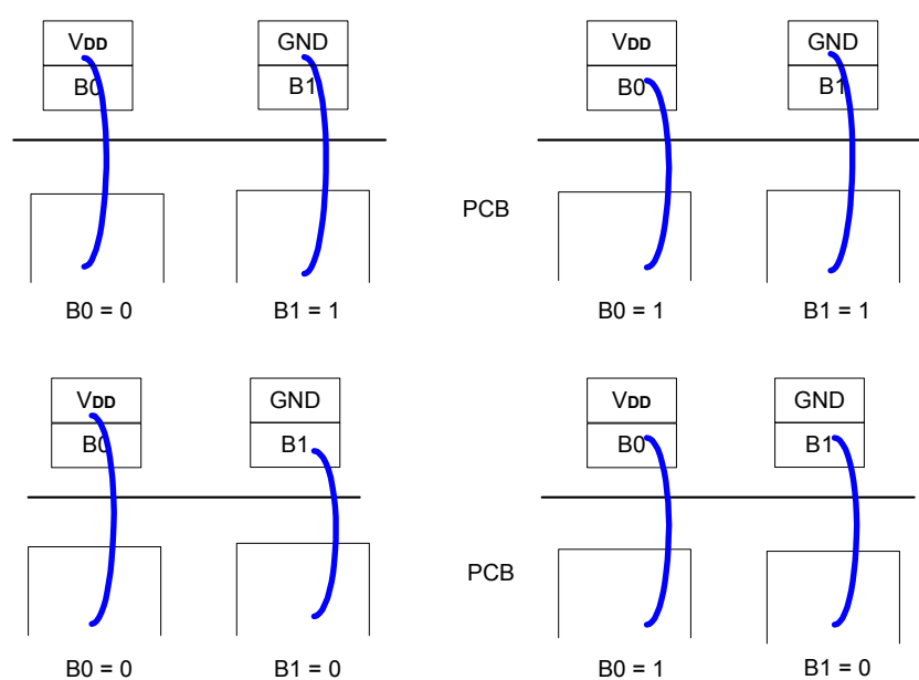
SH66L10A Bonding Option
