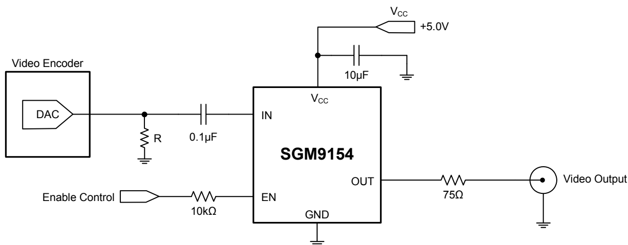
Figure 2. AC-Coupled Input and DC-Coupled Output Application Circuit
