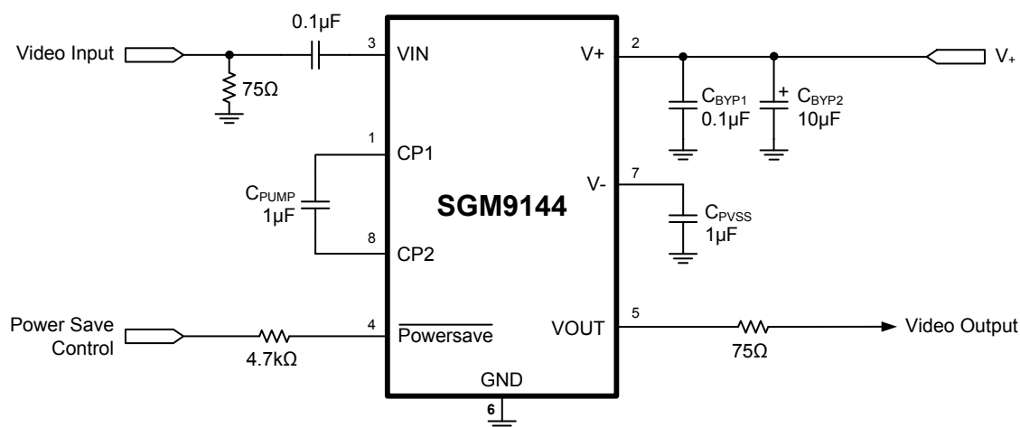
Figure 1. Standard Circuit
