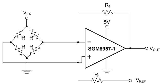
Figure 4. Bridge Amplifier Configuration
