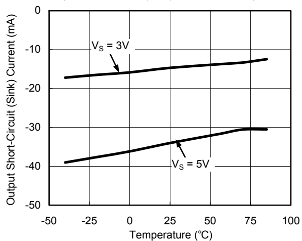
Output Short-Circuit (Sink) Current vs. Temperature
