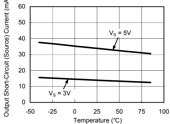
Output Short-Circuit (Source) Current vs. Temperature
