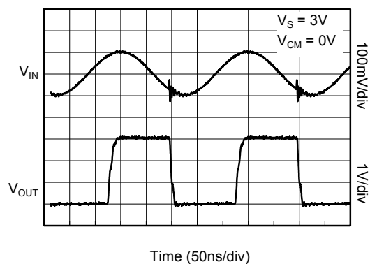
Sinusoid Response at 4MHz
