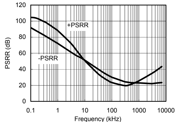
PSRR vs. Frequency at \pm 1.25\text{V}
