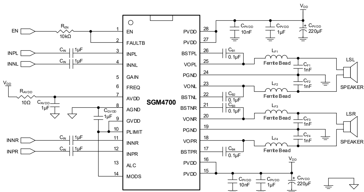
Figure 16. Differential Inputs in Non-ALC Mode with DSM
