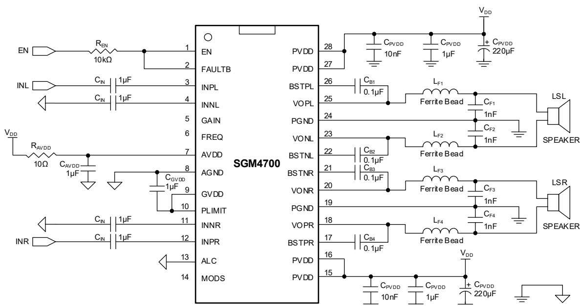
Figure 17. Single-Ended Inputs in ALC-1 Mode with SSM
