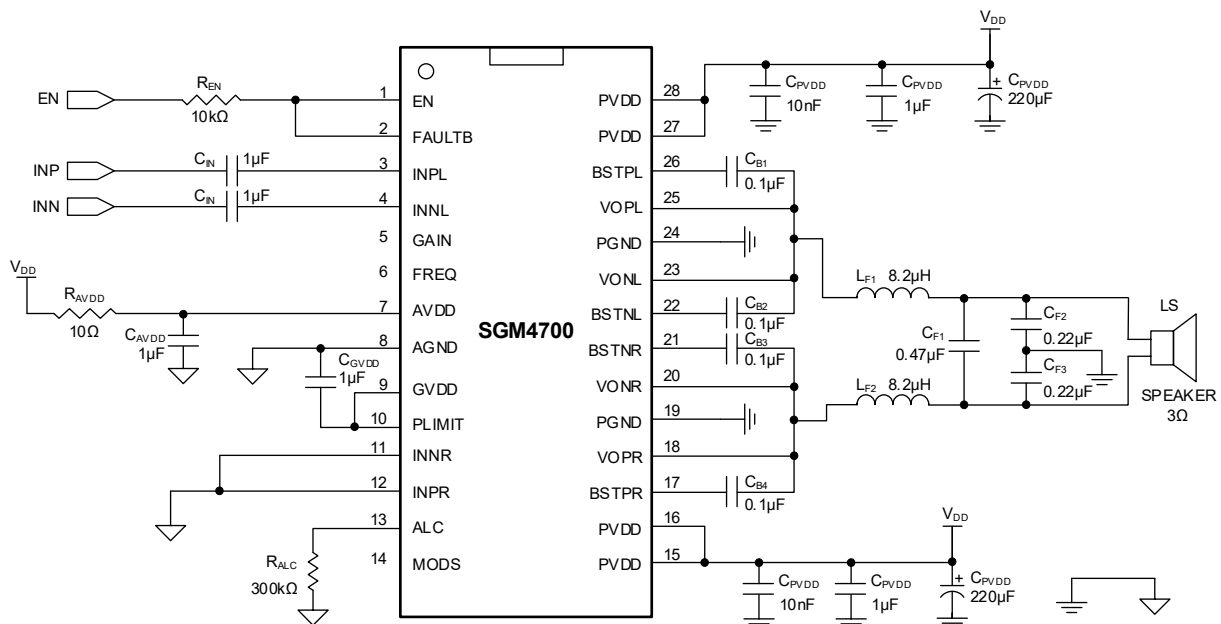
Figure 19. Differential Inputs in ALC-3 Mode with SSM in PBTL Configuration
