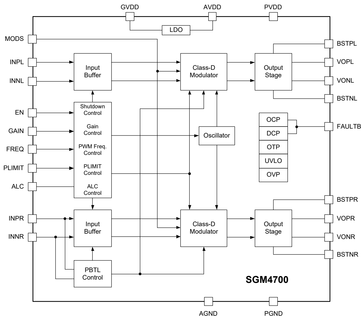
Figure 3. Block Diagram
