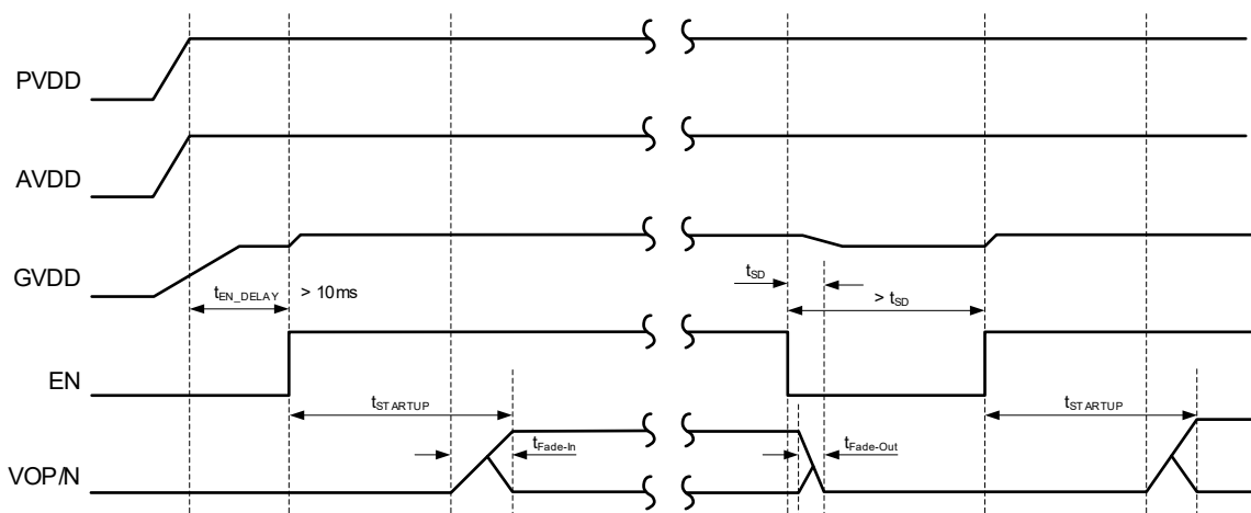
Figure 12. Startup Timing
