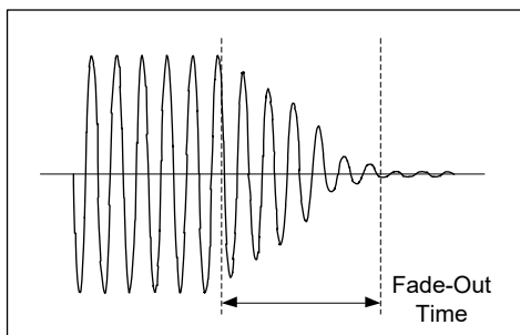
Figure 10. Fade-Out Waveform
