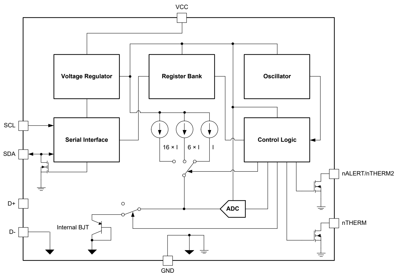
Figure 3. Block Diagram
