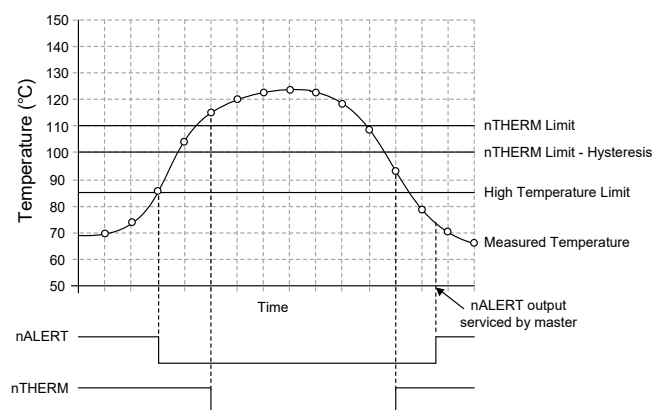
Figure 5. nALERT and nTHERM Interrupt Operation
