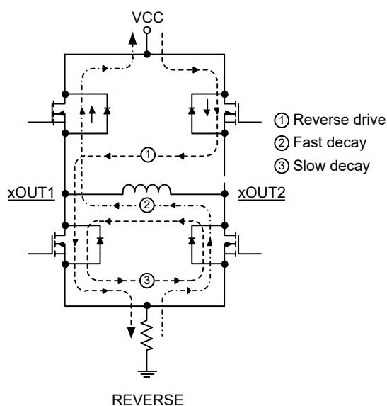
Figure 3. Decay Modes
