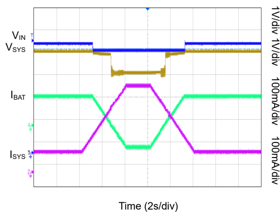
Input Voltage Regulation-Based PPM
