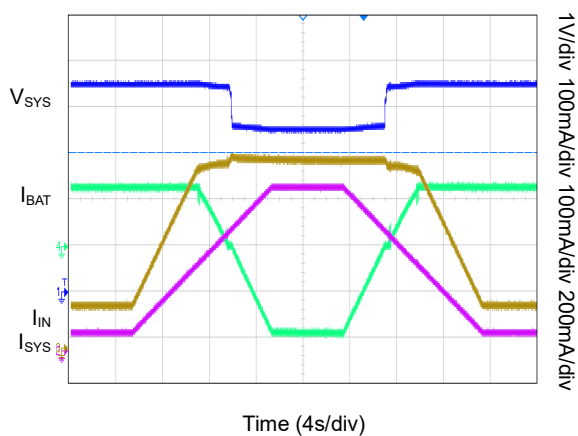
Input Current Limit-Based PPM
