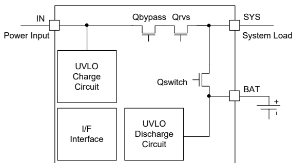
Figure 3. Power Path Management Structure
