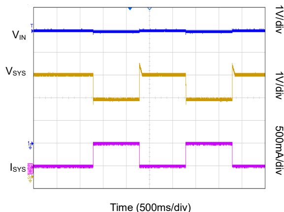
SYS Load Transient
