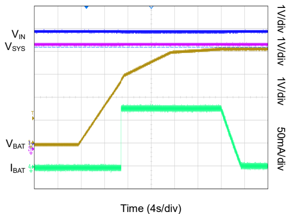
Battery Charge Curve
