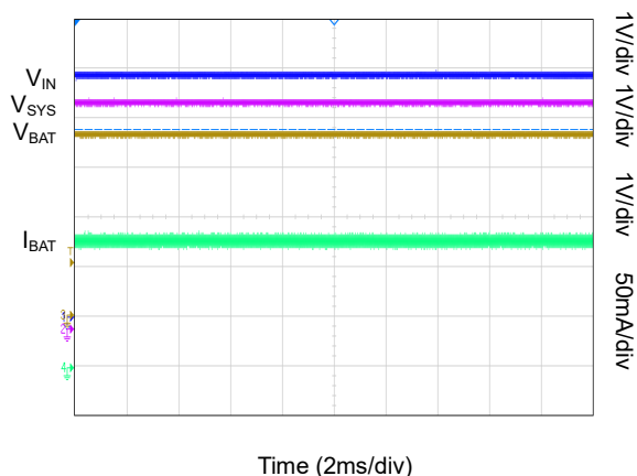
CC Charge Steady State
