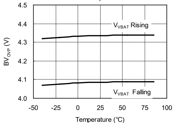
Battery Over-Voltage Protection Threshold vs. Temperature
