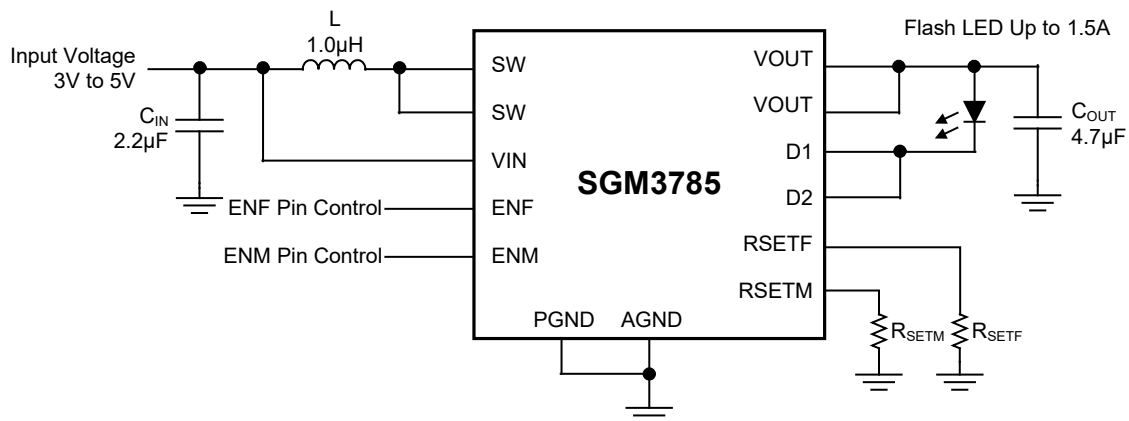
Figure 1. Optional Single LED Configuration
