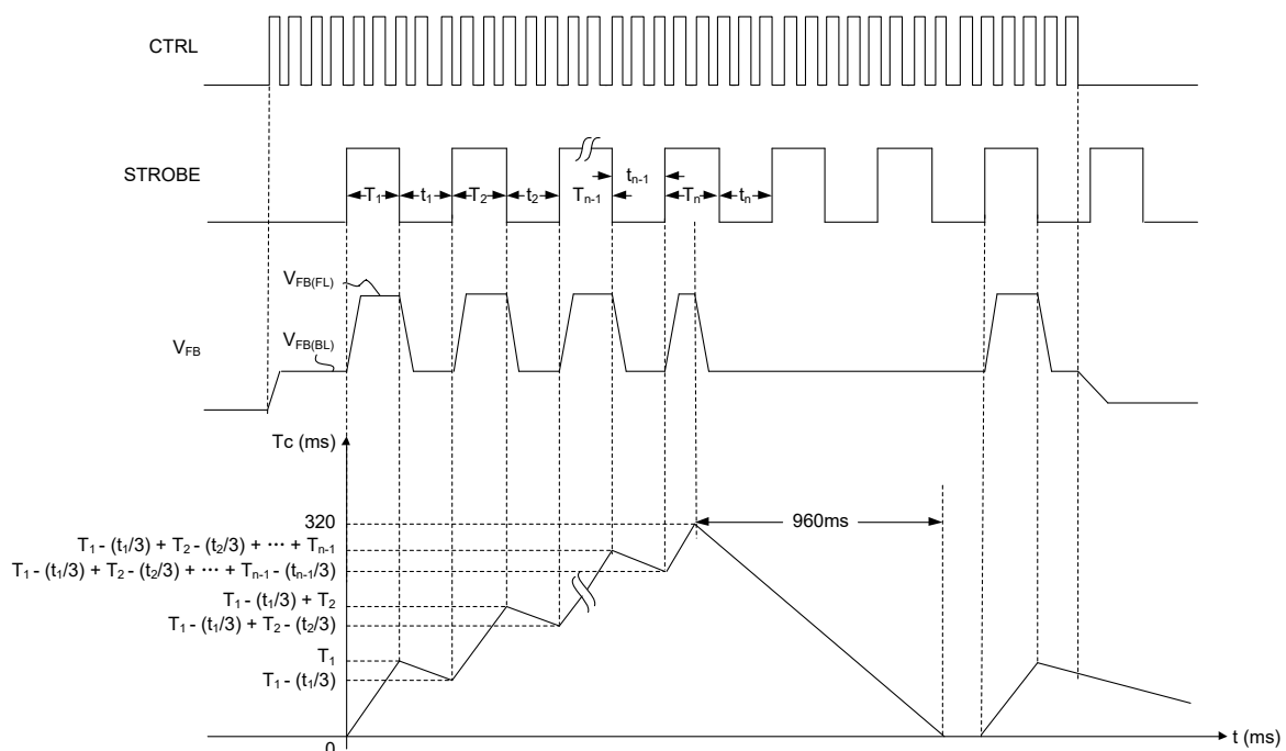
Figure 5. Timing Diagram
