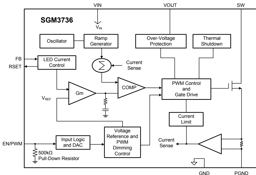
Figure 2. SGM3736 Block Diagram
