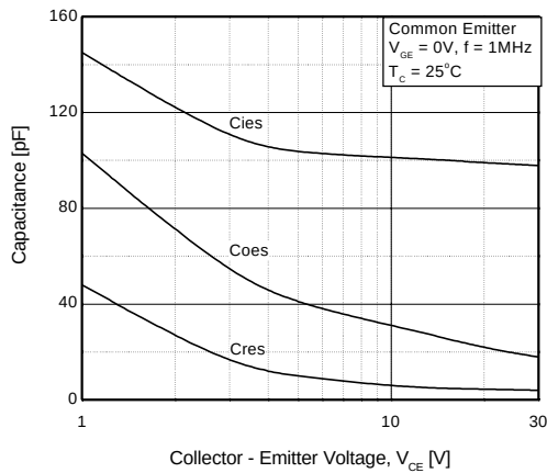
Fig 7. Capacitance Characteristics
