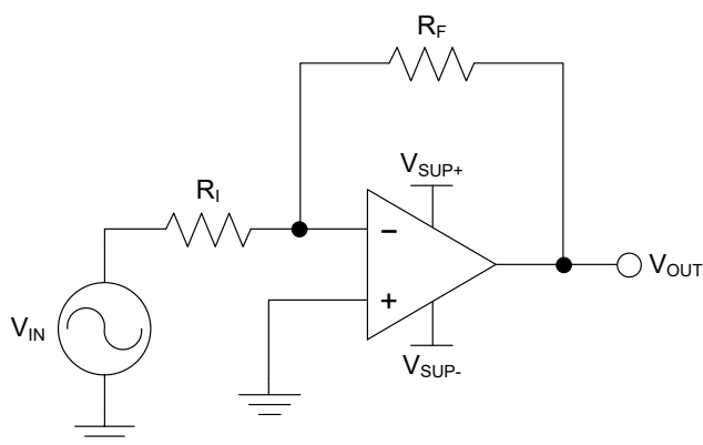
Figure 1. Application Schematic
