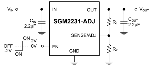
Figure 3. Adjustable Output Voltage Application
