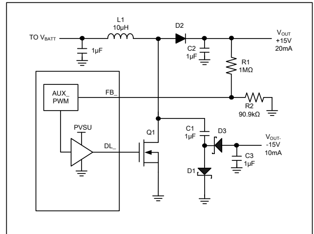
Figure 11. \pm 15V Output Using an AUX-Driven Boost with Charge-Pump Inversion
