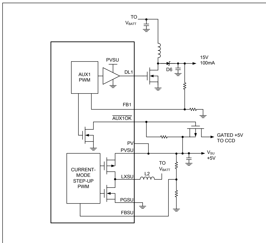
Figure 16. \overline{\text{AUX10K}} Drives an External PFET that Gates 5V Supply to the CCD after the +15V CCD Bias Supply Is Up
