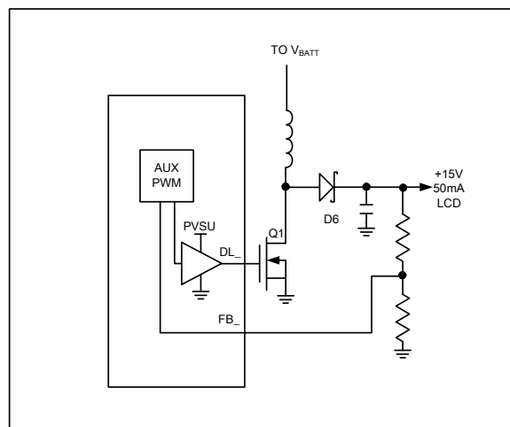
Figure 8. Boost DC/DC
