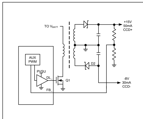
Figure 9. +15V and -8V CCD Bias with Transformer
