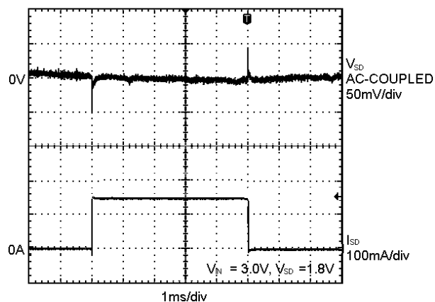
Step-Down Transient Response
