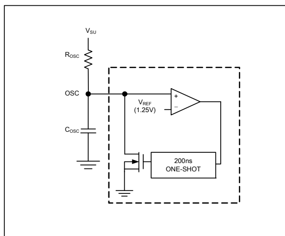
Figure 6. Oscillator Function Diagram
