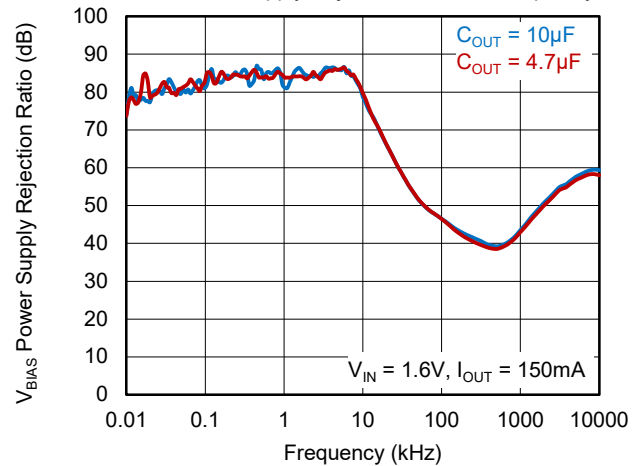
V_{BIAS} Power Supply Rejection Ratio vs. Frequency
