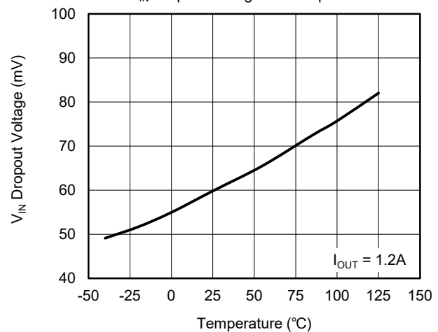
V_{IN} Dropout Voltage vs. Temperature
