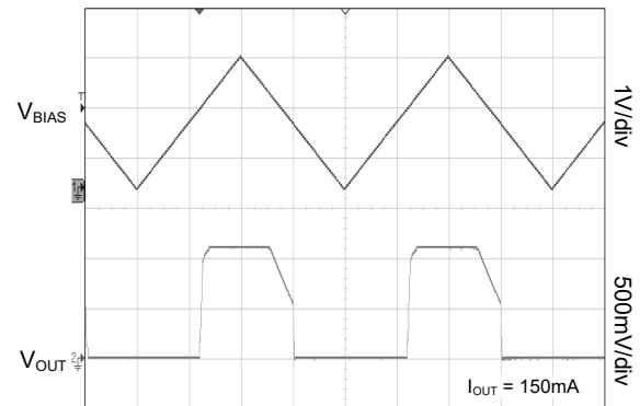
V_{BIAS} Power Ramp-Up/Ramp-Down Output Waveform
