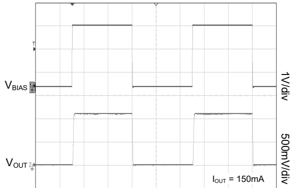
V_{BIAS} Power-Up/Power-Down Output Waveform
