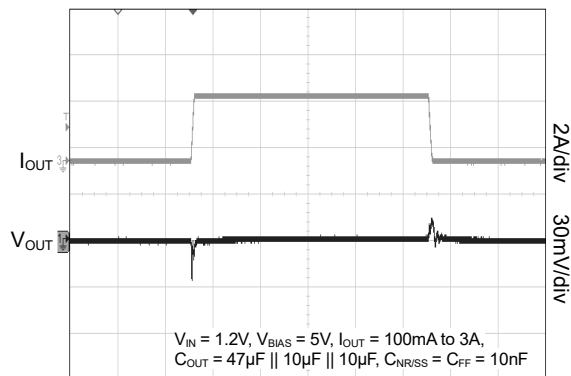
Load Transient Response with BIAS
