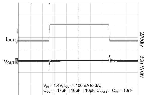
Load Transient Response without BIAS
