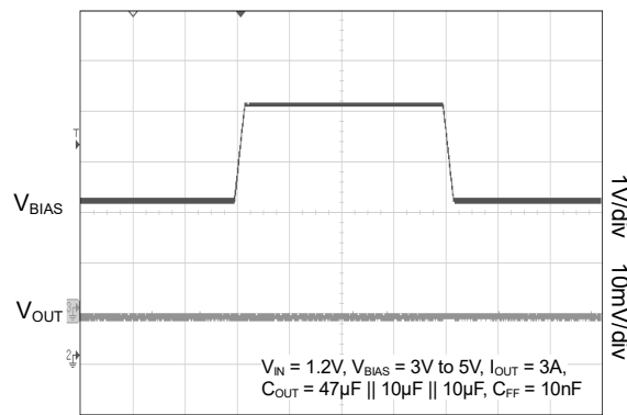
V_{BIAS} Line Transient Response
