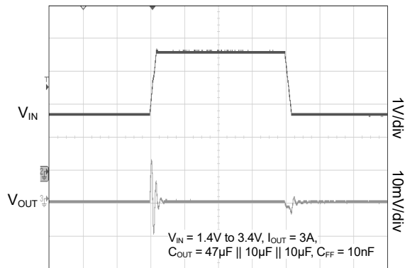
V_{IN} Line Transient Response without BIAS
