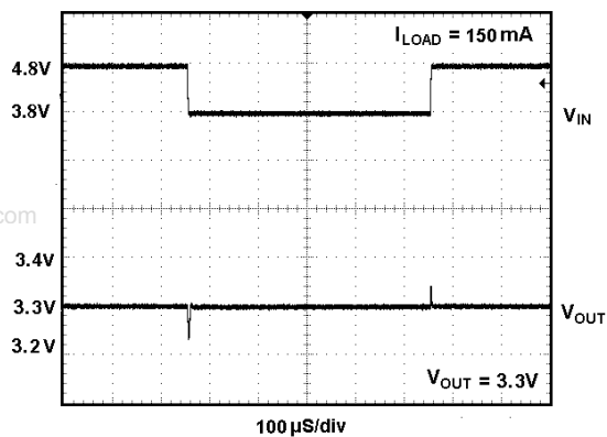
line-Transient Response
