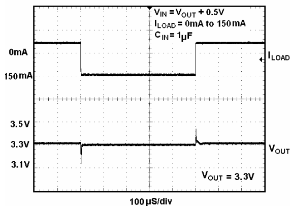
load-Transient Response
