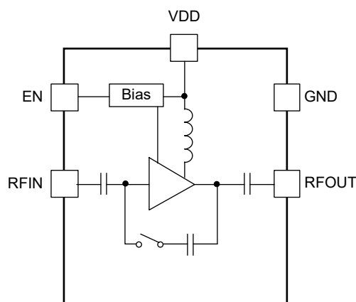
Figure 1. SGM13005L4 Block Diagram
